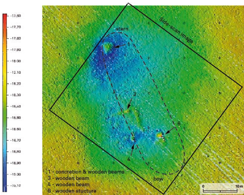
FIG. 8 Multibeam image obtained in 2009 from the 't Vliegent Hart wreck site (courtesy by MDK - Afdeling Kust - Vlaamse Hydrografie). Depth in m MLLWS (Mean Lowest Low Water level at Spring tide). The dotted line marks the (supposed) outline of the ship based on 1993 data (see fig. 6). Only few protruding wreck fragments are observed. Elongated features are most likely due to wooden beams or cannons. The stern remains stand out clearly. Numbered arrows refer to some of the wreck remnants observed in 2010 (see also fig. 9).
