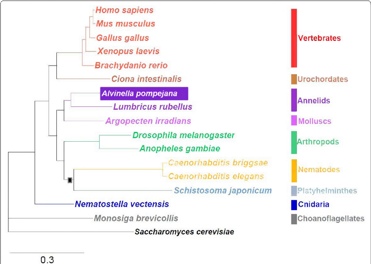
Figure 3 Bayesian phylogeny of Metazoa. The analysis was performed on a concatenation of 76 ribosomal protein family alignments, with Saccharomyces cerevisiae as the outgroup. The scale bar indicates the expected number of amino acid substitutions per aligned position. All nodes were resolved in 100% of the sampled topologies from the Bayesian analysis, except the node indicated by a square (support value of 96%).
