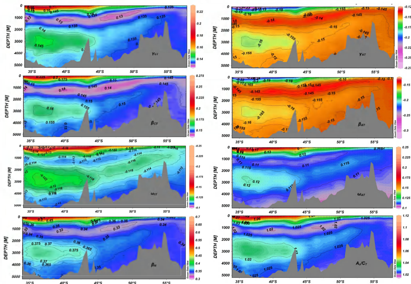
Fig. 5. The vertical distribution of fractional changes in [\text{CO}_2] ( \gamma_i ), [\text{H}^+] ( \beta_i ) and \Omega ( \omega_i ) ( \text{mmol kg}^{-1} ) over the changes in C_T and A_T and acid-base buffer capacity, \beta_H , ( \text{mmol kg}^{-1} ) for the whole of the BONUS GoodHope section, together with the ratio of carbonate alkalinity to inorganic carbon A_C/C_T .
