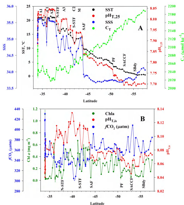
Fig. 2. (A) The sea surface temperature (SST), salinity (SSS), total dissolved inorganic carbon ( C_T , \mu\text{mol kg}^{-1} ) and pH in total scale at 25^\circ\text{C} ( \text{pH}_{\text{T},25} ) along the cruise track for samples analysed over the upper 10 m. The figure shows the position of the major frontal zones during the BONUS GoodHope cruise. (B) Surface ocean Chlorophyll a , partial pressure of \text{CO}_2 in seawater expressed as fugacity, f\text{CO}_{2,\text{sw}} ( \mu\text{atm} ) and pH in total scale at in situ conditions, \text{pH}_{\text{T},\text{IS}} .
