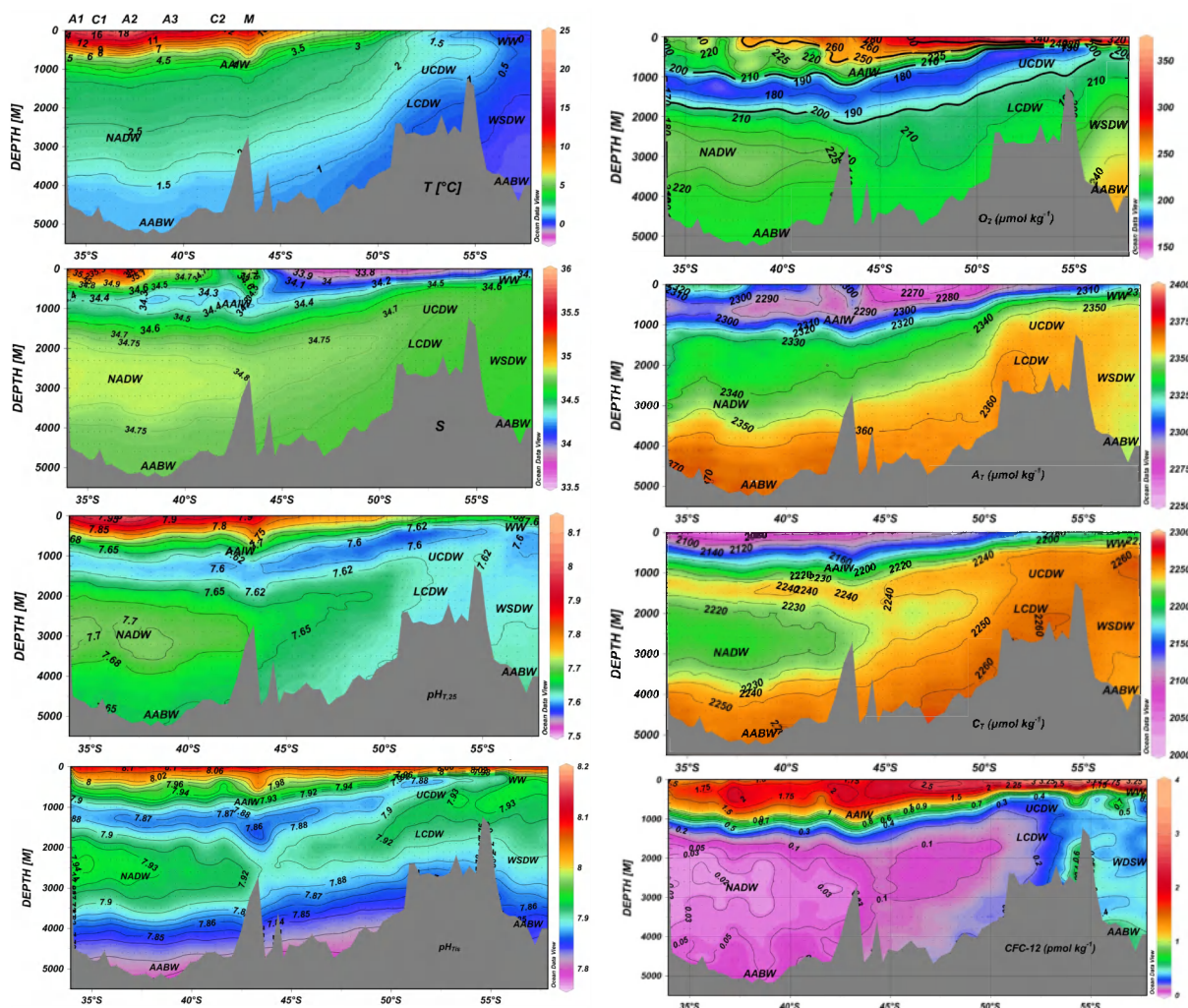
Fig. 3. The vertical distribution of temperature ( T , ^{\circ}\text{C} ), salinity ( S ), pH in total scale at 25^{\circ}\text{C} ( \text{pH}_{T,25} ), pH in total scale at in situ conditions ( \text{pH}_{TIS} ), dissolved oxygen ( \text{O}_2 , \mu\text{mol kg}^{-1} ), total alkalinity ( A_T , \mu\text{mol kg}^{-1} ), total dissolved inorganic carbon ( C_T , \mu\text{mol kg}^{-1} ) and chlorofluorocarbon-12 ( \text{CFC-12} , \text{pmol kg}^{-1} ) along the southeast Atlantic sector of the Southern Ocean during February to March 2008. The dots indicate the locations of discrete samples.
