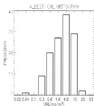
Chlorophyll-a values of algorithm selection dataset (A_best)
