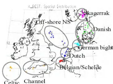
Locations of algorithm selection measurements (A_best dataset)
