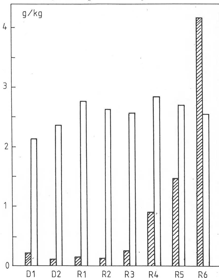
Figure 2 Total concentrations of iron (g/kg) in the <63 \mu m fraction (left columns) and the 63-500 \mu m fraction (right columns) of the eight stations
