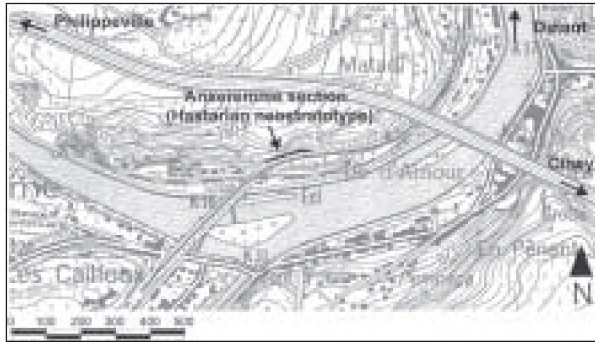
Figure 2. Detailed location of the neostratotype Anseremme railway bridge section.
