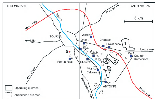
Figure 2. The Tournai area. Location of main quarries, operating and abandoned (from Delepine, 1911), opened in the “Calcaire de Tournai” and most important localities. 1. C.C.B. quarry at Gaurain-Ramecroix; 2. Milieu quarry (Obourg Granulats S.A.), at Gaurain-Ramecroix; 3. Lemay S.A. quarry at Vaulx; 4. Antoing S.A. quarry at Antoing. 5. Location of the Tournai drill hole.
