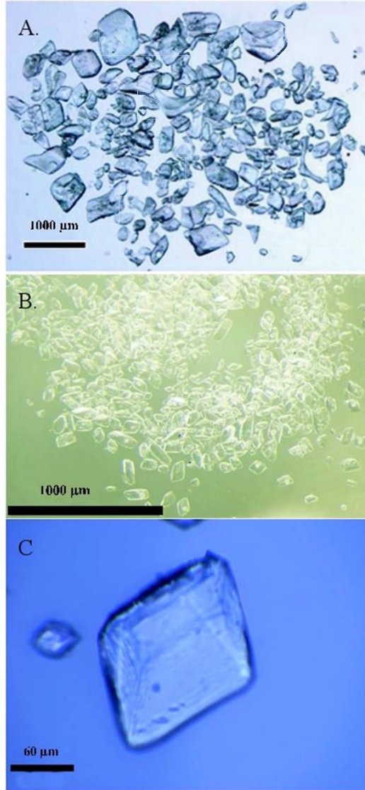
Figure II.2: Pictures of ikaite crystals. A. from Dieckmann et al. [2008], B. from our direct measurement under a binocular microscope, C. from a Raman
