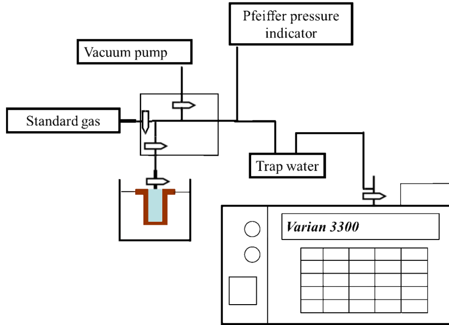
Figure IV.2: Sketch of the different components forming the extraction line, including the Varian 3300 ® gas chromatograph.
