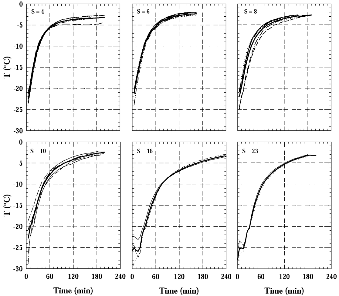
Figure IV.4: Evolution of ice temperature with time as a function of mean ice salinity for artificial ice samples immersed in a bath at -2^{\circ}\text{C} . The bold line in each graphic is the mean trend.
