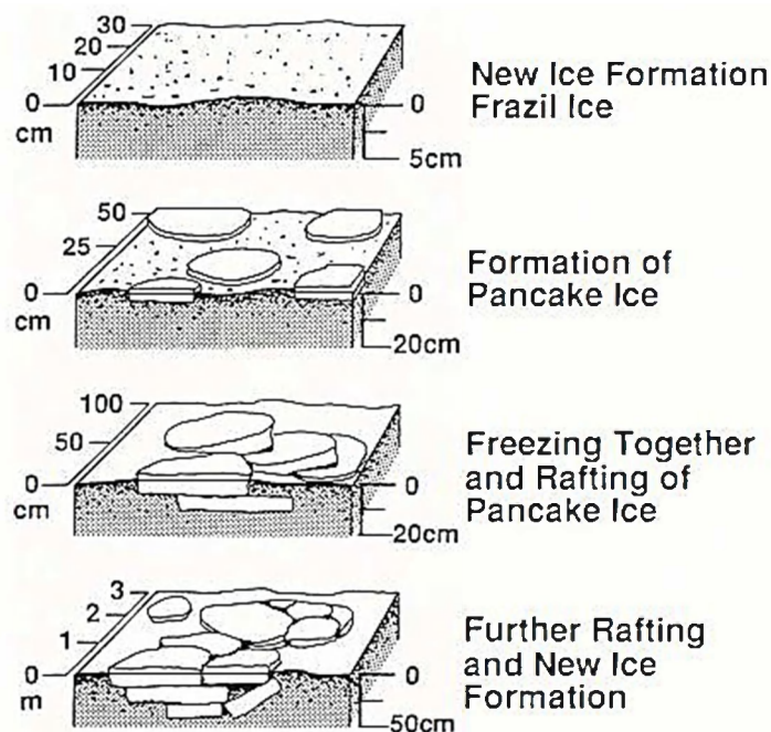
Figure I.3.5: Schematic representation of the “pancake cycle” [Lange et al. , 1989].
