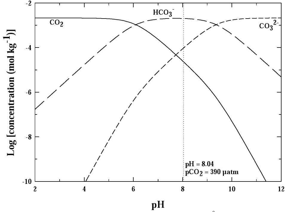
Figure I.2.1: Bjerrum plot showing the changes of CO 2 , HCO 3 - and CO 3 2- in typical conditions of arctic surface waters (S = 33, T = 2°C, P = 1 atm, DIC = 2139 μmol kg -1 ). The vertical dotted line corresponds to the equilibrium with the atmosphere.
