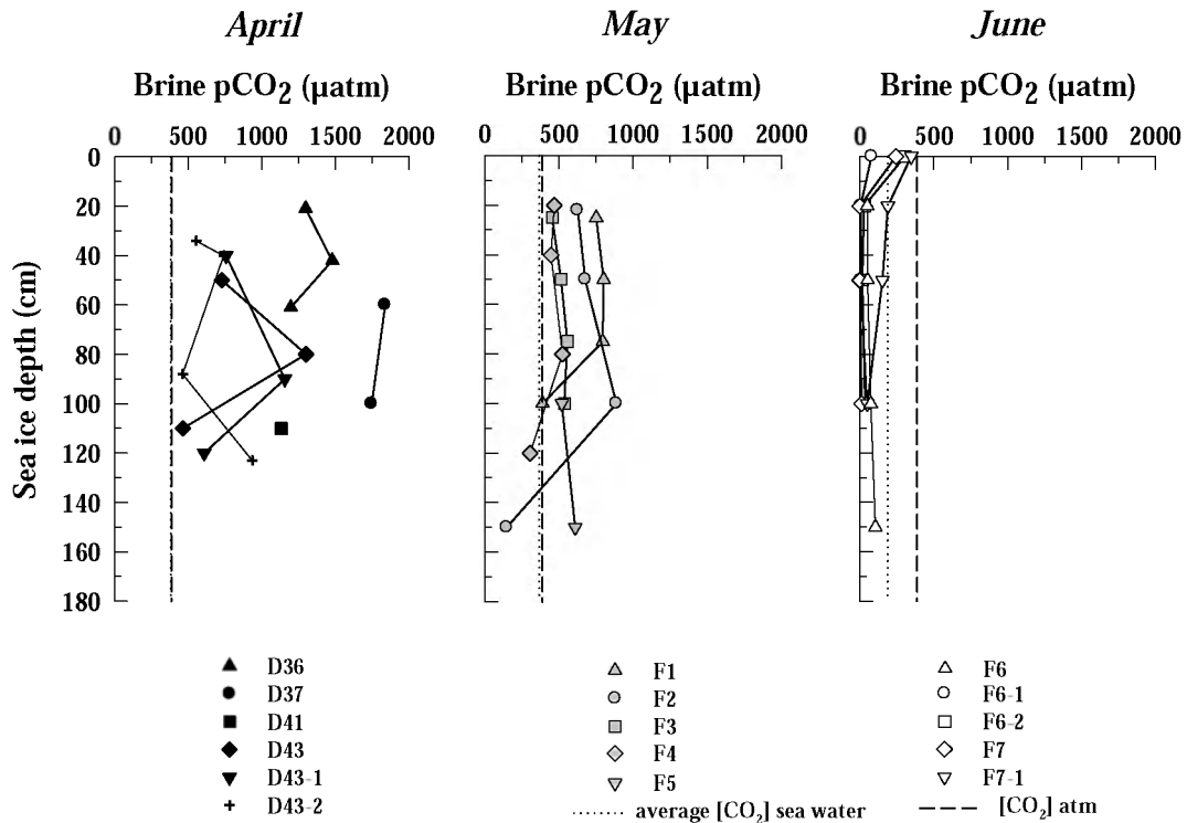
Figure III.5: Profiles of brine p\text{CO}_2 for the three groups of stations considered. The seawater p\text{CO}_2 (dotted line) is an average for the considered month.
