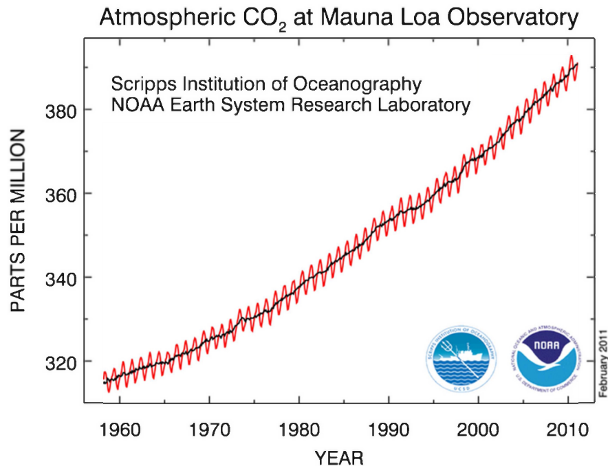
Figure I.2: Monthly mean atmospheric CO 2 concentration measured at Mauna Loa Observatory, Hawaii ( http://www.esrl.noaa.gov/gmd/ccgg/trends/ ).
