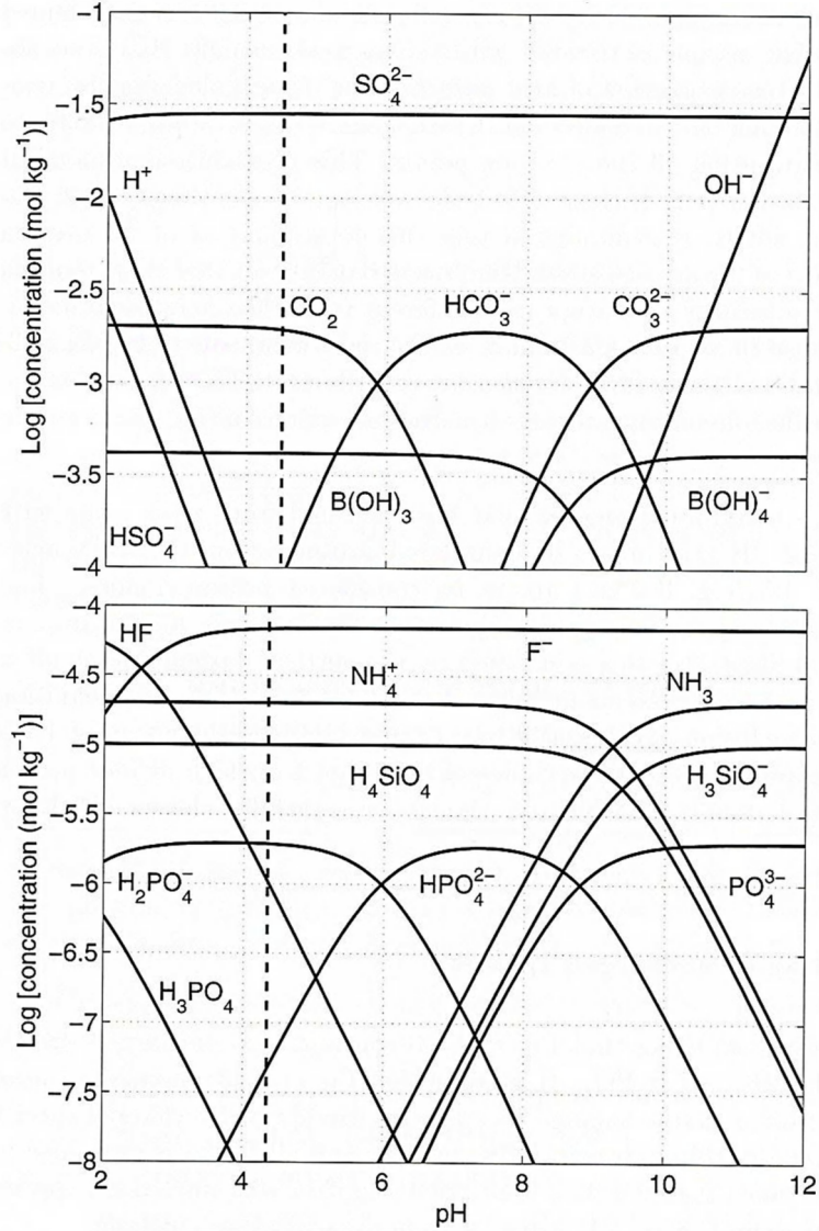
Figure I.2.2: Extended Bjerrum plot showing the acid-base systems relevant to TA in seawater. The vertical dashed line at pH = 4.5 indicates species to be considered as proton donors and acceptors [Zeebe R.E. and Wolf-Gladrow, 2001].
