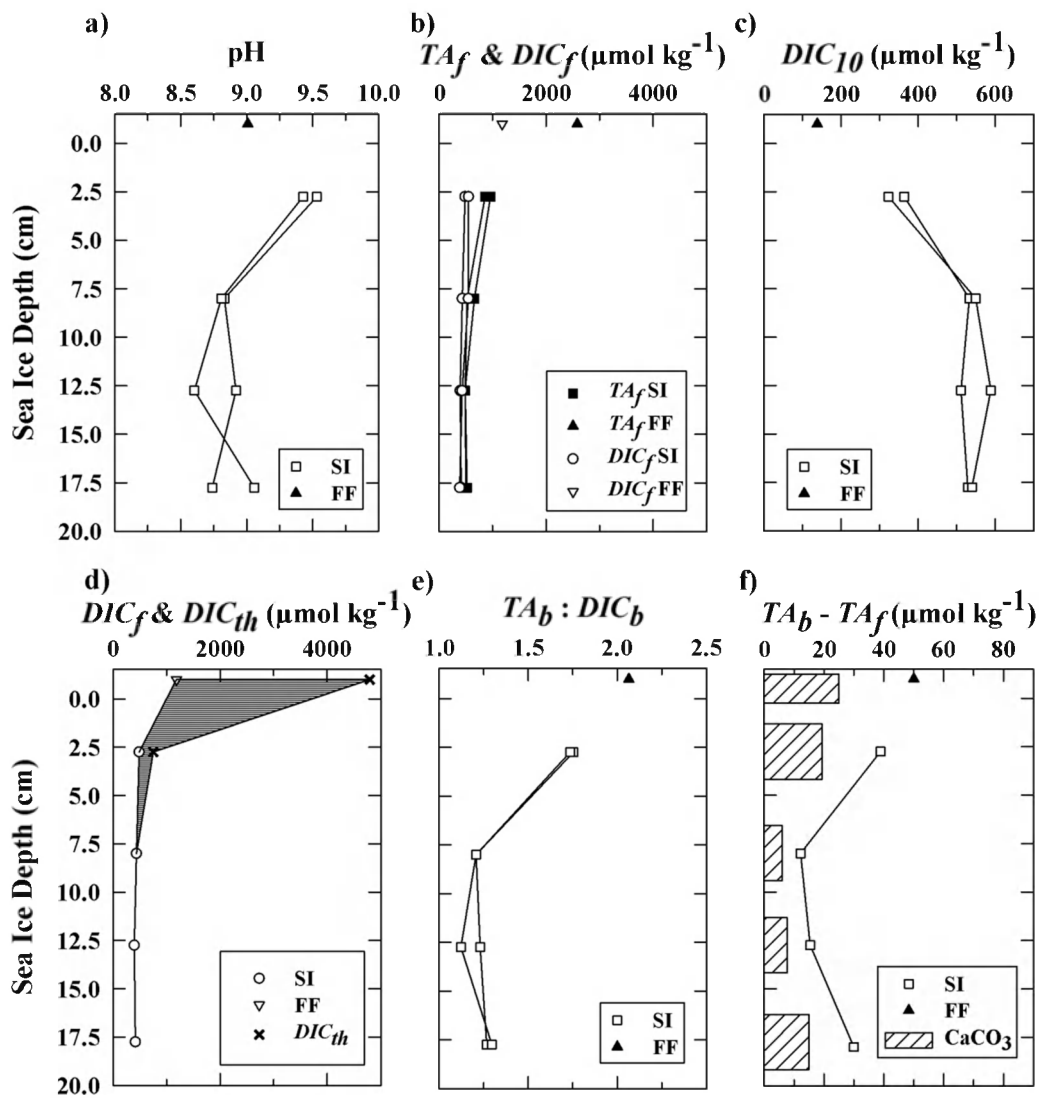
Figure II.5: Profiles of pH (a), TA_f and DIC_f (b), DIC_{10} (c), difference between the DIC_f and DIC_{th} (d), ratio between TA_b and DIC_b (e) and the difference between bulk and filtrated TA with the estimation of the precipitated amount of calcium carbonate (f).
