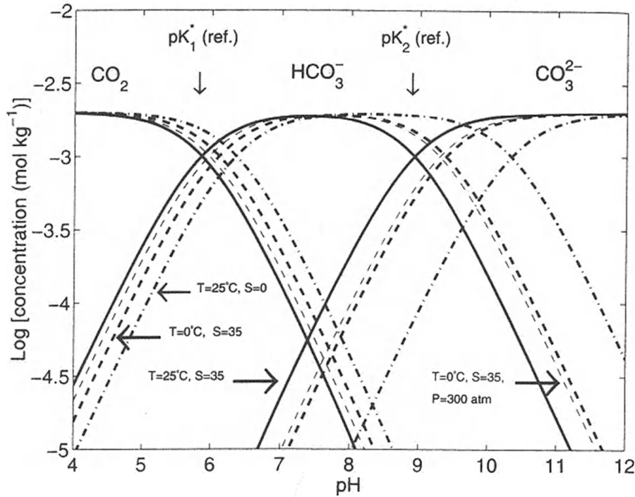
Figure I.2.3: Illustration of the effect of temperature, pressure and salinity on pK_1^* and pK_2^* . The reference case (solid line) is T = 25^\circ\text{C} , S = 35 , P = 1 \text{ atm} . \text{DIC} = 2 \text{ mmol kg}^{-1} in all cases.
