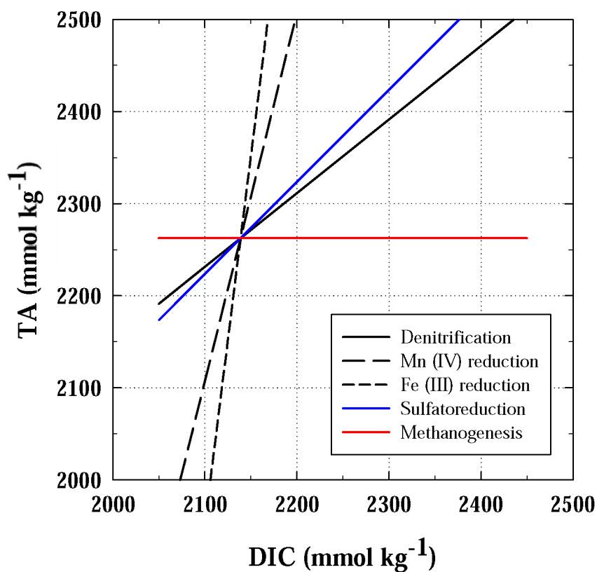
Figure I.2.5: Effects of different processes on DIC and TA (with the exception of precipitation of \text{CaCO}_3 , gas exchange and photosynthesis that are provided in Figure I.2.4). The initial conditions are typical conditions found in arctic surface waters ( S = 33 , T = 2^\circ\text{C} , P = 1 \text{ atm} ) in equilibrium with the atmosphere ( p\text{CO}_2 = 390 \mu\text{atm} , \text{pH} = 8.04 ) with a DIC of 2139 \mu\text{mol kg}^{-1} and a TA of 2262.5 \mu\text{mol kg}^{-1} .
