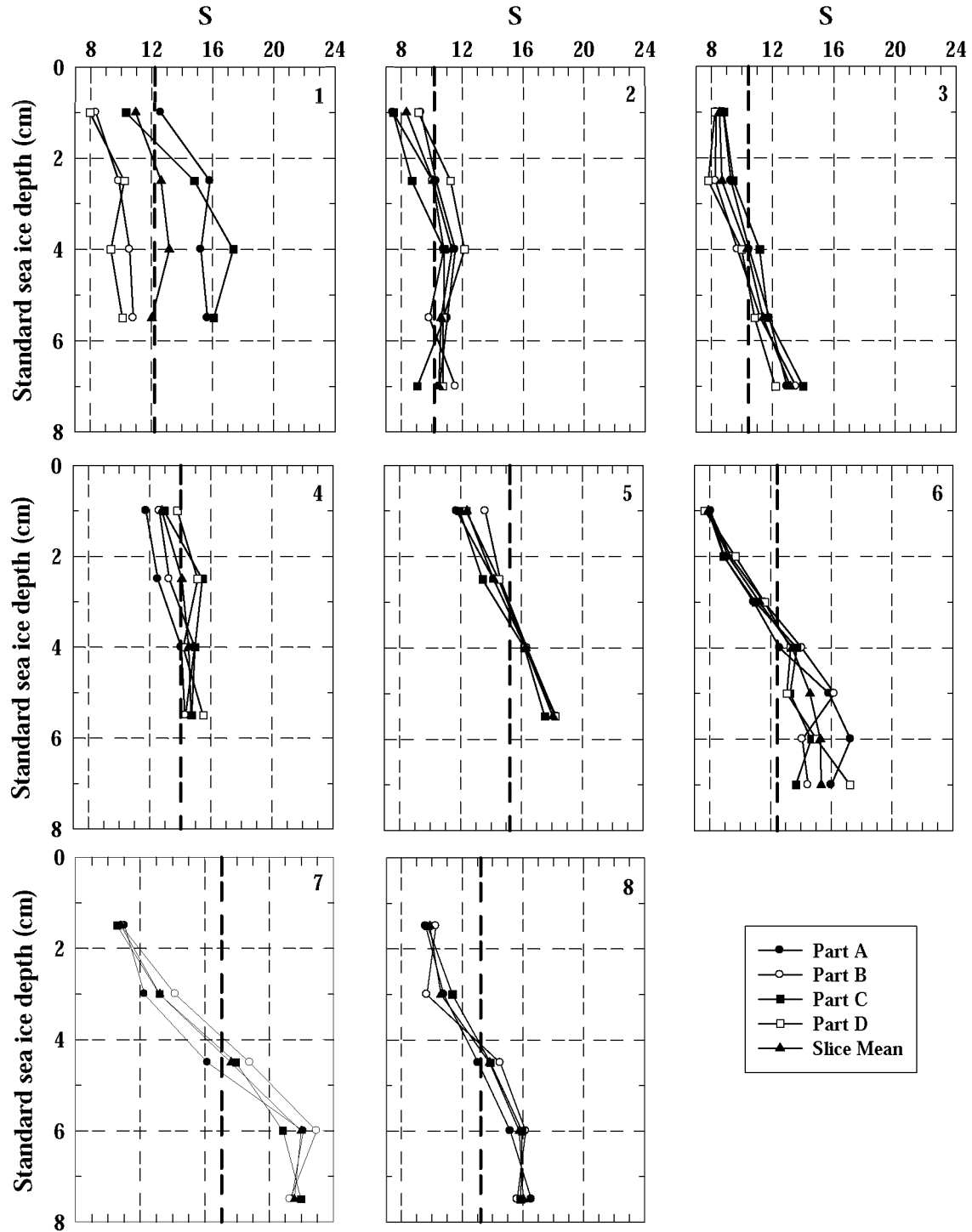
Figure IV.3: Salinity profile in 8 artificial standard sea ice blocks. The bold dashed line represents the mean salinity of the bulk block while the black triangle is the mean salinity of each slice of the block.
