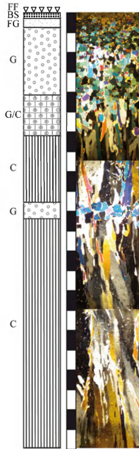
Figure II.4: Textural features of the young sea ice include: frost flowers (FF), brine skim (BS), fine-grained granular ice (FG), orbicular granular ice (G), intermediate granular/columnar ice (G/C) and columnar ice (C).
