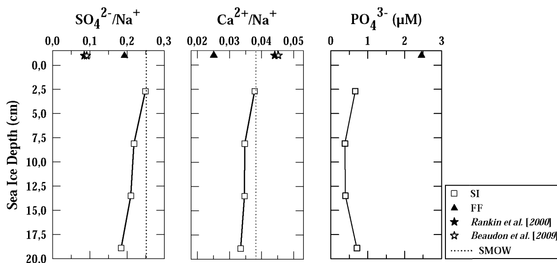
Figure II.6: Ratios of ions in frost flowers (FF) and sea ice (SI) in our study as compared with the frost flowers data from Rankin et al. [2000] and Beaudon et al. [2009] and to standard mean ocean water (SMOW). Concentration of phosphates in frost flowers (FF) and sea ice (SI)
