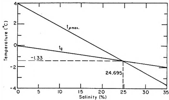
Figure I.3.3: Temperature of the density maximum T_{\rho_{max}} and of the freezing point T_g for seawater of different salinities [Weeks and Ackley, 1982].
