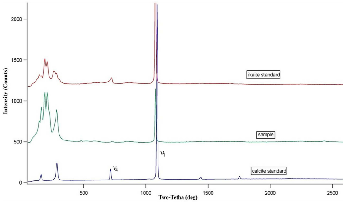
Figure II.8: Raman spectra of calcite standard (blue), ikaite (red) and sample (green).
