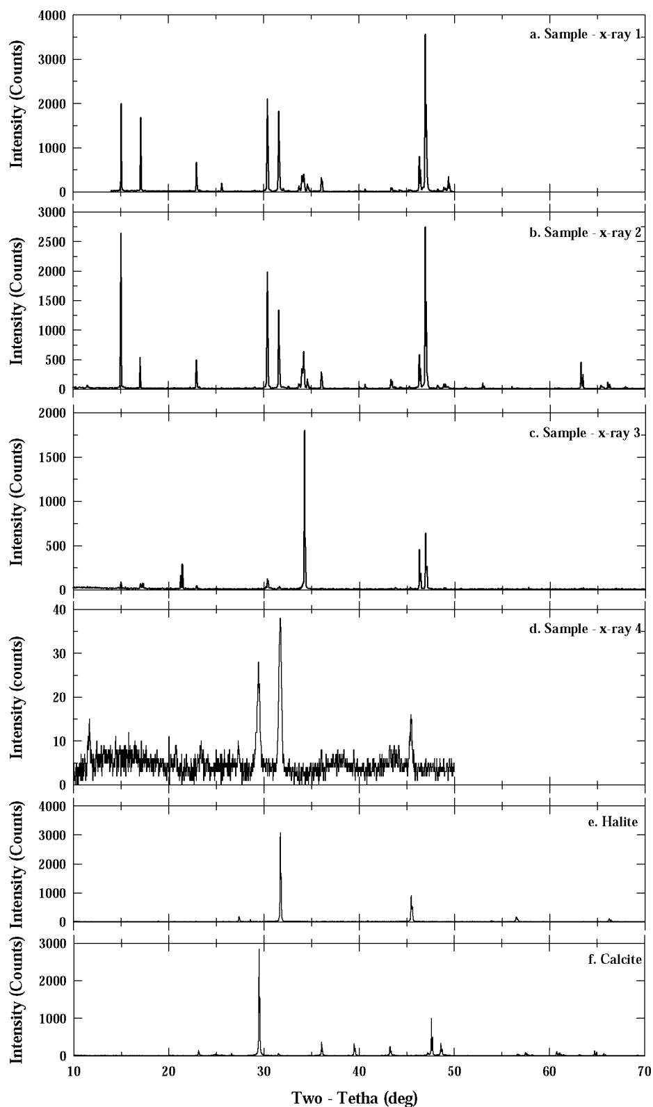
Figure II.7: Successive X-ray diffraction patterns of crystals stored on Millipore filters at -25^{\circ}\text{C} ( a , b , c ), X-ray diffraction from same sample after 1 day at room temperature ( d ). Line patterns for Halite ( e ) and Calcite ( f ) from the RRUFF data base. The data base numbers are R070534 for Halite and R040070 for Calcite.
