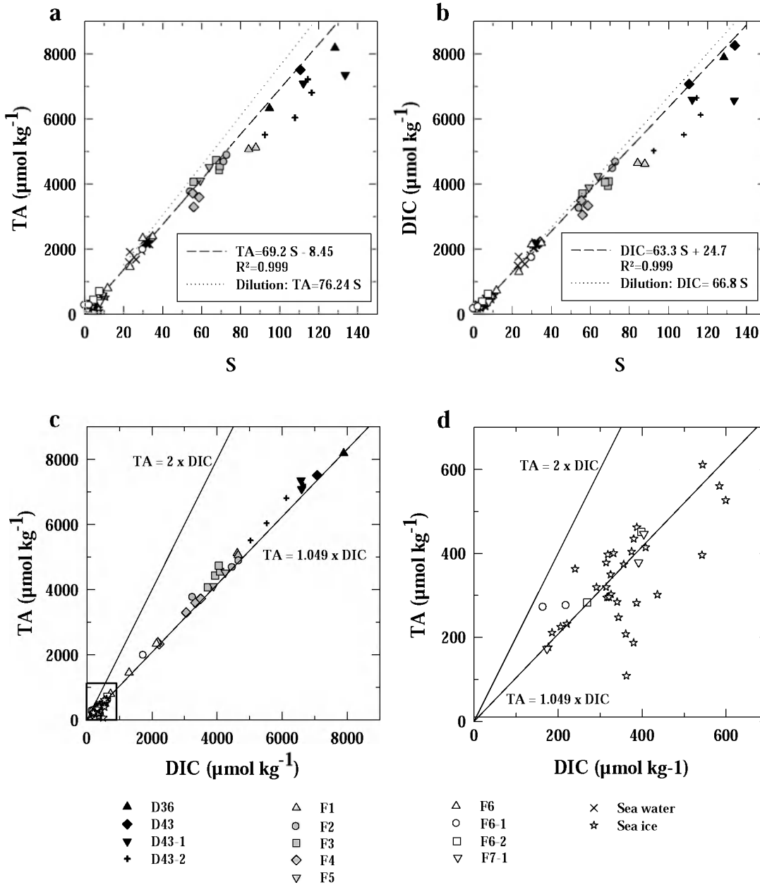
Figure III.6: Evolution of TA (a) and DIC (b) as a function of the salinity of the brine for all the CFL stations considered. The dotted line represents expected values based on dilution effect during melting while the dashed line represents the highly correlated relation between TA (or DIC) with salinity. The relation between TA and DIC for both the brine and the sea ice (stars) is shown in c. Figure d is a “zoom in” of the square from figure c in order to better document the relation in bulk sea ice. The two lines show the ratio TA: DIC of 2 (representing the stoichiometry of the precipitation/dissolution equilibrium in equation 1) and the TA: DIC ratio of 1.049, typical of the underlying seawater.
