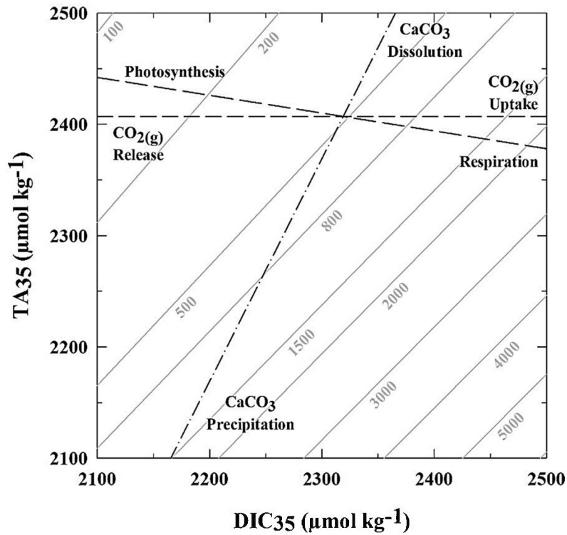
Figure III.1: Effect of various processes on \text{DIC}_{35} and \text{TA}_{35} , TA and DIC values normalized to a salinity of 35, (dashed lines). Gray lines indicate levels of constant p\text{CO}_2 (in \mu\text{atm} ).
