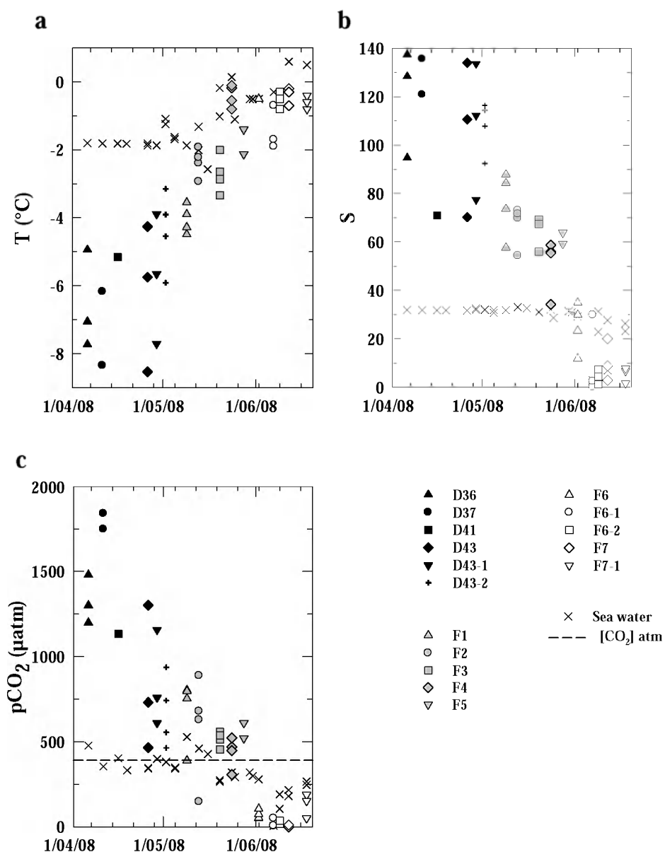
Figure III.4: Temporal evolution of brine and seawater temperature (a), salinity (b) and p\text{CO}_2 (c) for the CFL stations considered.
