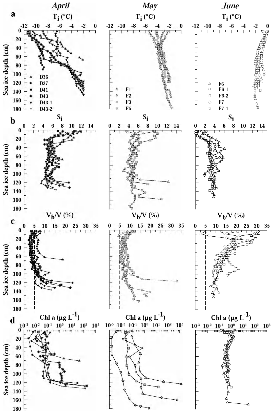
Figure III.3: Sea ice conditions for the CFL stations considered, adapted from the companion paper Carnat et al. [this issue], including (a) temperature profile, T_i , (b) salinity profile, S_i , (c) relative brine volume, V_b/V and (d) Chl a concentration.
