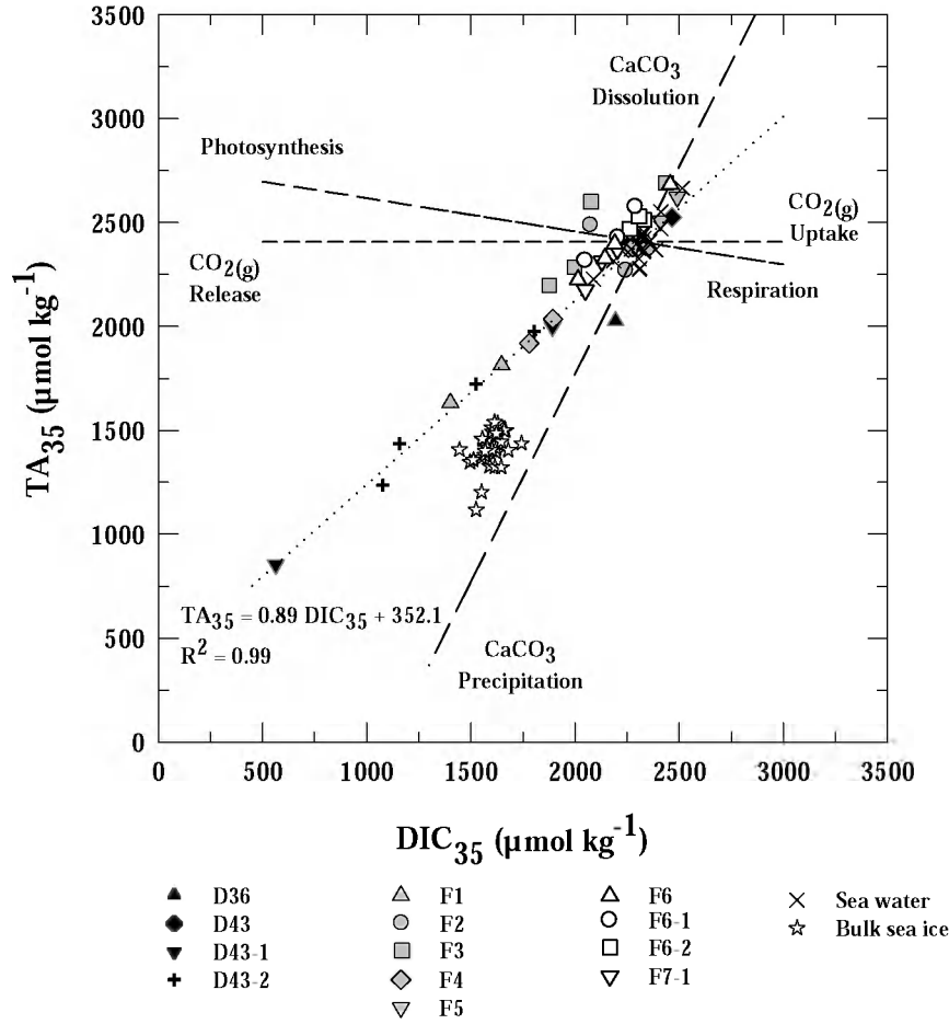
Figure III.8: DIC 35 : TA 35 (values normalized to a salinity of 35) relationship in brine, seawater samples and ice samples. The different dotted lines represent the theoretical evolution of DIC 35 : TA 35 following a precipitation/ dissolution of calcium carbonate, a release or uptake of CO 2(g) and impacts of biology.
