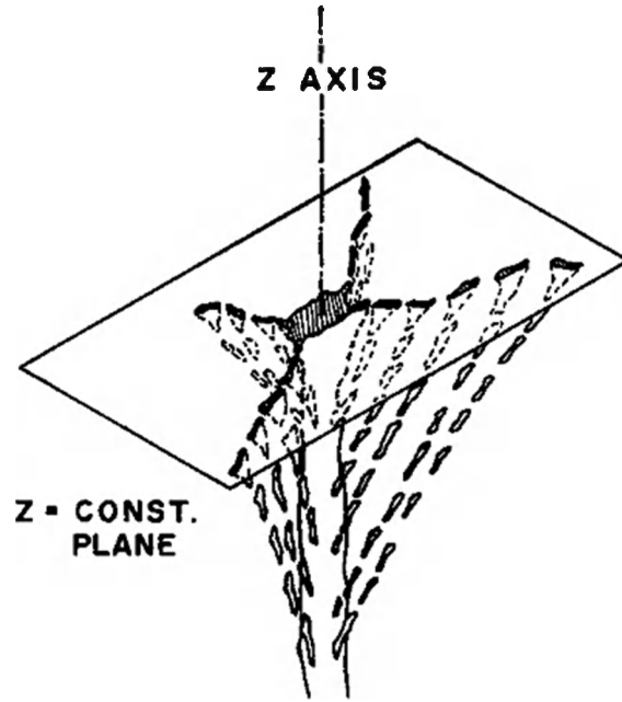
Figure I.3.11: Schematic drawing of a brine drainage channel and its feeder arms. Feeder arms are formed of inclusions inclined to the vertical at angles in the range of 40°-54° [Lake and Lewis, 1970].
