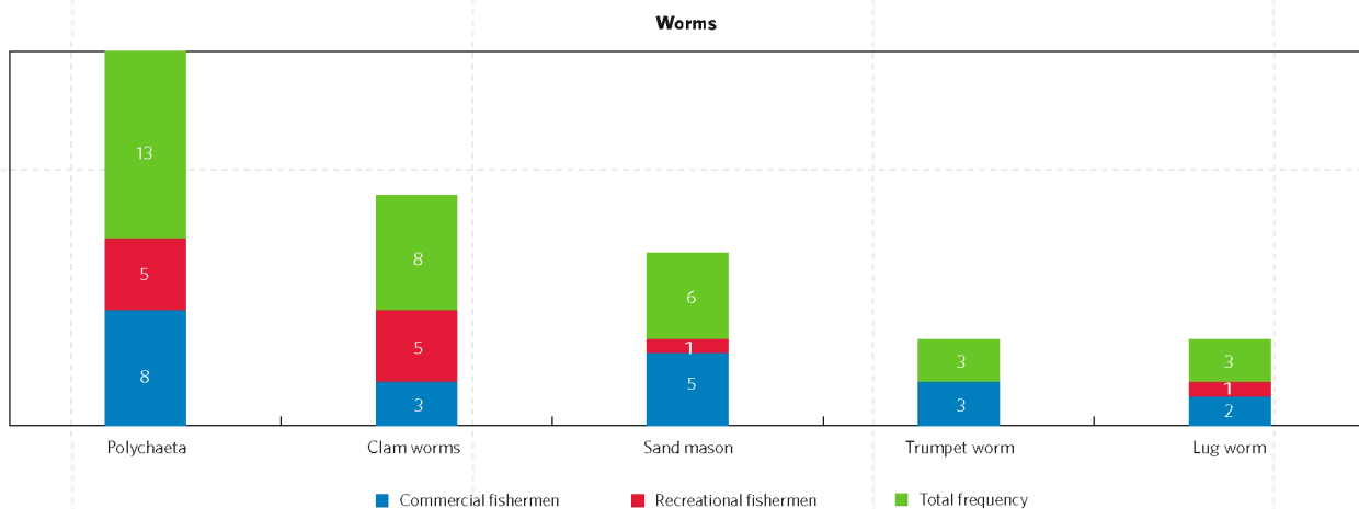
Figure 22: Worm subspecies
