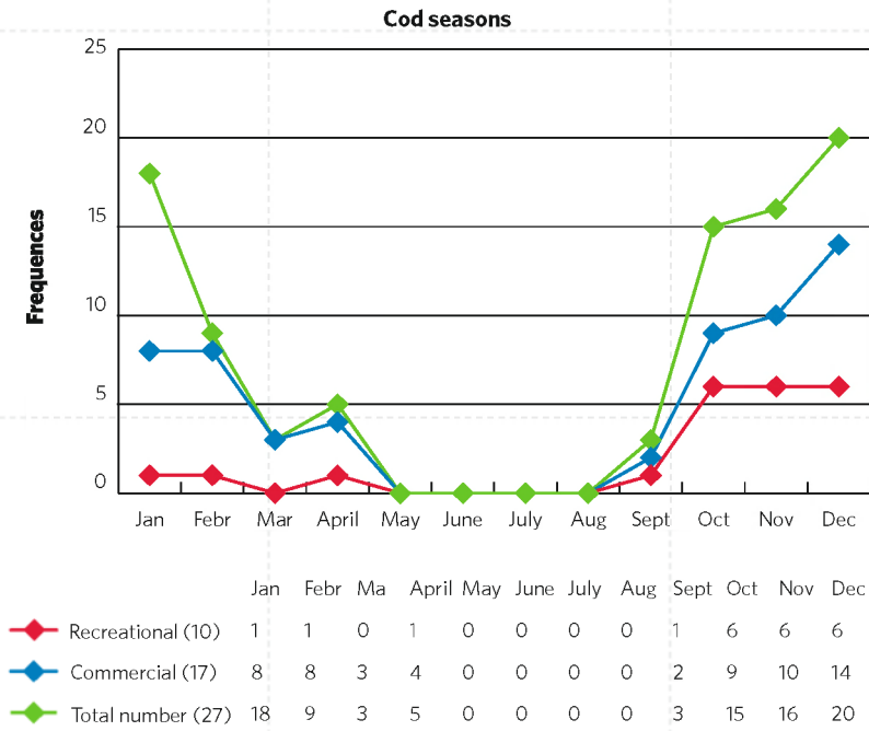
Figure 18: Cod seasons
