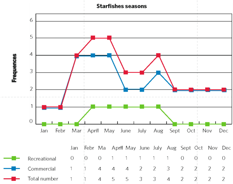
Figure 31: Starfishes seasons
