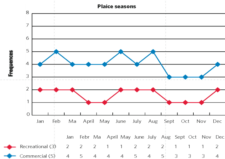
Figure 26: Plaice seasons
