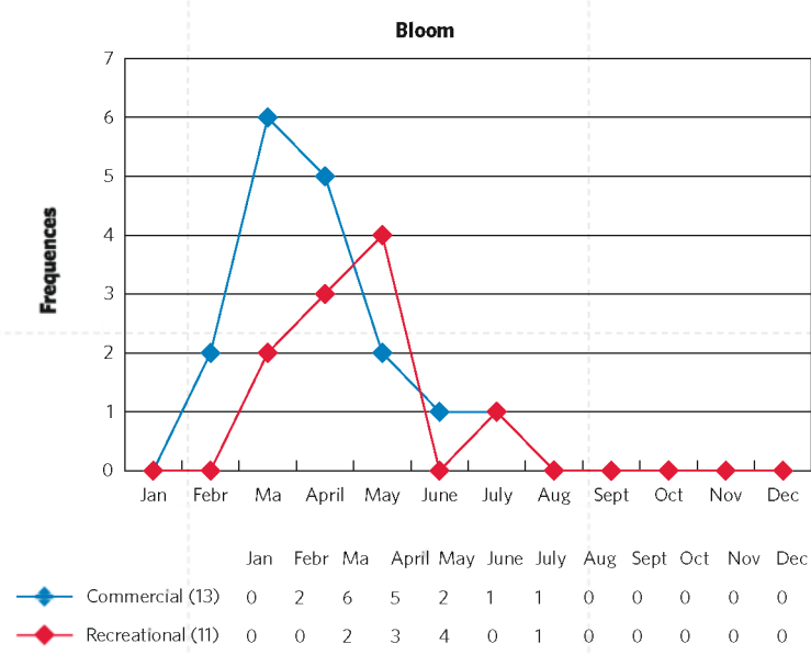
Figure 17: Bloom season
