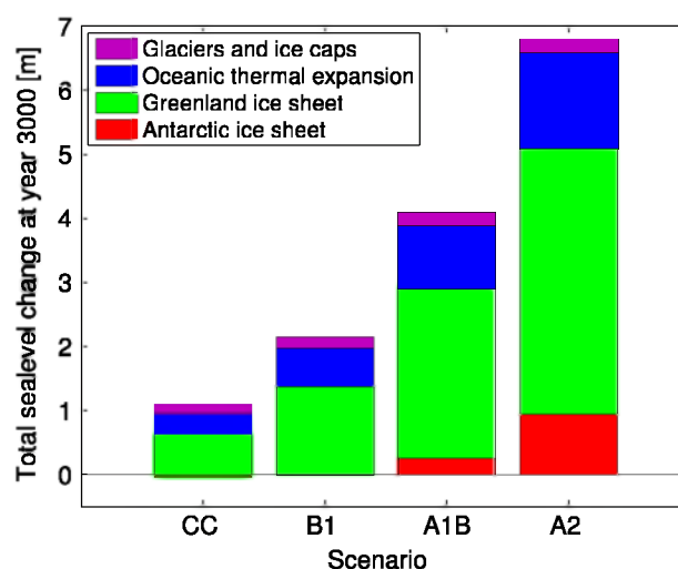
Figure 5. Committed total sea-level contributions from the different components considered in this study by the year 3000 relative to 2000 AD for prolonged SRES scenarios B1, A1B and A2 and constant year 2000 composition CC. The total bar is shifted downwards to represent the negative contribution from the Antarctic ice sheet (B1, CC) and display the total sea-level rise on the left axis correctly.
