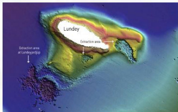
Figure 5. Seabed topography in Kollafjörður generated from bathymetric survey.
