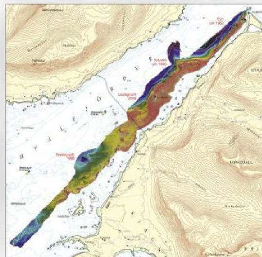
Hvalfjörður seafloor survey by Icelandic Coast Guard – Hydrographic Department 2010. Dredging areas are marked by a dotted line in red, year indicates beginning of extraction.
