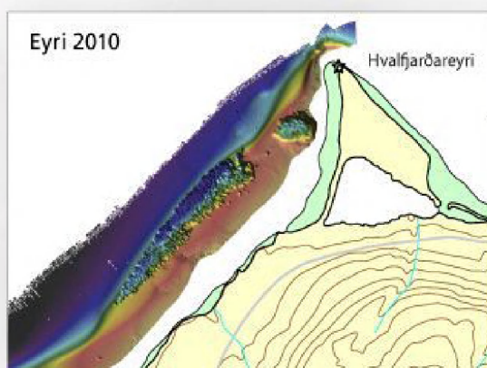
Marine aggregate area for Eyri in Hvalfjörður as surveyed in 2010. Extraction of gravel and sand from the seabed in Iceland started in 1963 in the west side of Hvalfjörður, first in the round pit shown on the chart and then moved to the dredging area further offshore.
