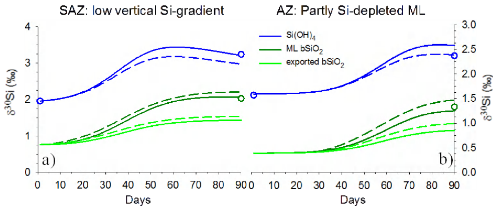
Fig. 8. Model outputs for the SAZ (a) and AZ (b). Simulated \delta^{30}\text{Si} values for \text{Si(OH)}_4 , ML \text{bSiO}_2 , exported \text{bSiO}_2 without (full lines) and with (dashed lines) \text{bSiO}_2 dissolution isotopic fractionation ( ^{30}\epsilon = -0.55\text{‰} ). The initial and final estimations are indicated by empty dots with the corresponding colors (Table 2). Respectively, for the SAZ and AZ: V_{\text{max}} = 0.40 and 0.31\text{ d}^{-1} , K_{\text{Si}} = 2 and 10\text{ }\mu\text{mol l}^{-1} , k_{\text{export}} = 0.11 and 0.13\text{ d}^{-1} , \text{Si(OH)}_4 supply = 77 and 1170\text{ mmol m}^{-2} , and net \text{bSiO}_2 production = 275 and 4149\text{ mmol m}^{-2} .
