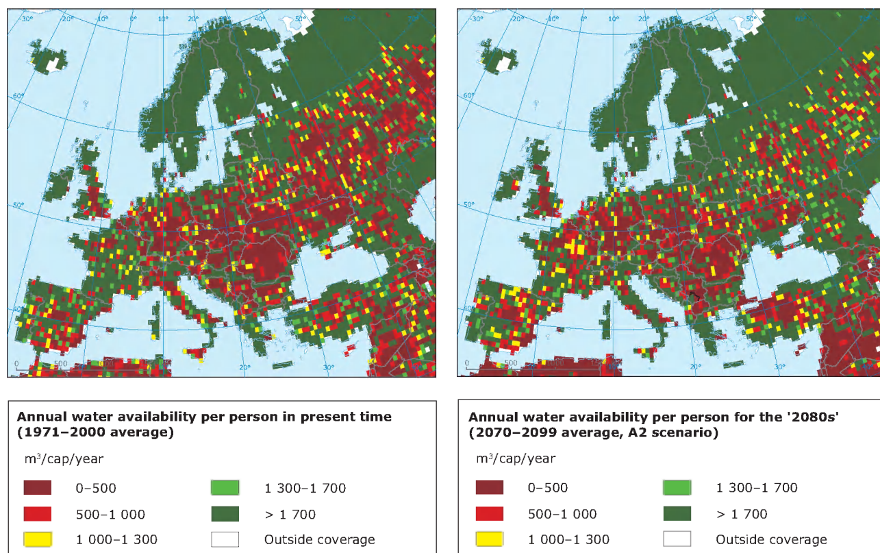
Map 2.5 Annual water availability per person (Falkenmark indicator)
