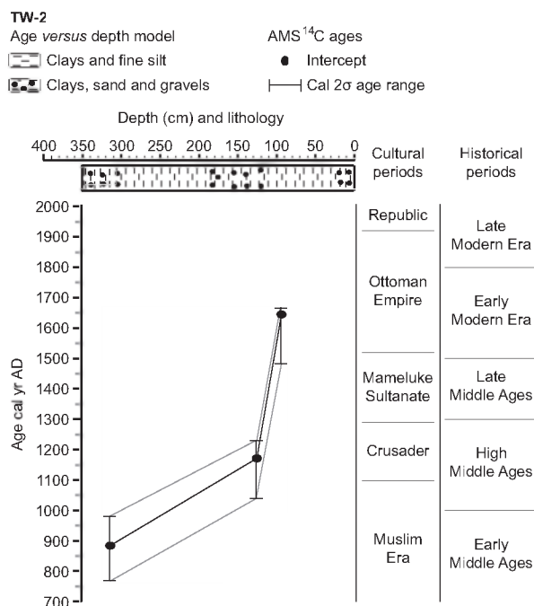
Figure 2. AMS ^{14}\text{C} calibrated ages and suggested age–depth curves
