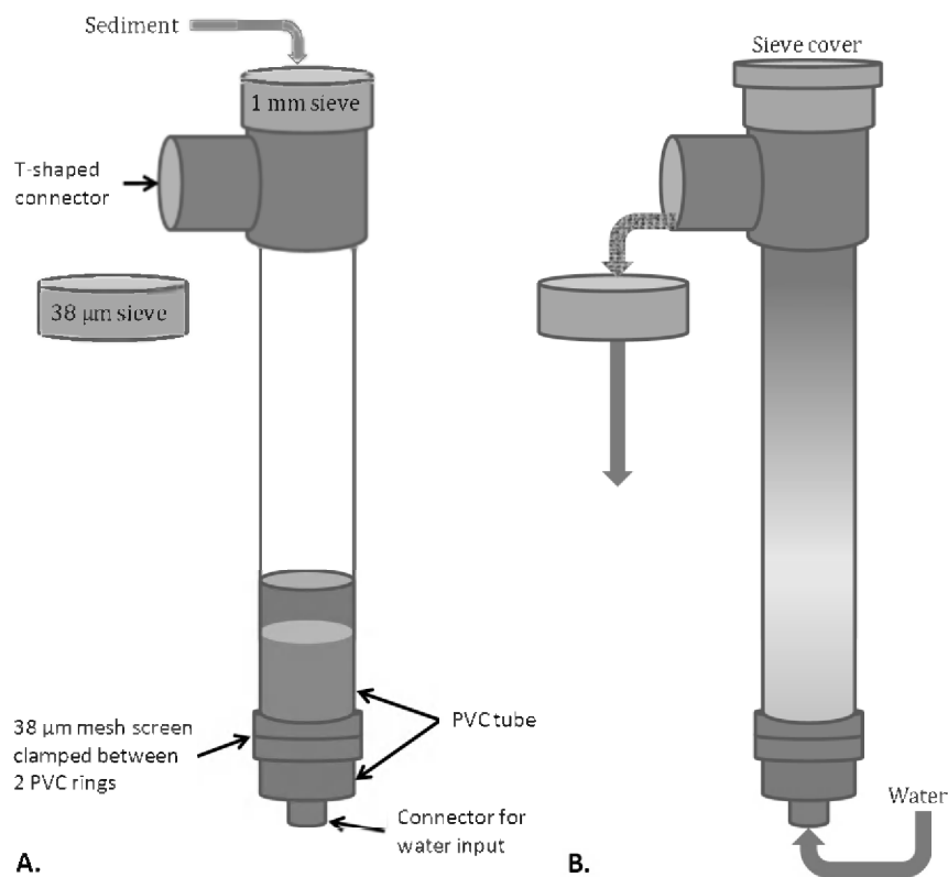
Figure 6: Schematic representation of the elutriation device used to extract microplastics from sediments
