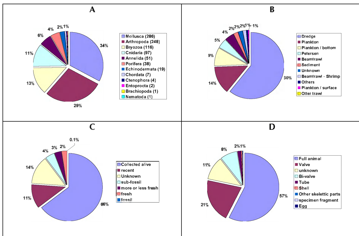
Figure 2.2-3. Overview figures from the bulk of the historic data on invertebrates (G. Gilson) (relative proportions of ‘records’ from the bulk data-set). A. Species richness of the represented phyla. B. Relative importance of sampling methods. C. Relative abundance of specimen “freshness” levels in the collections. D. Relative abundance of specimen stated in the collection.
