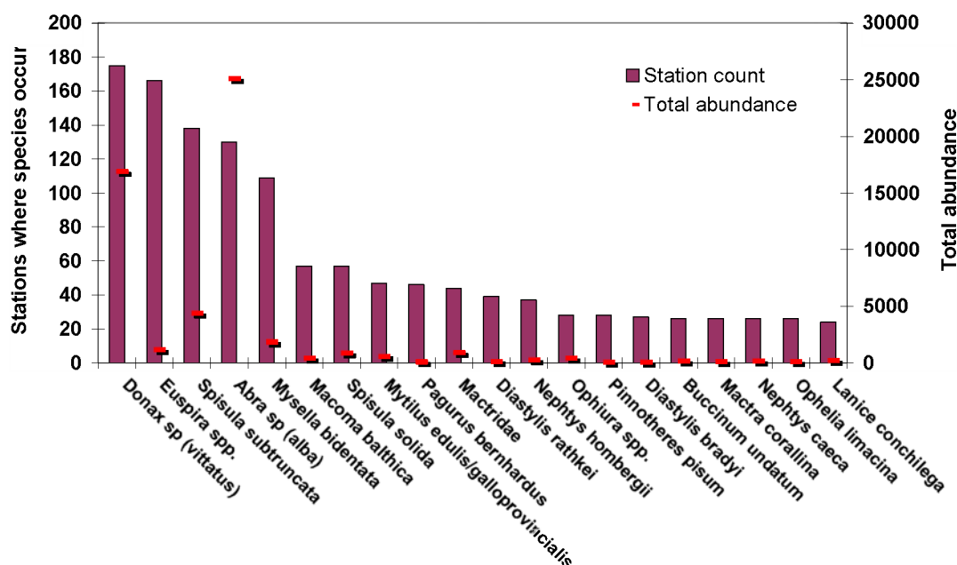
Figure 2.3-1: Most widespread (station occupancy) and abundant (total abundance) macrobenthic species within the historic data; period 1899-1911. Sampling gear: dredge.
