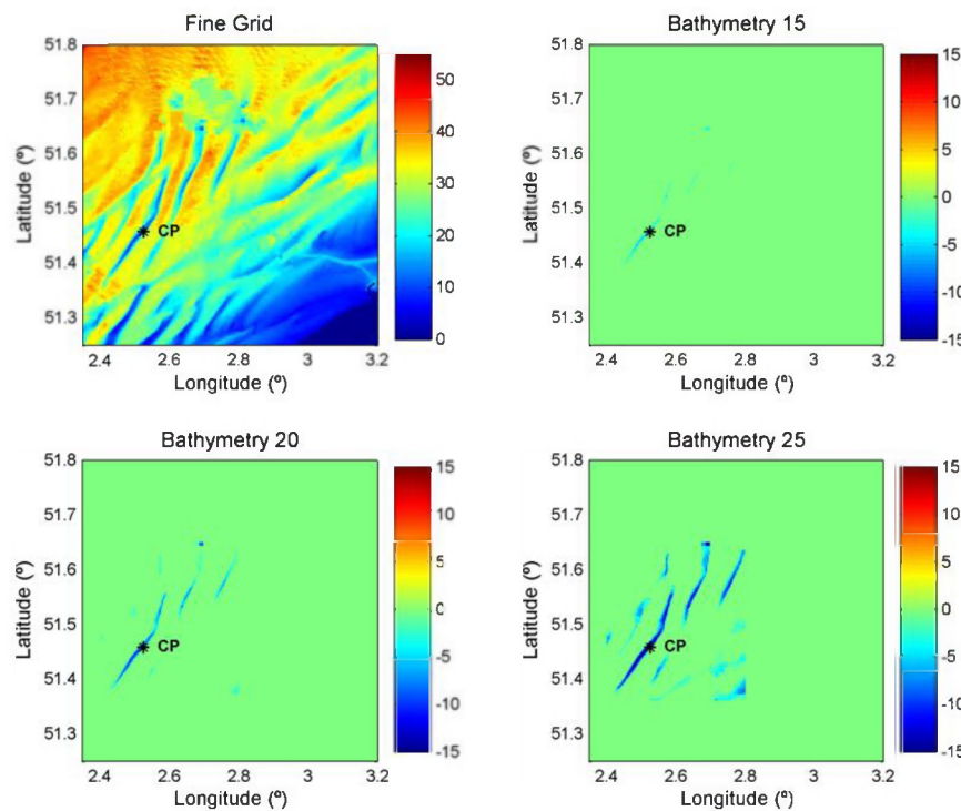
Figure 3.4-6. Zoom of the differences between the fine-scale bathymetry grid and the adapted bathymetries (lower to 15, 20 and 25 meters depth). CP is a control point for output comparison.
