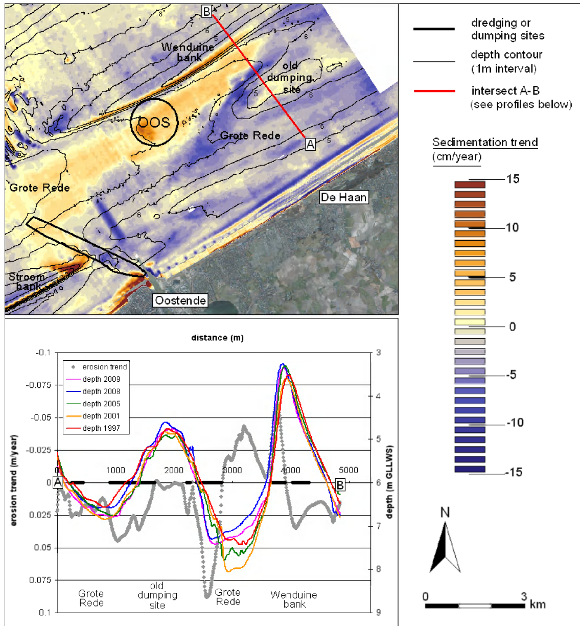
Figure 3.3-5. Top figure: erosion-sedimentation trend for beach, foreshore and the nearshore between Ostende and De Haan. Bottom figure: depth profiles (solid lines, right vertical axis) and erosion trend profile (dotted line, left vertical axis) along cross section A-B.
