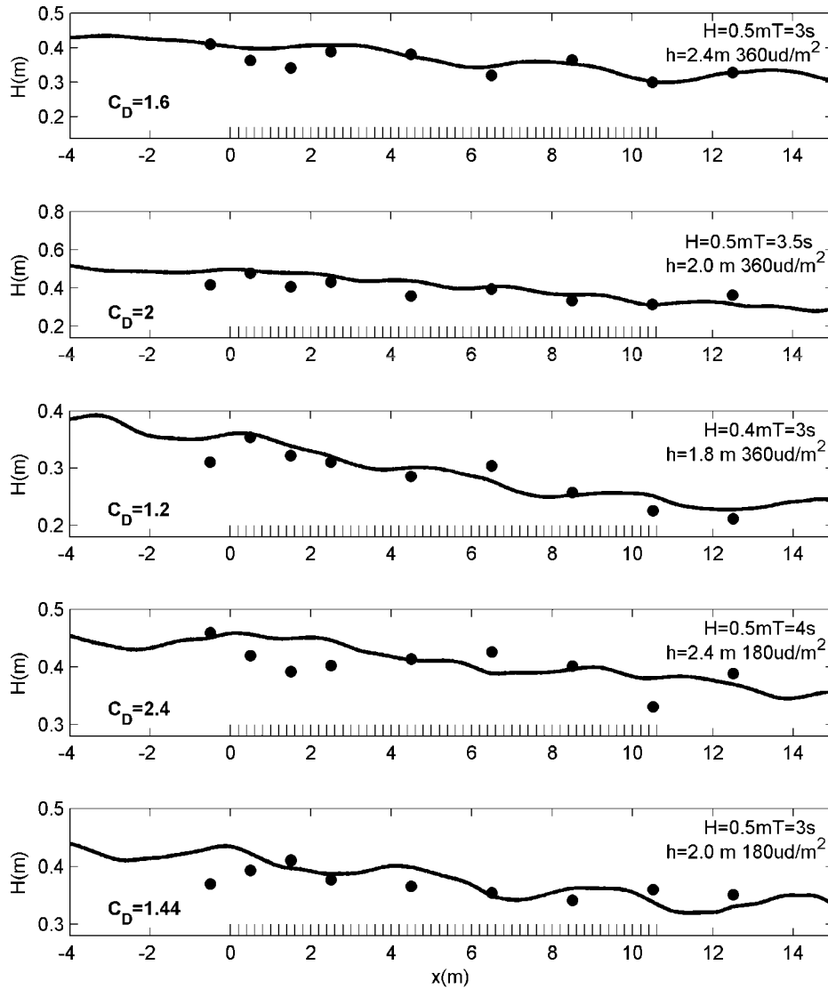
Figure 1. Wave evolution validation using Stratigaki et al. (2011) experiments. Black solid line represents the numerical results and black dots the laboratory measurements. Wave height (H), wave period (T), water depth (h) and density ( \text{ud/m}^2 ) are displayed as well as the drag coefficient ( C_D ).
