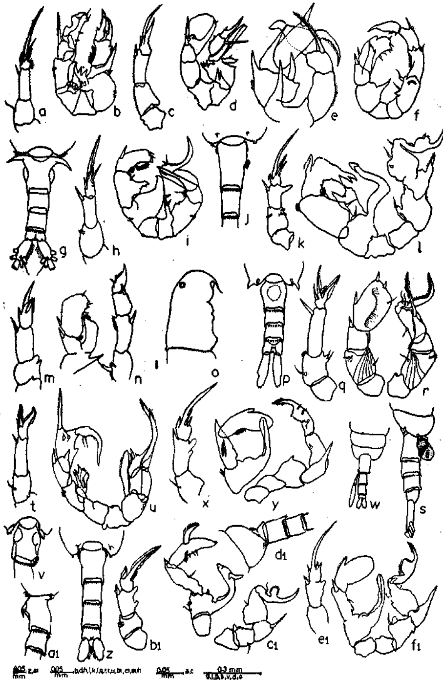
Fig. 1. a. Pseudodiptomus mertoni , female, P5; b. male P5; c. P. aurivillii , female P5; d. male P5; e. P. daughtshi male P5; f. P. batillipes , male P5; g. P. annandalei , female urosome, dorsal view; h. female P5; i. male P5; j. P. tollingeriae , female urosome, dorsal view; k. female P5; l. male P5; m. P. pauliani , female P5; n. male P5; o. P. clevei , cephalon of female, lateral view; p. female urosome, dorsal view; q. female P5; r. male P5; s. female urosome, lateral view; t. P. serricaudatus , female P5; u. male P5; v. female urosome, lateral view; w. P. lobipes , female urosome, dorsal view; x. female, P5; y. male P5; z. P. binghami malayalus , female urosome, dorsal view; a1: female urosome, lateral view; b1: female, P5; c1: male P5; d1: P. binghami , male urosome, lateral view; e1: female, P5; f1: male P5. Figs. e (after Sewell, 1932); f (after Brehm, 1951); m & n (after Brehm, 1954); w-y (after Gurney, 1907).
