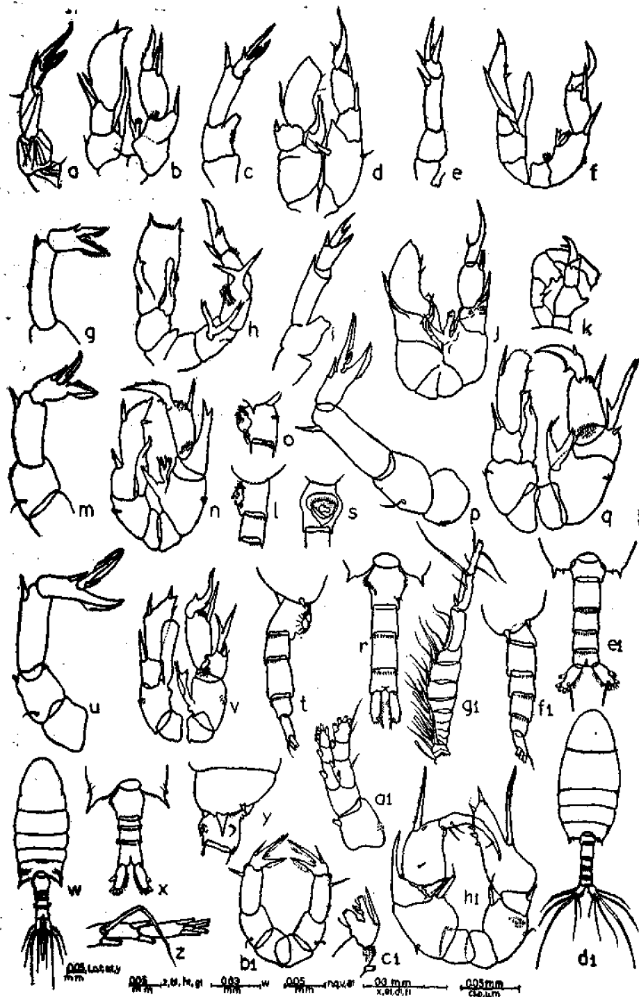
Fig. 2. a. Pseudodiaptomus salinus , female P5; b. male P5; c. P. charteri , female P5; d. male P5; e. P. cornutus , female P5; f. male P5; g. P. hickmani , female P5; h. male P5; i. P. stuhlmanni , female P5; j. male P5; k. P. heterothrix male P5; l. P. jonesi , female urosome, lateral view; m. female P5; n. male P5; o. P. ardjuna , female urosome, lateral view; p. female, P5; q. male P5; r. P. marinus , female urosome, dorsal view; s. female, genital segment, ventral view; t. female urosome, lateral view; u. female P5; v. male P5; w. P. burckhardtii , female dorsal view; x. female urosome, dorsal view; y. female TV and genital segment, lateral view; z. female, A-1 distal segments enlarged; a 1. female, P4; b 1. female P5; c 1. Re of female P5, distal segment enlarged; d 1. male, dorsal view; e 1. male urosome, dorsal view; f 1. male urosome, lateral view; g 1. male A-1; h 1. male P5.
