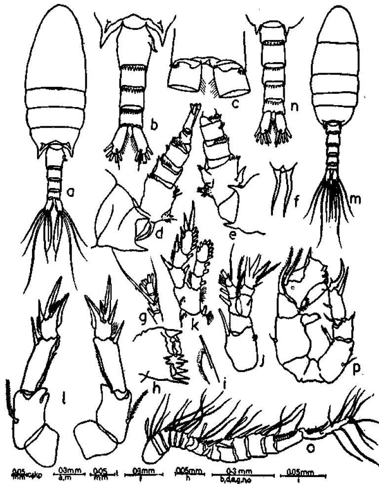
Fig. 3. Pseudodiaptomus andamanensis sp. nov. a. female, dorsal view ; b. female urosome, dorsal view ; c. female, TV and caudal rami, enlarged ; d. female urosome, right lateral view ; e. female urosome, left lateral view ; f. rostrum, female ; g. distal segment of female A-1 enlarged ; h. Mnd ; i. distal enlargement of seta on Mxp ; j. female P1 ; k. female P2 ; l. female P5 ; m. male dorsal view ; n. male urosome, dorsal view ; o. male A-1 ; p. male P5.
