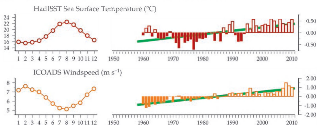
Figure 9.1.3 Regional overview plot (see Section 2.2.3) showing long-term sea surface temperatures and windspeeds in the general region surrounding the Málaga Bay monitoring area.
