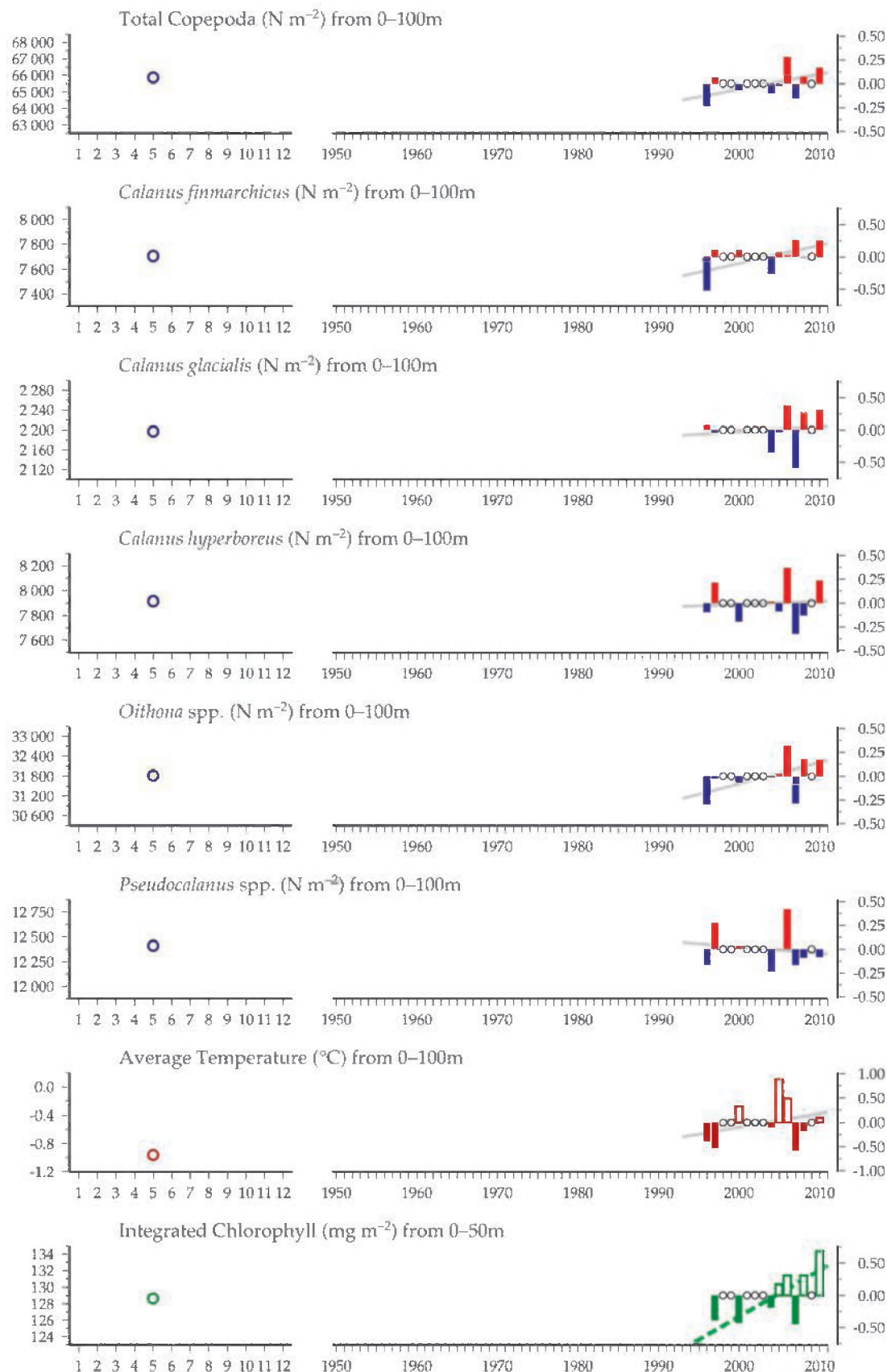
Figure 4.2.2 Multiple-variable comparison plot (see Section 2.2.2) showing the seasonal and interannual properties of select cosampled variables at the AR7W Labrador Shelf zooplankton monitoring area (data collected in late May only).
