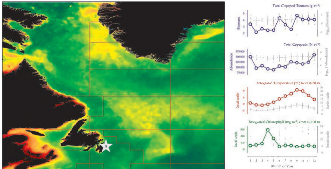
Figure 4.1.1 Location of the Station 27 monitoring area (Site 9) plotted on a map of average chlorophyll concentration, and its corresponding seasonal summary plot (see Section 2.2.1).
