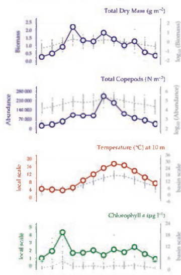
Seasonal Summary Plot
