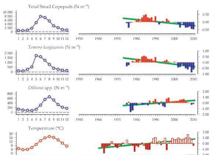
Multiple-Variable Comparison Plot
