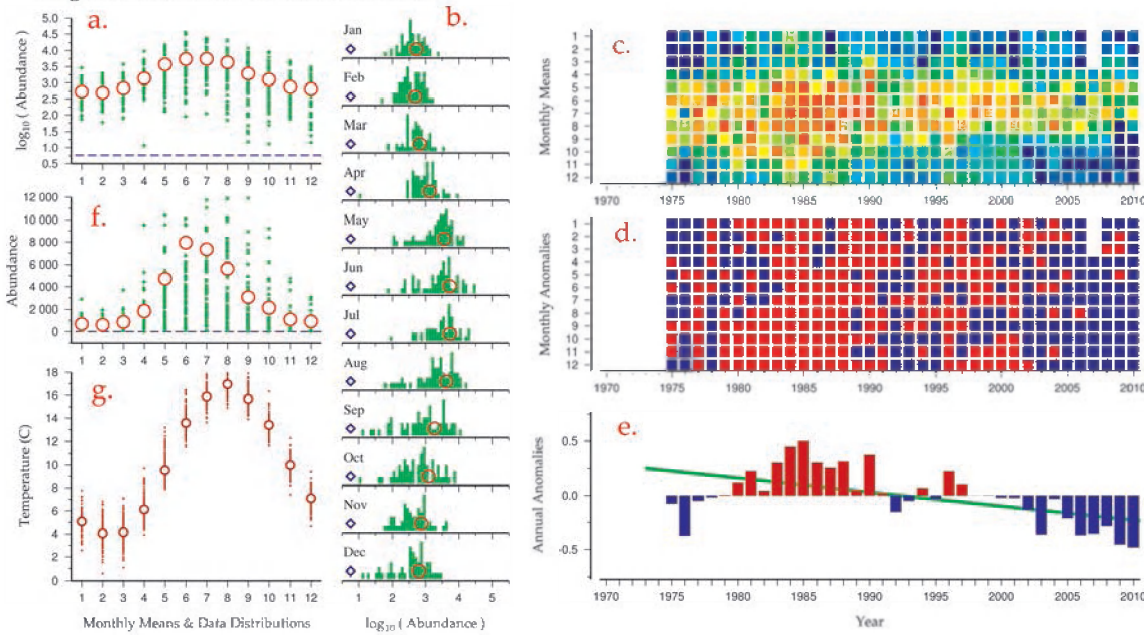
Figure 2.1.1 A collection of standard WGZE time-series visualization figures illustrating the steps and components used in the WGZE analysis for creating annual anomalies of total small copepod abundance from the Helgoland Roads time-series (Site 45, see Section 7.2 for more information on this site).
