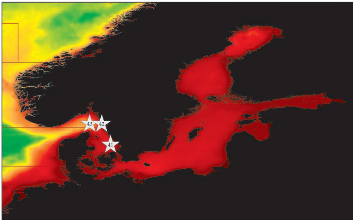
Figure 6.8.1 Locations of the Swedish Meteorological and Hydrological Institute (SMHI) survey areas in the Kattegat and Skagerrak region (Sites 41–43), and their corresponding seasonal summary plot (see Section 2.2.1).
