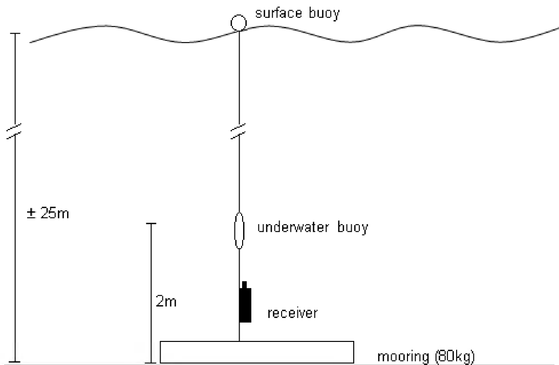
Figure 1. Receiver mooring scheme used in the present study.
