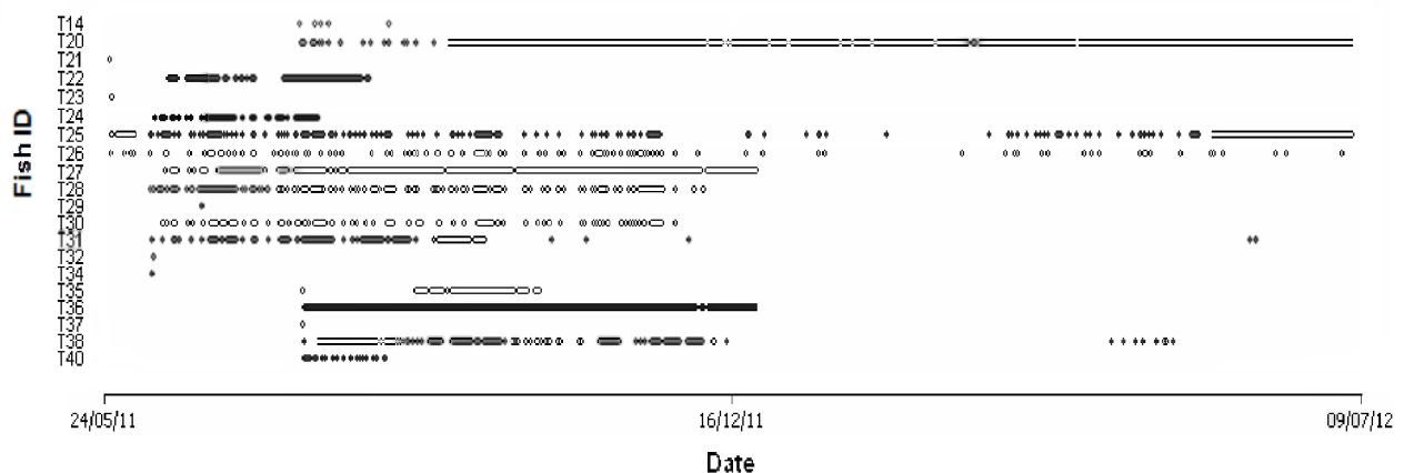
Figure 4. Overview of detections of all tagged Atlantic cod; from 24 th of May 2011 until 9 th of July 2012 (based on information of 2 receivers). Each line represents the detections of one fish.
