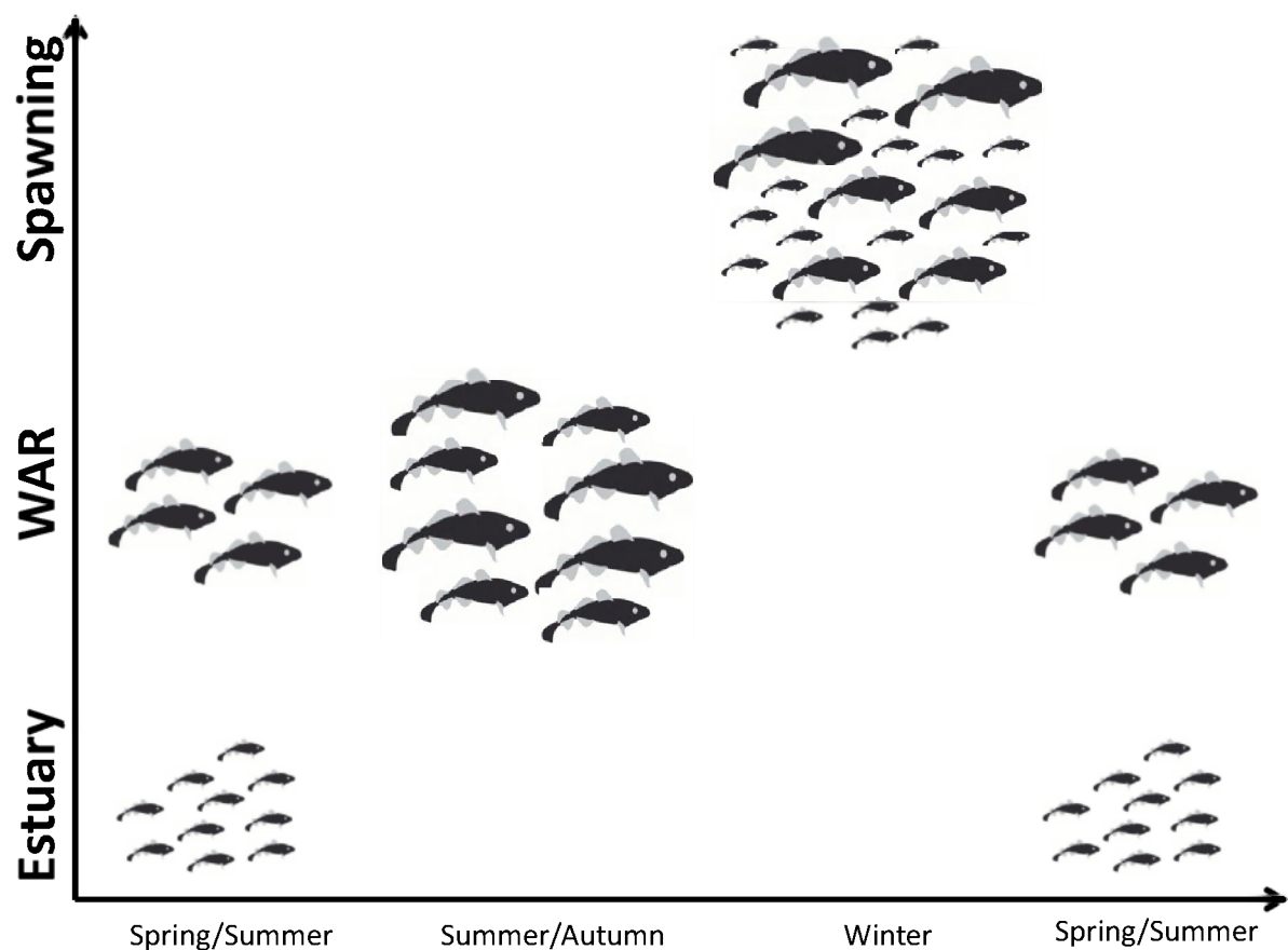
Figure 6. Conceptual representation of the life history of pouting occurring at the WARs. In spring the O-group lives in estuaries, while the I-group is present at the WARs. Both groups grow and by Autumn the O-group moved towards the WARs. By winter time they leave the area and move towards the spawning locations (now they became the I- and II-group). After spawning, the newly hatched O-group pouting arrive at the estuaries while the I-group pouting move back to the WARs. Older age groups probably move elsewhere.
