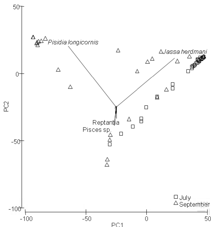
Figure 2. Numeric PCA based on density ratio of the most important prey items. Axes 1 and 2 explain 66 % and 15 % of the total variation respectively.
