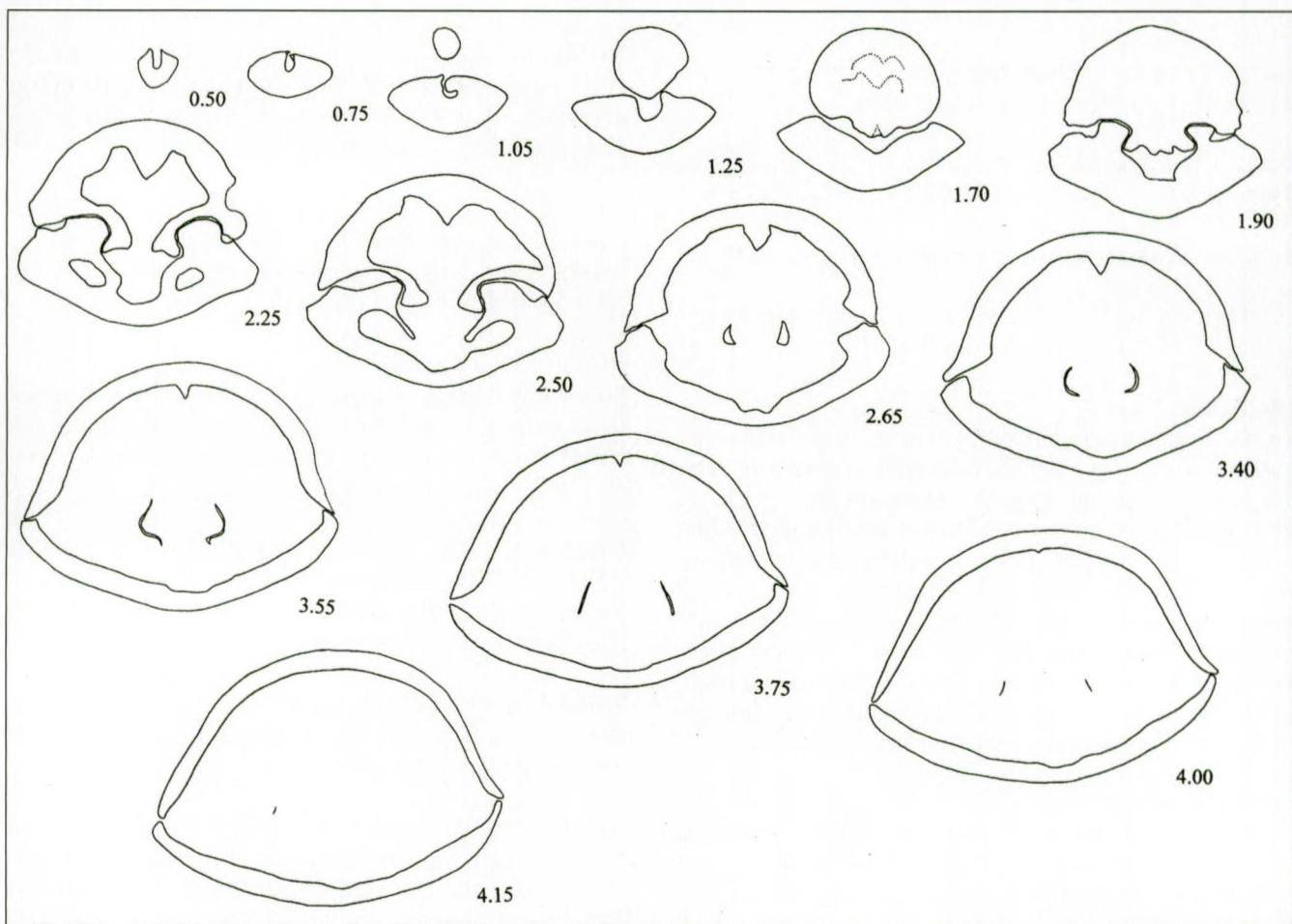
Fig. 3 — Transverse serial sections through the umbonal portion of an adult specimen (NHMM GK 1378, ex Felder colln., paratype) of Cretirhynchia ( Homaletarhynchia ) postarcuata n. sp., from Zeven Wegen in Vijlenerbosch (62D-15d), Vijlen, southern Limburg, The Netherlands. Lower Maastrichtian, Gulpen Formation, base of Vijlen Member. x 4.0
