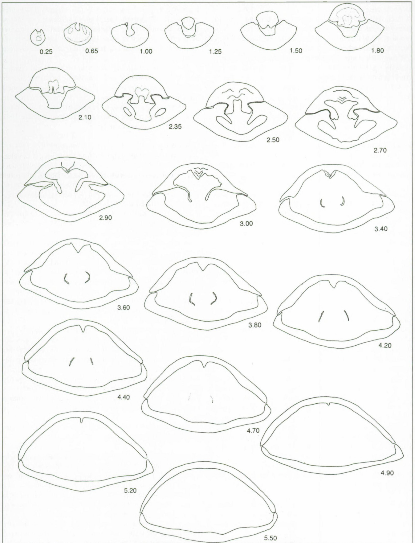
Fig. 4 — Transverse serial sections through the umbonal portion of an adult specimen (NHMM GK 941, ex Felder colln., paratype) of Cretirhynchia ( Homaletarhynchia ) postarcuata n. sp., from Vijlenerbosch (62D-15), Vijlen, southern Limburg, The Netherlands. Lower Maastrichtian, Gulpen Formation, base of Vijlen Member. x 4.84
