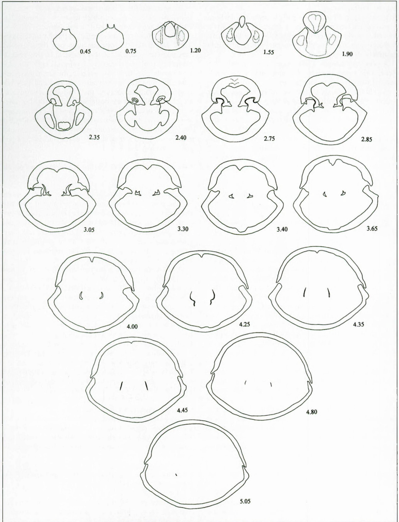
Fig. 2 — Transverse serial sections through the umbonal portion of an adult specimen (NHMM GK1379, ex Felder colln., paratype) of Woodwardirhynchia pseudonorvicensis n. sp., from Zeven Wegen in Vijlenerbosch (62D-15d), Vijlen, southern Limburg, The Netherlands. Base of the Vijlen Member (Gulpen Formation, Lower Maastrichtian). x 4.1
