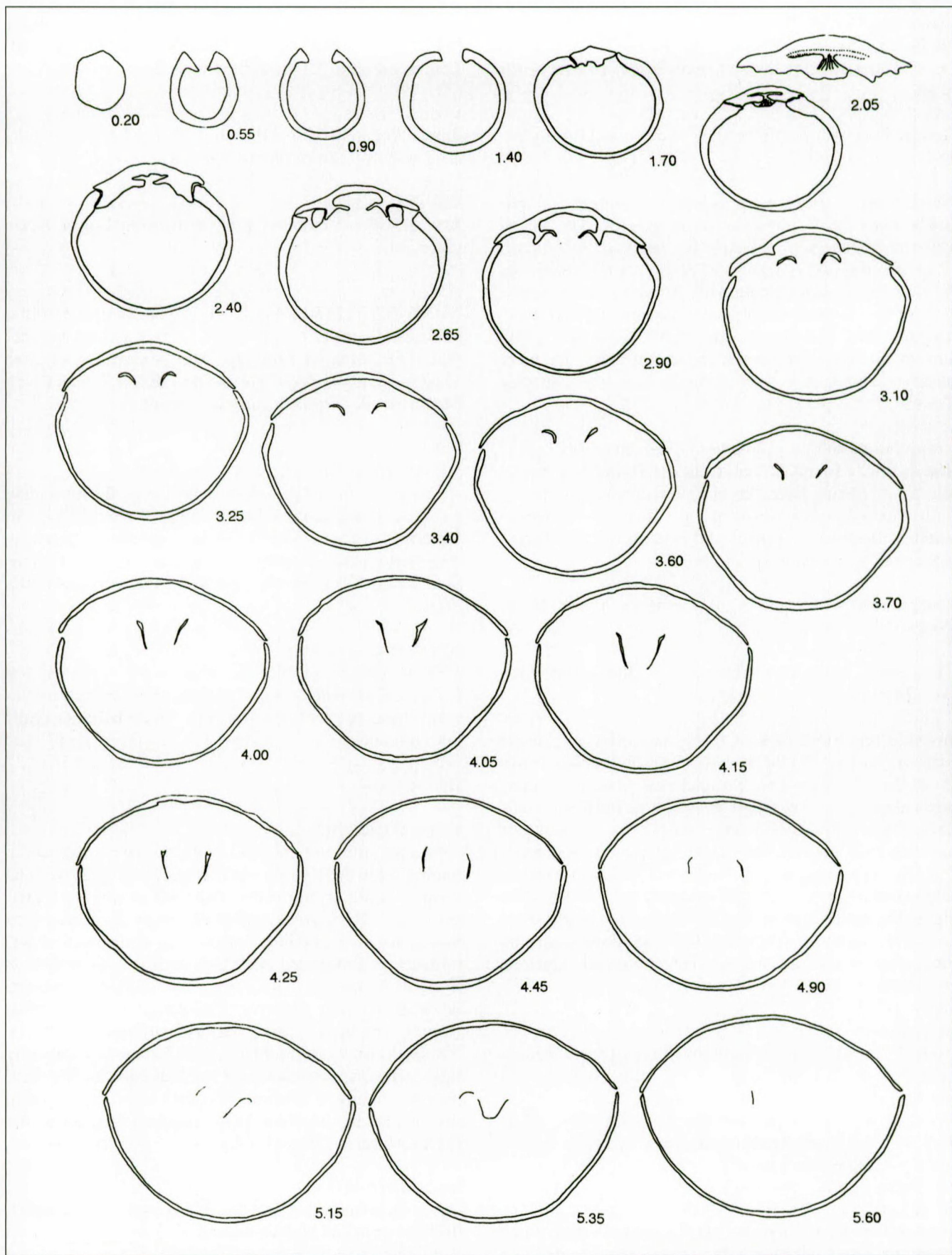
Fig. 6 — Transverse serial sections through the umbonal portion of an adult specimen (NHMM GK 475, ex Felder colln., holotype) of Nerthebrochus sulcata n. sp., from Nieuwe Weg, Zeven Wegen in Vijlenerbosch (62D-15b), Vijlen, southern Limburg, The Netherlands. Lower Maastrichtian, Gulpen Formation, base of Vijlen Member. X 5.1
