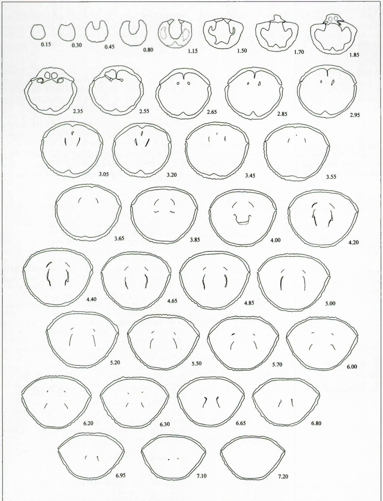
Fig. 8 — Transverse serial sections through the umbonal portion of an adult specimen (NHMM GK 1317, ex Felder colln., paratype) of Maastrichtiella costellata n. sp. from Slenaken-Kerkdel (62C-15), southern Limburg, The Netherlands. Lower Maastrichtian, Gulpen Formation, base of the Vijlen Member. x 5.0
