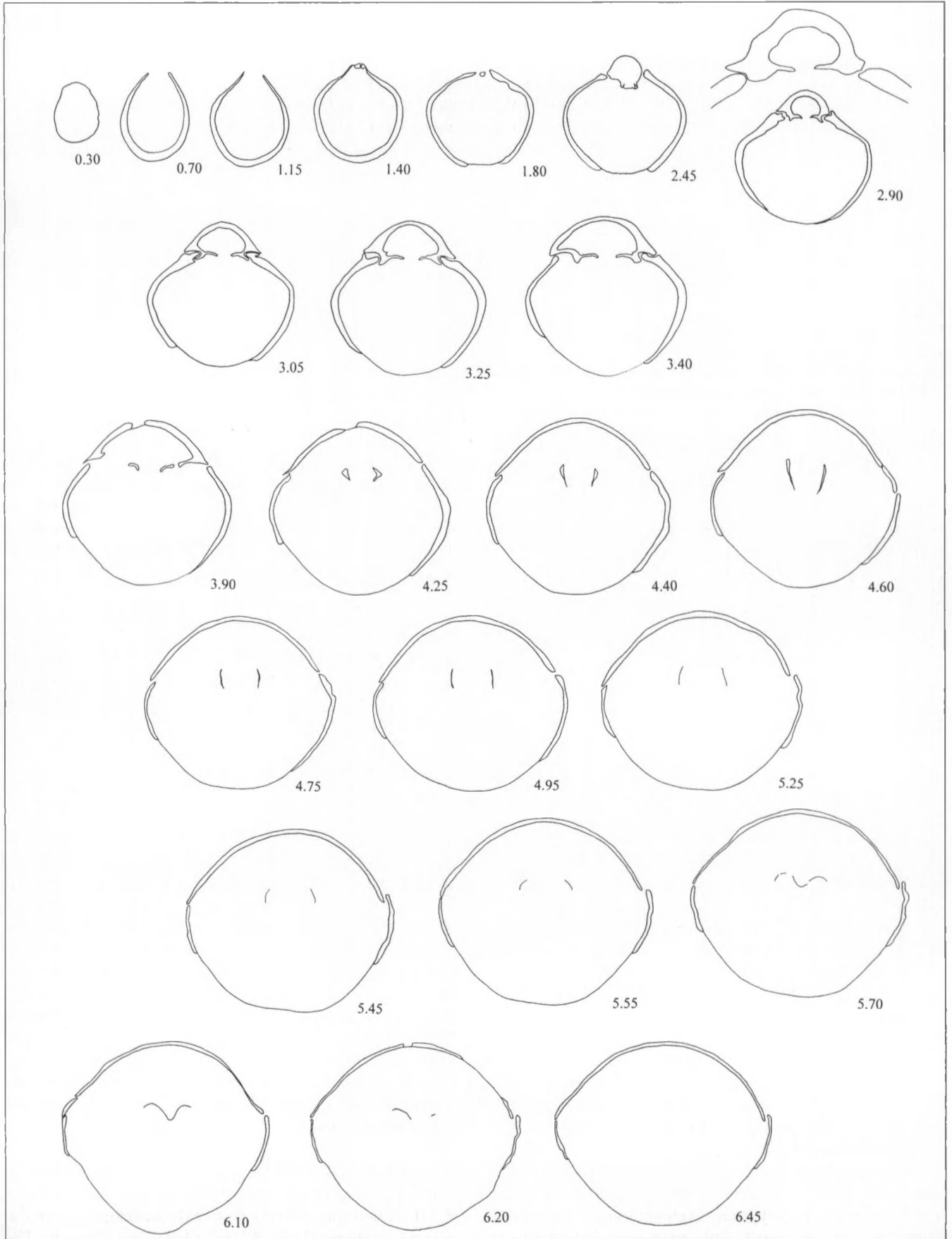
Fig. 5 — Transverse serial sections through the umbonal portion of an adult specimen (NHMM GK 1341, ex Felder colln., paratype) of Nerthebrochus ovalis n. sp., from Zeven Wegen in Vijlenerbosch (62D-15d), Vijlen, southern Limburg, The Netherlands. Lower Maastrichtian, Gulpen Formation, base of the Vijlen Member. x 3.75
