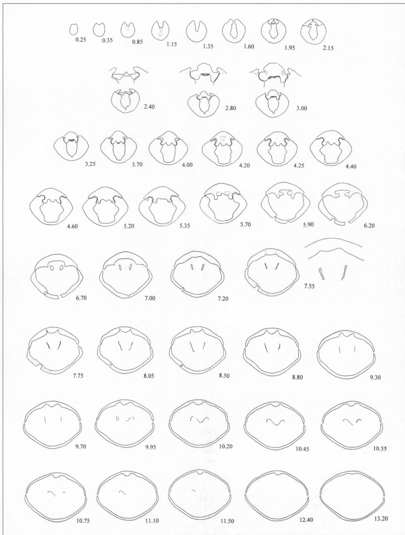
Fig. 7 — Transverse serial sections through the umbonal portion of an adult specimen (NHMM GK 1229, ex Felder colln.) of Carneithyris sp., from Slenaken-Kerkdel (62C-15), southern Limburg, The Netherlands. Lower Maastrichtian, Gulpen Formation, base of the Vijlen Member. x 1.54
