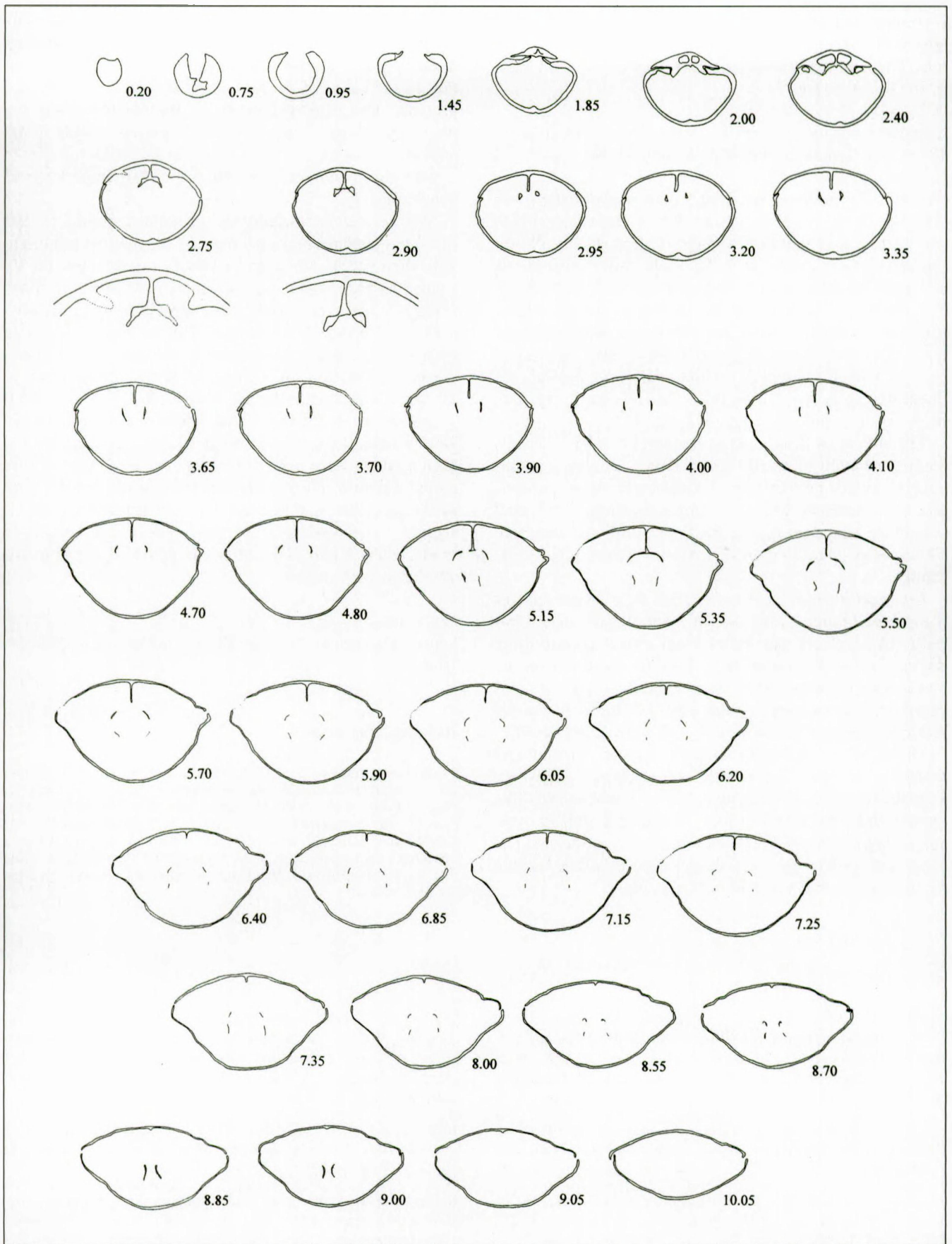
Fig. 9 — Transverse serial sections through the umbonal portion of an adult specimen (NHMM GK 1348, ex Felder colln., paratype) of Mosaethyris felderi n. sp. from Nieuwe Weg, Zeven Wegen in Vijlenerbosch, Vijlen, southern Limburg, The Netherlands. Lower Maastrichtian, Gulpen Formation, base of the Vijlen Member. x 3.05
