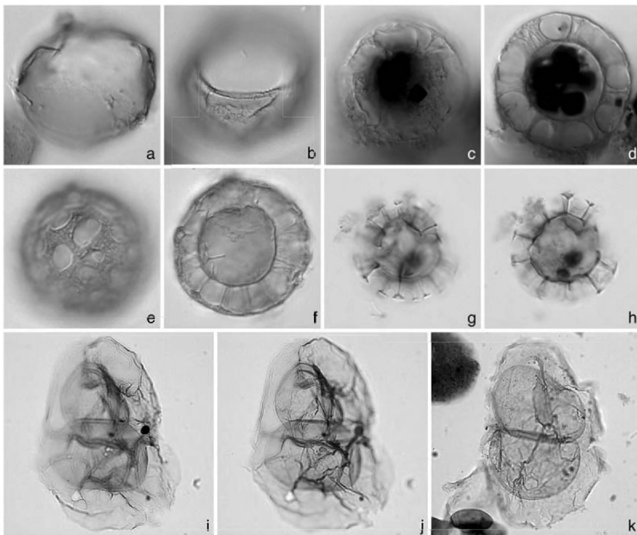
Figure 12. Acritarchs (t, s) from the Verrebroek Dock (VBD) and Deurganck Dock (DGD) sections. Various magnifications. Max. dia. = Maximum diameter. (a, b) Paleostomocystis globosa Louwey. Antapertural view at (a) mid focus, and (b) apertural surface; max. dia., 39 \mu\text{m} ; sample VBD 4.5 p2, X48/0. (c, d) Acritarch sp. 1 of Head, Norris & Mudie (1989). (c) upper surface, and (d) mid focus; overall max. dia., 33 \mu\text{m} ; sample VBD 4.5 p2, Q33/0. (e, f) Cyst type 1 of de Vernal & Mudie (1989). (e) upper surface, and (f) mid focus; overall max. dia., 30 \mu\text{m} ; sample DGD 22, G30/0. (g, h) Algal cyst sp. 1 of Head (1996). (g) upper surface. (h) mid focus; central body max. dia., 17 \mu\text{m} ; sample DGD 22, L52/3. (i–k) Incertae sedis 1. (i, j) upper and mid foci respectively; max. length, 167 \mu\text{m} ; sample VBD 2.6 p1, X19/2. (k) mid focus; max. length, 120 \mu\text{m} ; sample DGD 8, V44/2.
