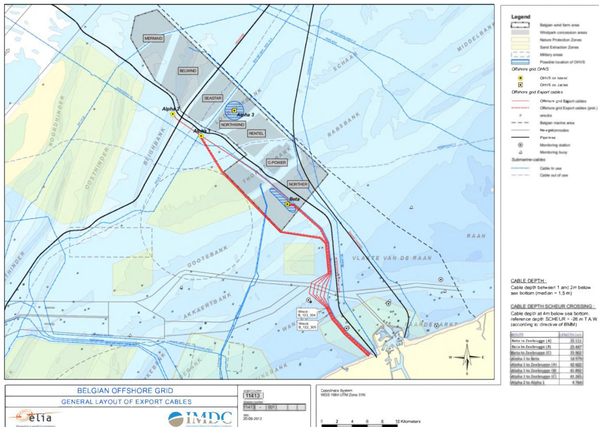
Figuur 38: Belgian Offshore Grid [Bron: Elia (2012)].
