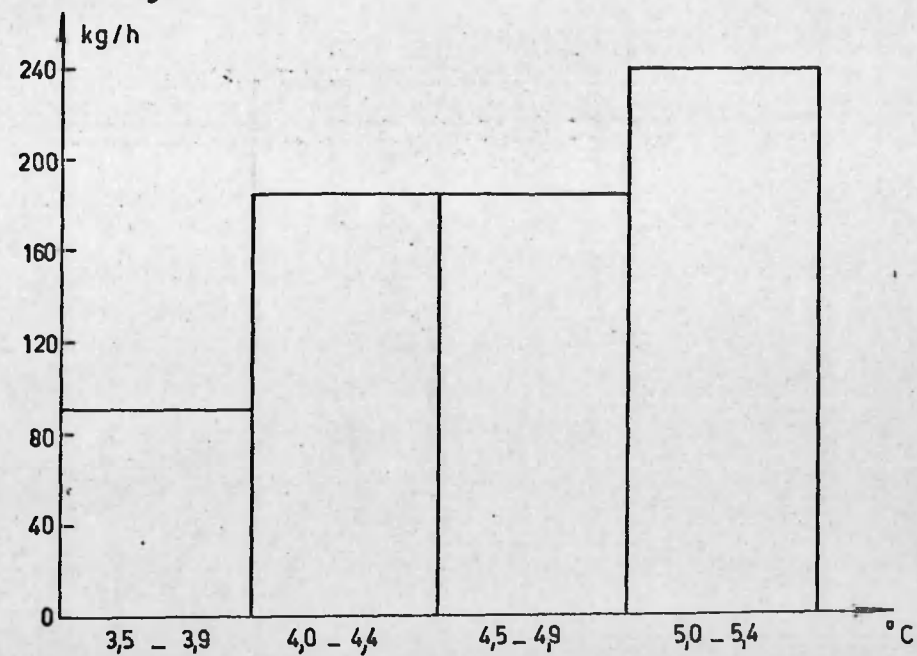
Figure 5 - Catch of saithe in relation to temperature
