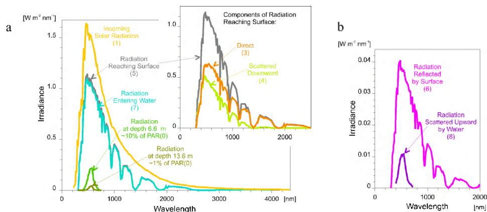
Figure 6 Spectra of a) downward and b) upward radiation fluxes (example values for May 15, solar noon, site 1).
