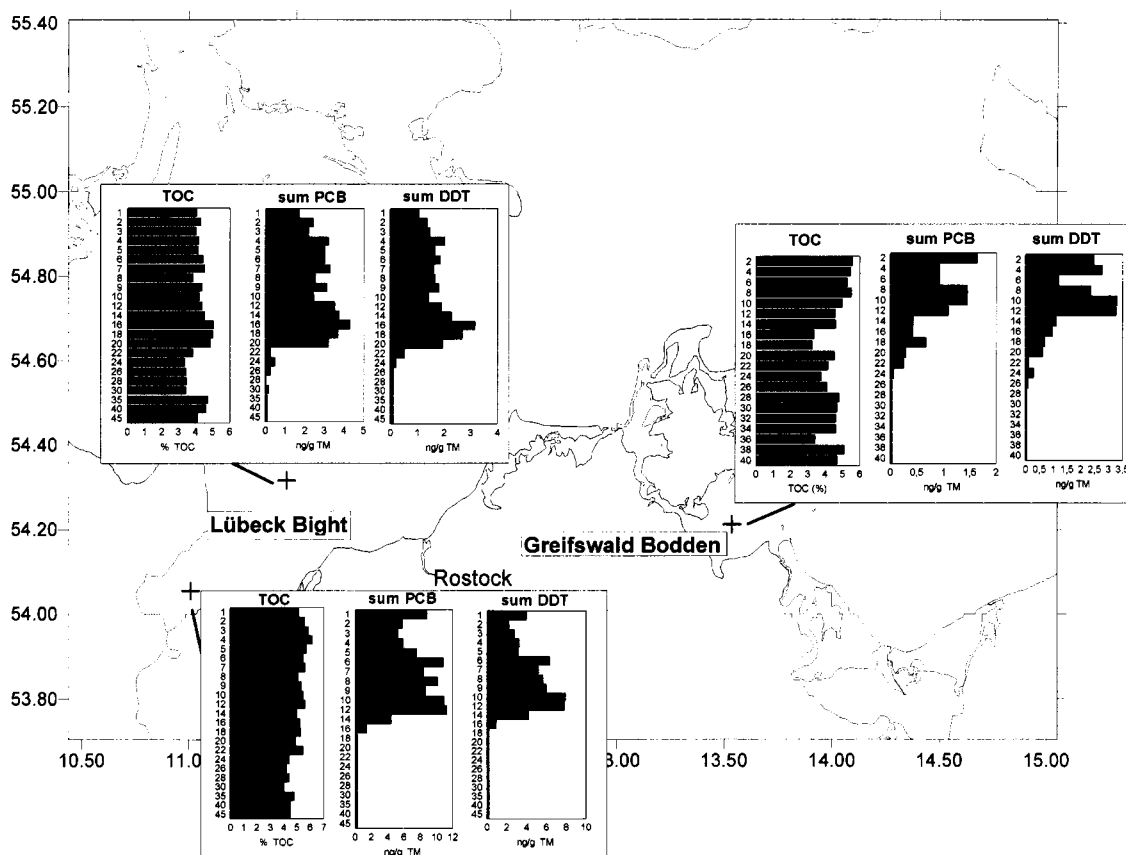
Figure 4 Vertical distribution of TOC, CBs and DDTs in sediment cores of the Lübeck Bight and the Greifswald Bodden
