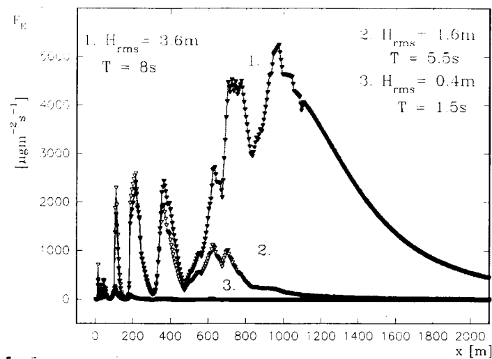
Figure 3 The aerosol emission flux obtained from model for three boundary conditions for the sea bottom profile in Lubiato
