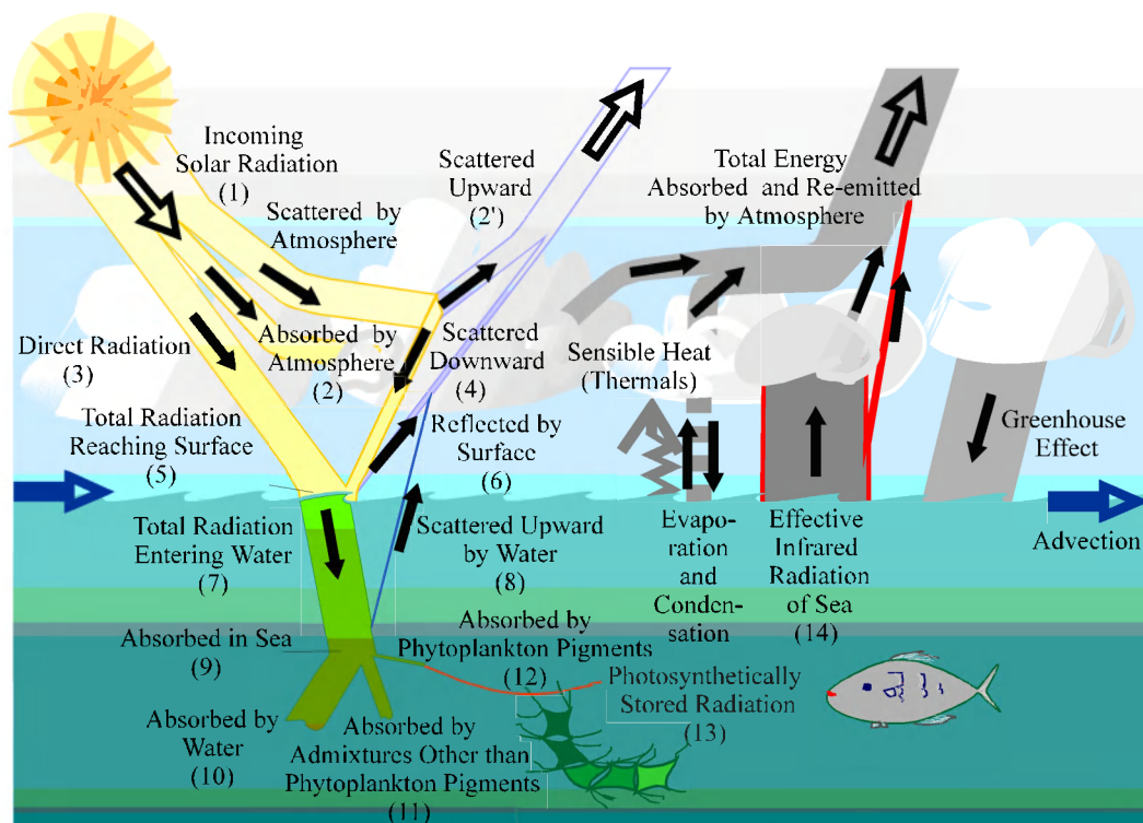
Figure 1 The main elements of energy balance in the atmosphere-sea system
