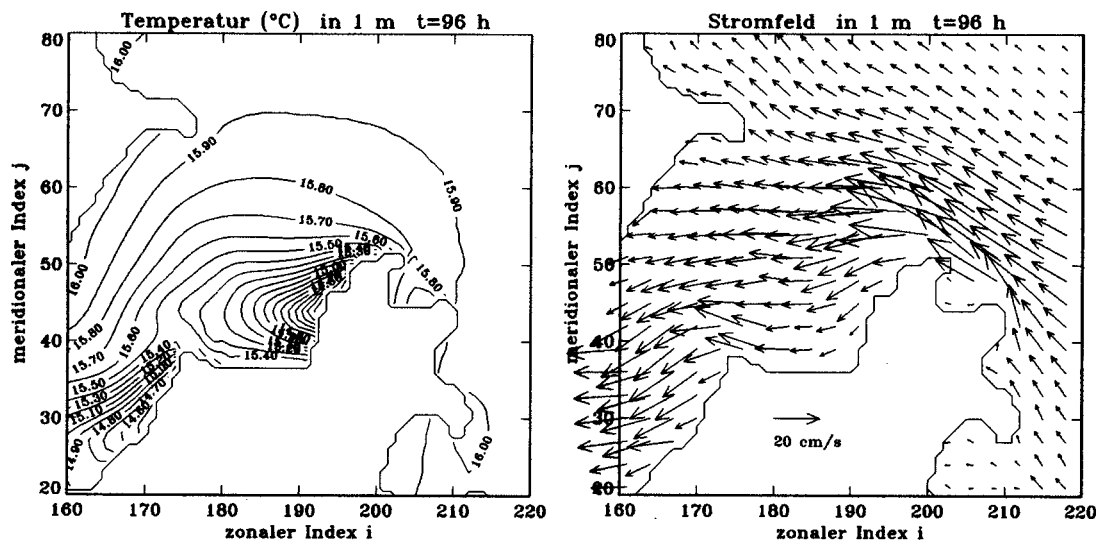
Figure 7 Modelled sea surface temperature (left) and current (right), 96 h after a step-like lowering of the sea level of the North Sea by 30 cm and the onset of a localised east wind in the Western Baltic
