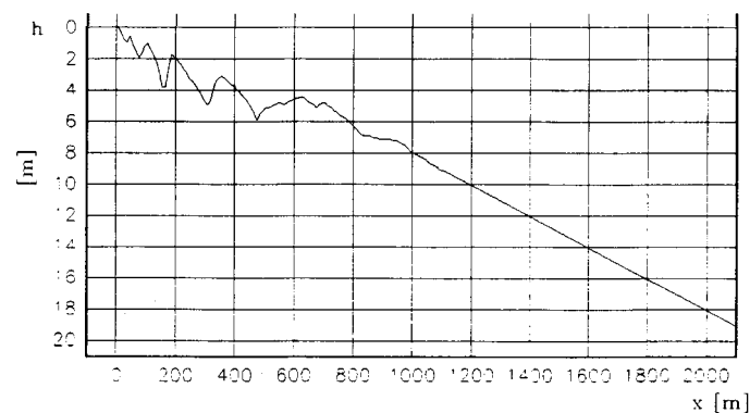
Figure 4 The sea bottom profile in Lubiato (BAEX I. II)
