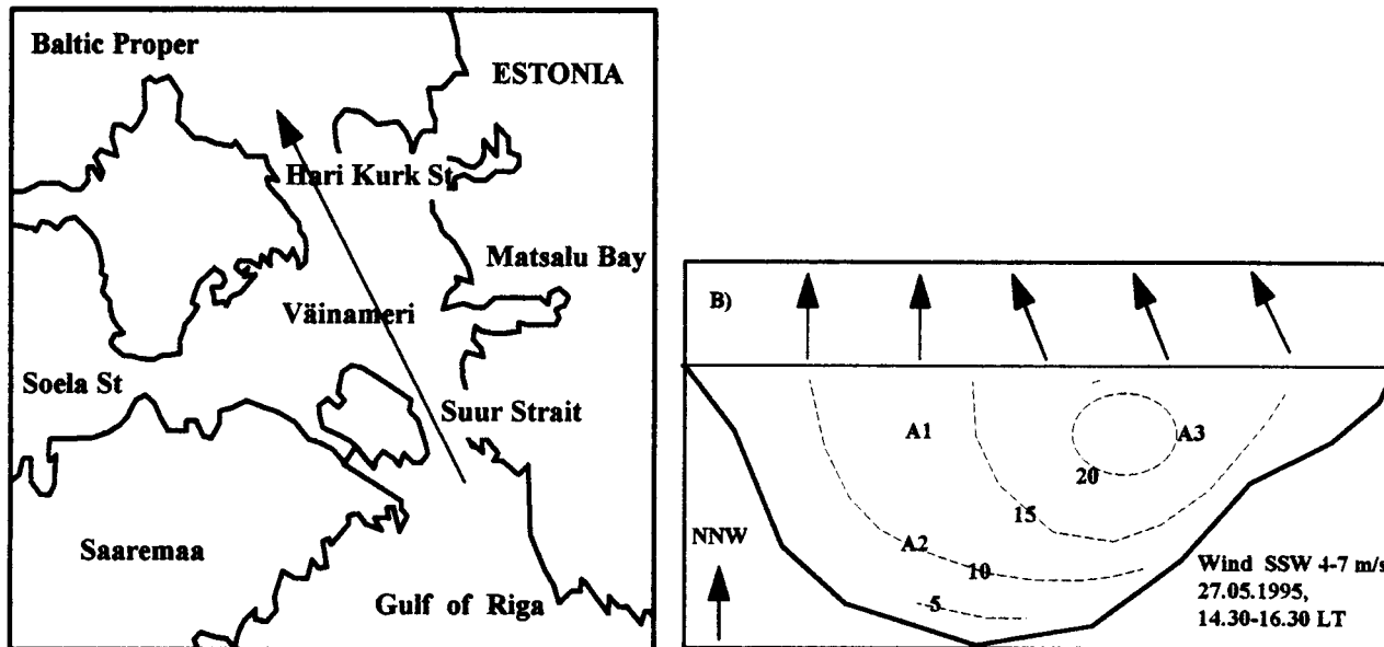
Figure 1 The Väinameri area and the cross-section of the Suur Strait; current velocities in \text{cm s}^{-1} . A1, A2 and A3 mark the positions of the mooring stations.
