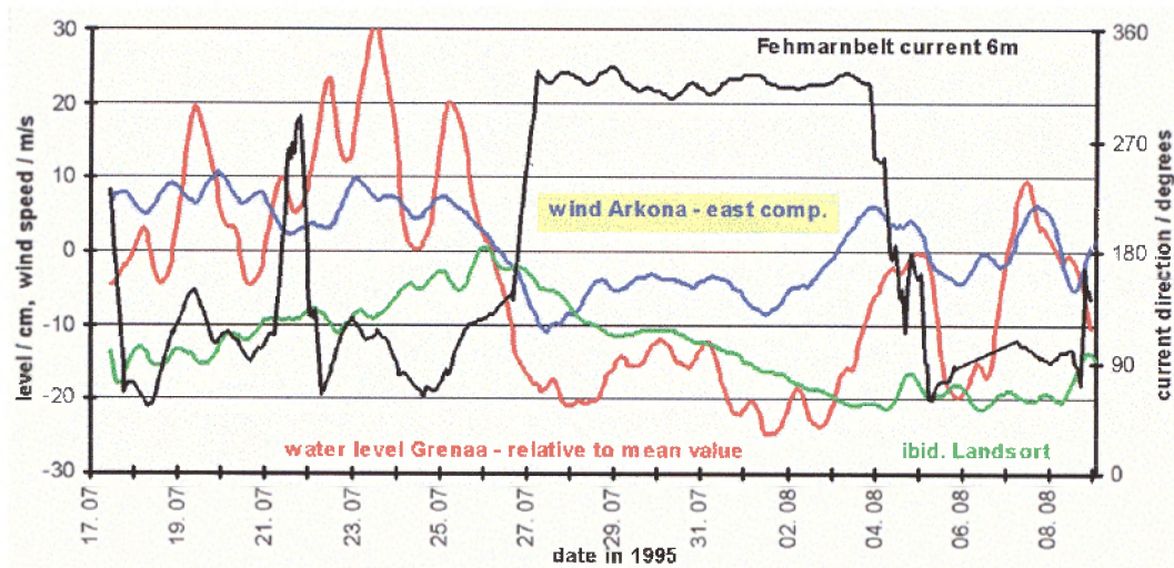
Figure 5 Time series of east component of wind velocity measured at the meteorological station Arkona (blue), sea level at Grenaa in the Kattegat (red) and Landsort in the Baltic proper (green), and direction of current measured in the Fehmarn Belt at a depth of 6 m (black). Outflow from the Baltic Sea toward the Kattegat is about 310^\circ in the Fehmarn Belt.
