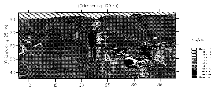
Figure 11 Bottom divergence ( \text{cm year}^{-1} ) in Kuznica A and Kuznica B pits area, wind NW 15\text{ms}^{-1} .
