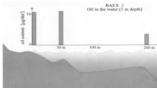
Figure 3 Concentration of hydrocarbons in subsurface layer as related to offshore distance
