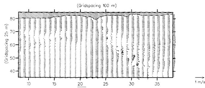
Figure 10 Depth integrated current field in Kuznica A and Kuznica B pits area, wind NW 15\text{ms}^{-1} .
