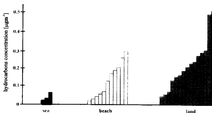
Figure 7 Concentrations of hydrocarbons in air as related to air advections from sea, beach and land
