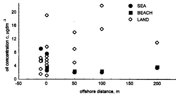
Figure 8 Concentration of hydrocarbons in seawater for different wind sectors: from sea, from land or along the coast.
