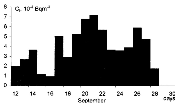
Figure 1 Course of the ^7\text{Be} concentration in the air over the beach in Lubiato during BAEX-3 (1995)
