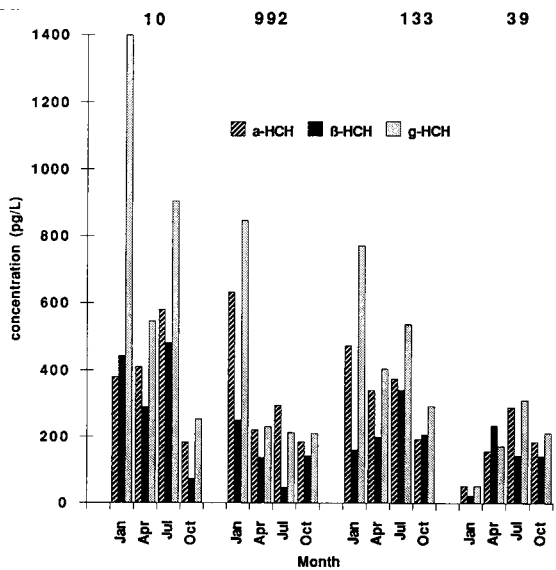
Figure 7 Seasonality of HCH-isomers in solution in the Pomeranian Bight in 1995
