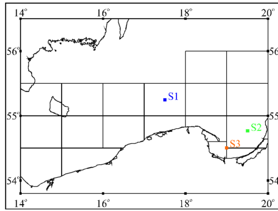
Figure 4 Location of sites for which radiative energy budget components are modelled
