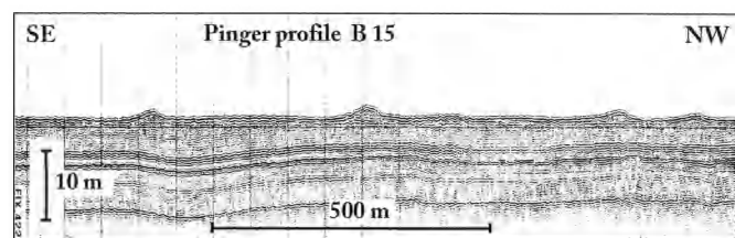
Figure 4 Pinger profile (B15) of isolated sand-silt waves in the central part of Fehmarn Belt. Location indicated on Figure 1.
