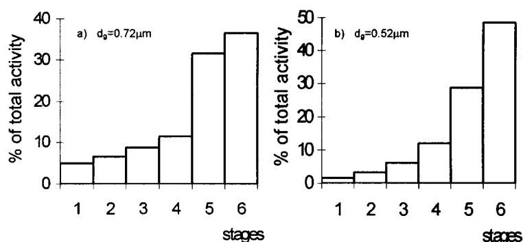
Figure 2 ^7\text{Be} carrier size g-activity distribution in the air over the beach in Lubiato during BAEX-3:
