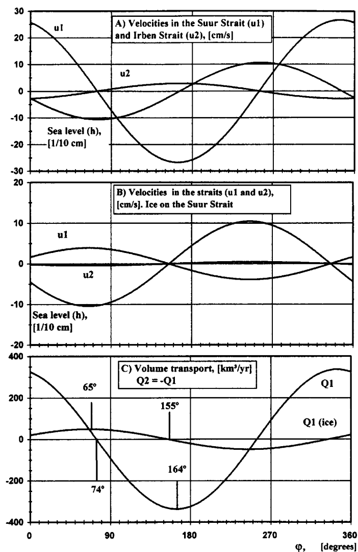
Figure 2 Dependence of velocities and volume transports in the Suur Strait and the Irben Strait on the wind direction ( \varphi , module = 7\text{ m s}^{-1} ) and on existence of ice in the Suur Strait area. Q_j = H_1 = H_2 = 0 .
