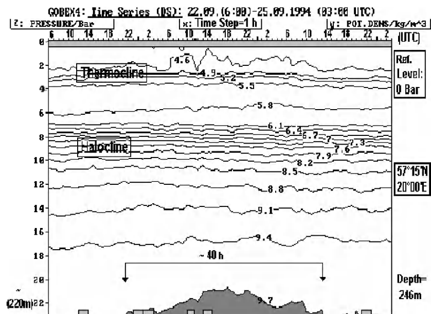
Figure 4 Plotted time series of the potential density (PD) sampled with a time step of 1 h at the position of station BY15A above the Gotland Deep according to Hagen and Feistel (1996); \text{PD} > 9.7 \text{ kg m}^{-3} is black
