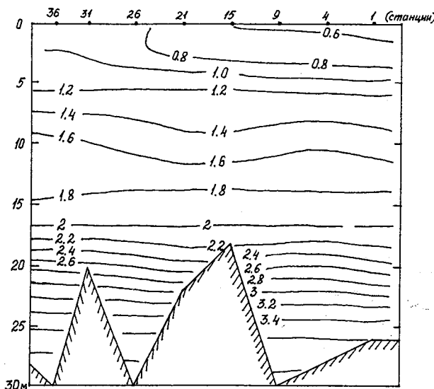
Figure 5 Distribution of density relation R_p = -E_T/E_S at the transect along the parallel of latitude 60^\circ N (stations 36-31-26-21-15-9-4-1)
