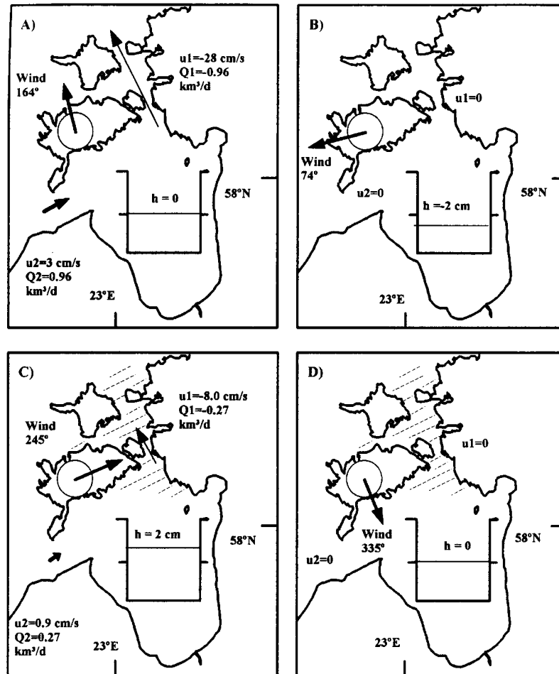
Figure 3 Water exchange and mean sea level in the Gulf of Riga for some special wind directions ( \tau=1 \text{ cm}^2 \text{ s}^{-2} , Q_2=-Q_1 , see also Figure 2). A and B show the situation without ice while C and D show ice on the Vāinameri area (typical winter situation). The situation with the wind from 344^\circ is similar to A but with opposite flows in the straits; 254^\circ is similar to B but with the sea level h=2 \text{ cm} ; 65^\circ is similar to C but with the sea level h=-2 \text{ cm} and 155^\circ is identical to D.
