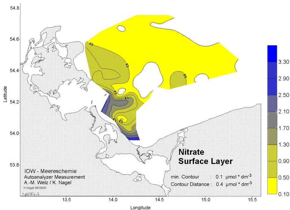
Figure 7 Distribution pattern of nitrate in September 1995. Samples have been taken from the surface layer at the first sampling from the grid stations.
