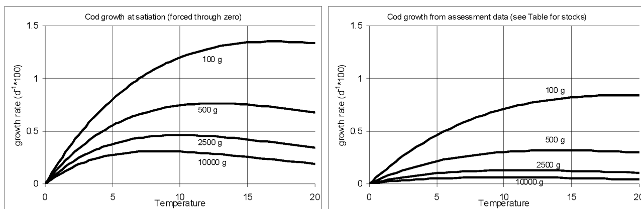
Figure 3.3 Three parameter growth model fitted to Björnsson's satiation reared cod and to assessment data.
