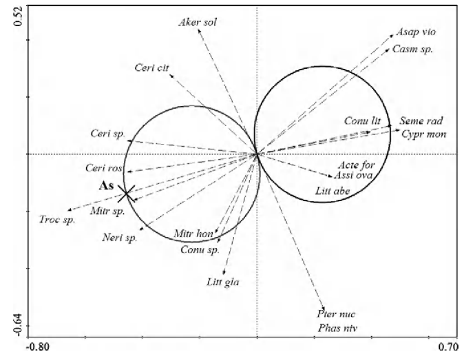
Fig. 8. T-value biplot showing the relationship between intertidal molluscs and the environmental variable As at the Dar es Salaam coast, Tanzania. Species are represented by dashed arrows and the environment variable by a symbol X. Species with arrow tips enclosed within the van Dobben circle are significantly positively related with that variable. Asap vio = Asaphis violascens , Acte for = Acteon fortis , Aker sol = Akera soluta , Assi ova = Assiminea ovata , Casm sp = Casmaria sp. , Ceri cit = Cerithium citrinum , Ceri ros = Cerithium rostratum , Ceri sp. = Cerithium sp. , Conu sp = Conus sp. , Conu lit = Conus litteratus , Cypr mon = Cypraea moneta , Litt abe = Littoraria aberrans , Litt gla = Littoraria glabrata , Mitr hon = Mitra honkeri , Mitr sp = Mitra sp. , Neri sp. = Nerita sp. , Phas niv = Phasianella nivosa , Pter nuc = Pterygia nucea , Seme rad = Semele radiata , Troc sp = Trochus sp.
