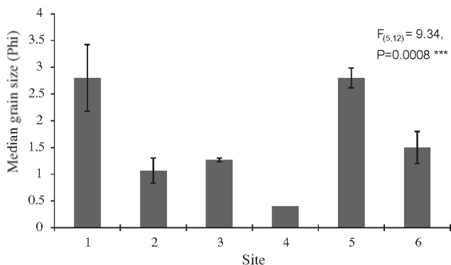
Fig. 3. Median sediment particle size ( \pm SE) of intertidal sediments at the Dar es Salaam coast, Tanzania ( \pm SE). For sample sites, see Fig. 1.
