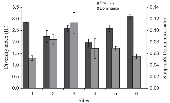
Fig. 6. Average Shannon-Wiener diversity index and Simpson's dominance index for intertidal molluscs at the Dar es Salaam coast, Tanzania ( \pm SE). For sample sites, see Fig. 1.
