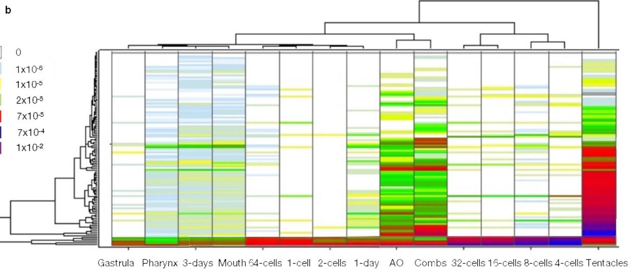
Extended Data Figure 9 | Diversity of ion channels in Pleurobrachia bachei . a , Metazoan ion channel complement. The 112 ion channels identified in the Pleurobrachia genome are classified as voltage gated (v) or other gating such as second messengers. Receptor channels (R) are ligand-gated or ionotropic (iGluR, ChRN, HTR3, GABA and CLR) and indicated in grey. Metazoan novelties indicate type of ion channels absent in the choanoflagellates, the sister group to all animals. Coloured squares show channels: (1) primarily absent in ctenophores (pink); (2) secondarily lost in sponges or placozoans (dark yellow); (3) eumetazoan (Cnidaria+Bilateria) innovations (blue); or (4) examples of expansion of certain class of channels in some animal lineages (red). All
