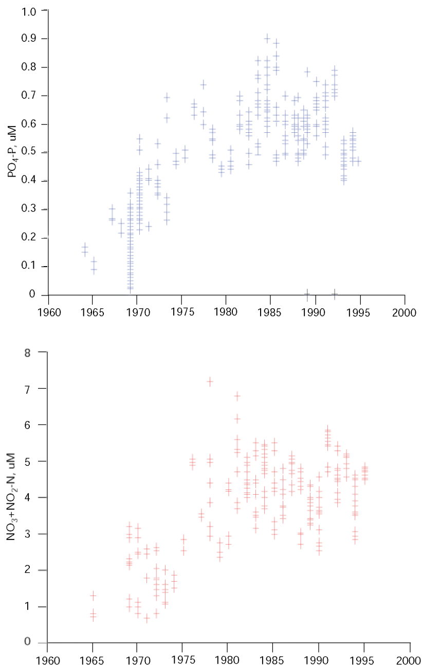
Long-term development (1964–95) of winter concentrations (mid-January to mid-April) of phosphate and nitrate and nitrate in the surface layer (0–10 m) of the open Baltic Proper (East-Gotland Basin)
