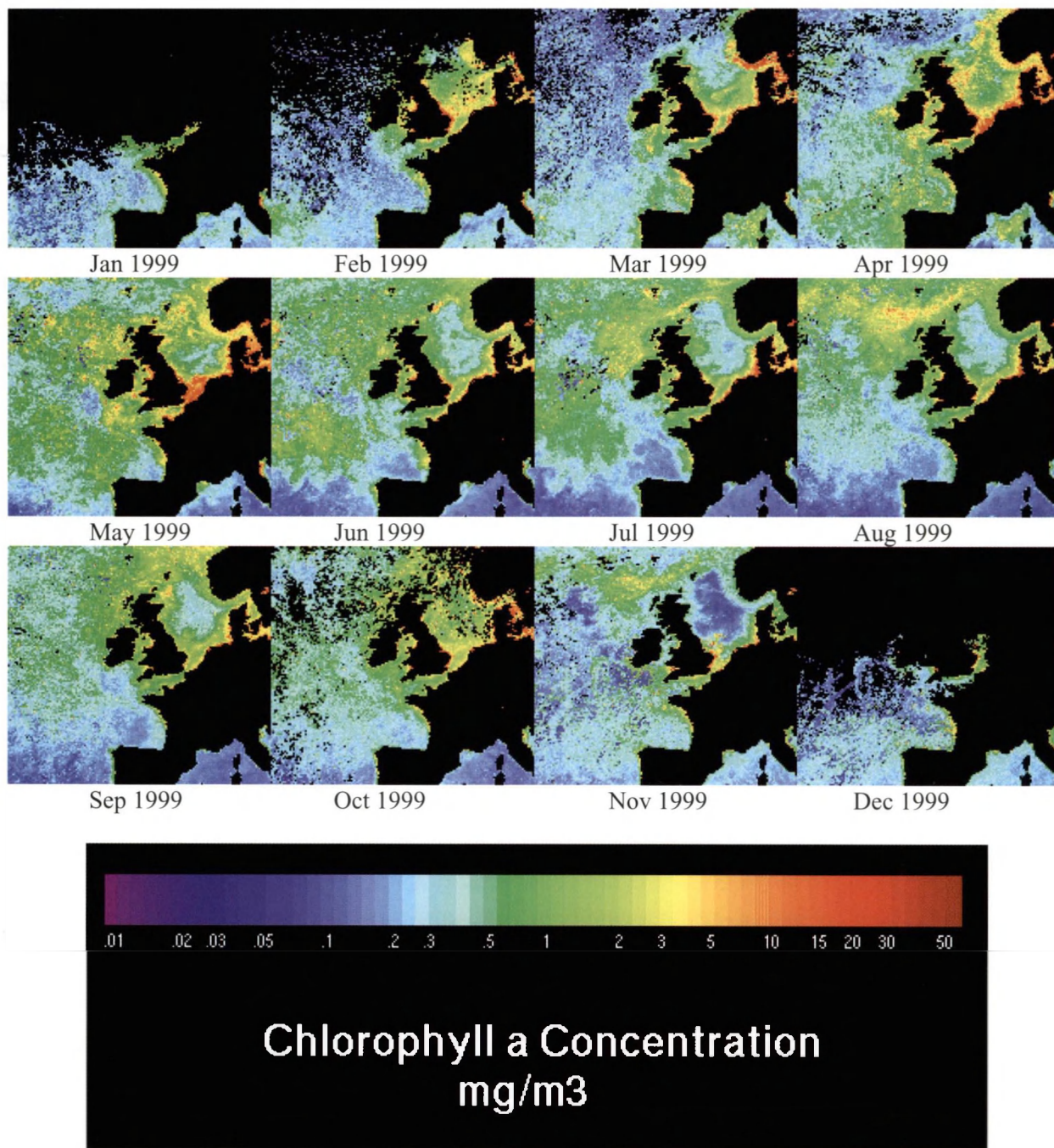
Figure 2: Bio-ecological products showing monthly monthly composites of chlorophyll a distribution in the North Sea from SeaWiFS data. Plymouth Marine Laboratory - Remote Sensing Group involvement within SEAMAR ( http://www.ieo.es/seamar/seamar.htm ).
