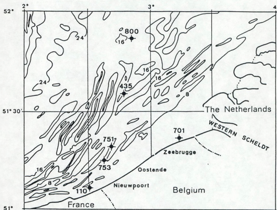
The position of the six stations in the Southern Bight of the North Sea.
