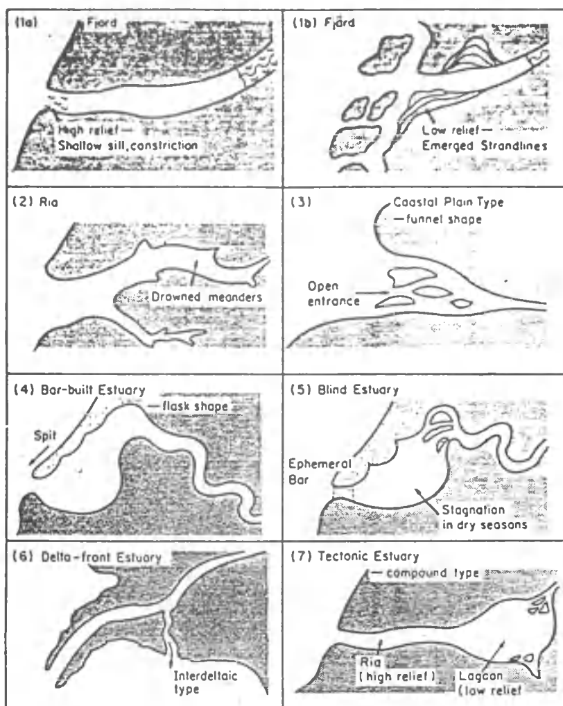
fig. 3 Basic estuarine physiographic types. Hydrodynamic characteristics are not considered here; discharge, tidal range, latitude (climate), and exposure all play important roles in modifying these examples, in addition to long-term secular processes such as tectonics and eustasy (schematic) (from Fairbridge, 1980).
