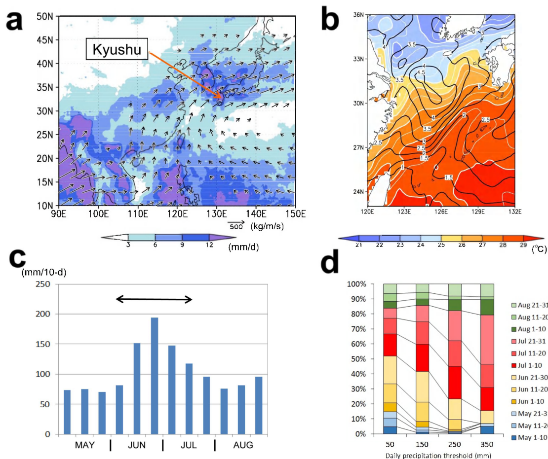
Figure 1 | Climatologies of the Baiu/Meiyu rain front and rain events in Kyushu Island. (a), July climatologies of monthly precipitation ( \text{mm d}^{-1} ; color) and vertically-integrated moisture flux ( \text{kg m}^{-1} \text{s}^{-1} ; vectors). (b), Monthly SST climatology ( ^{\circ}\text{C} ; color) for July, and climatological SST rising from June into July ( ^{\circ}\text{C} ; black lines). (c), Climatological bi-pentad precipitation (mm) over western Kyushu. The arrow indicates the climatological Baiu period. (d), Seasonality in frequency of precipitation events that occurred in western Kyushu and its dependency on daily precipitation threshold for selecting rain events as given on the lower abscissa. Total accumulated numbers of the selected events based on the individual thresholds are given on the upper abscissa. Data sources for this figure are given in Supplementary Information S1. The Grid Analysis and Display System was used for creating the maps in (a) and (b).
