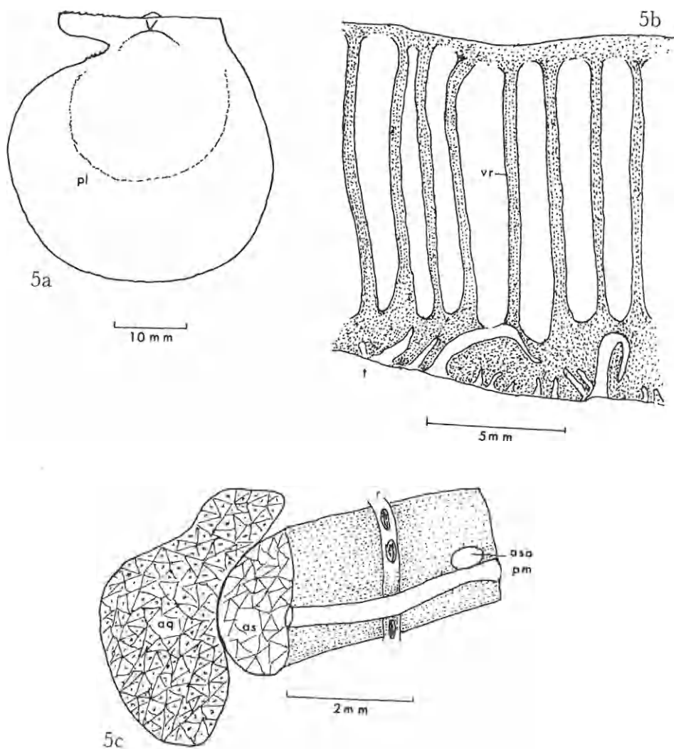
Fig. 5. Pseudohinnites levi . a, internal view of right valve; b, a section of ventral part of velum; c, adductor, postrectal muscle and abdominal sense organ.
