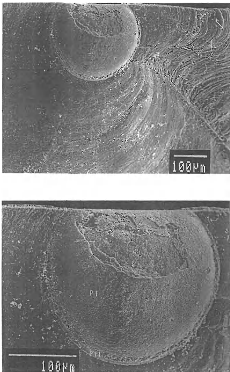
Fig. 10. Pseudohinnites levii . a (above), b (below). Micrographs of the prodissocoench of the right valve of the 'Siboga' specimen.
