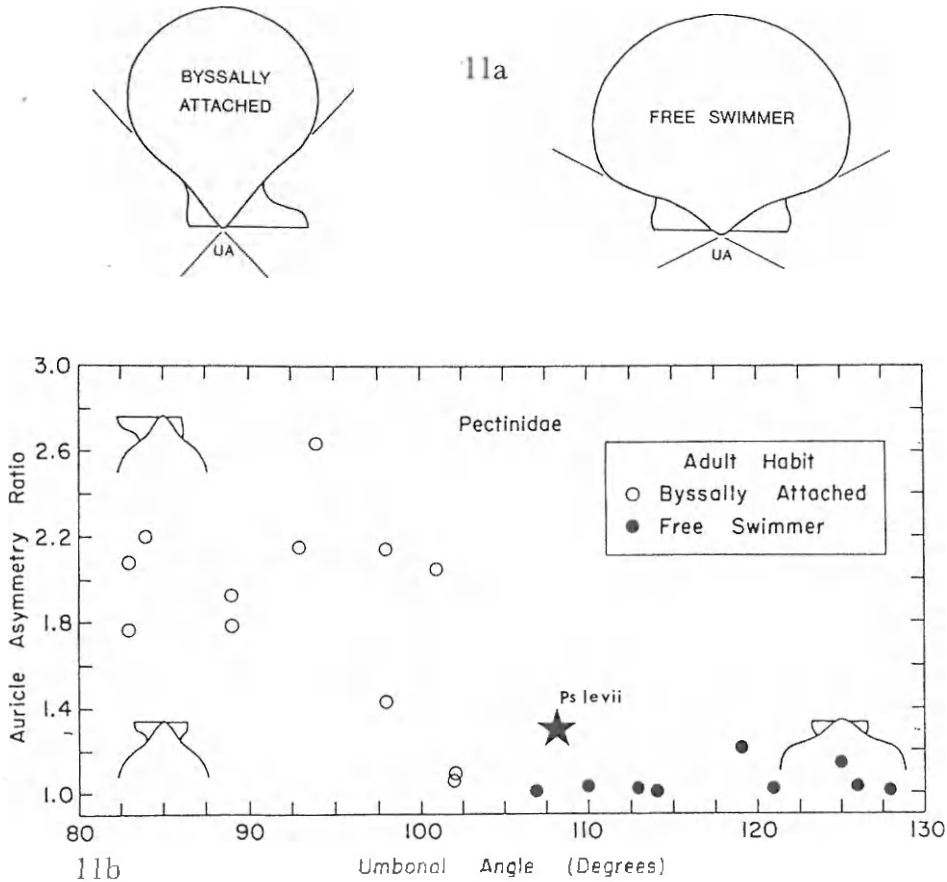
Fig. 11. a, Relation of swimming capacity and outline of valve in Pectinoidea; b, graph of auricle asymmetry versus umbonal angle for byssally attached and free-swimming members of Pectinoidea. Auricle asymmetry is the ratio between anterior and posterior auricle lengths. Modified from Stanley (1970).
