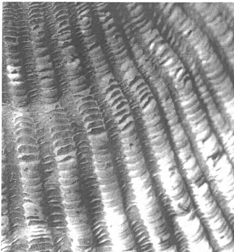
Fig. 3. Pseudohinnites levii Sculpture of the central part of left valve. x about 9.
