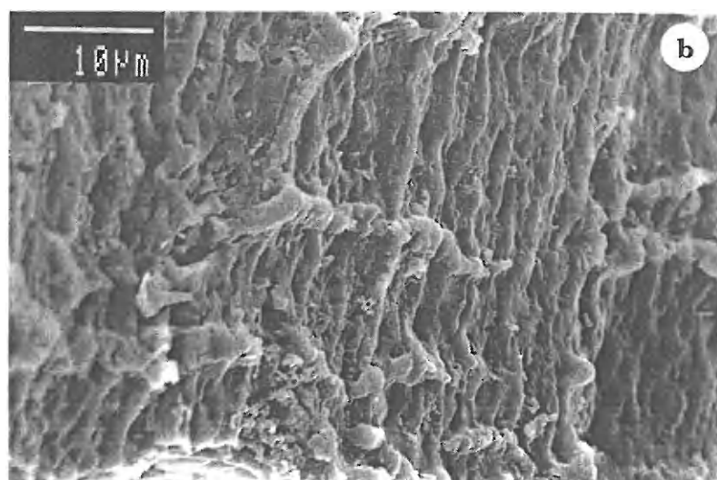
Fig. 4. Pseudohinnites levi . a, micrograph of prismatic layer of right valve; b, micrograph of microsculpture of left valve. - Both micrographs were taken near the prodissocoach. The specimen originates from 'Siboga' expedition, stn 300 (Dijkstra, 1990).
