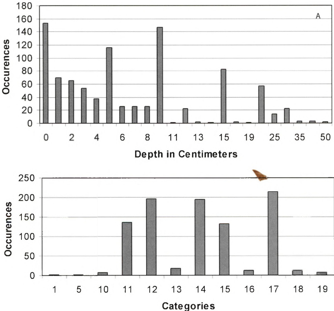
Figure 7.8. Frequency distributions of penetrability (a) and SPOT values (b).
