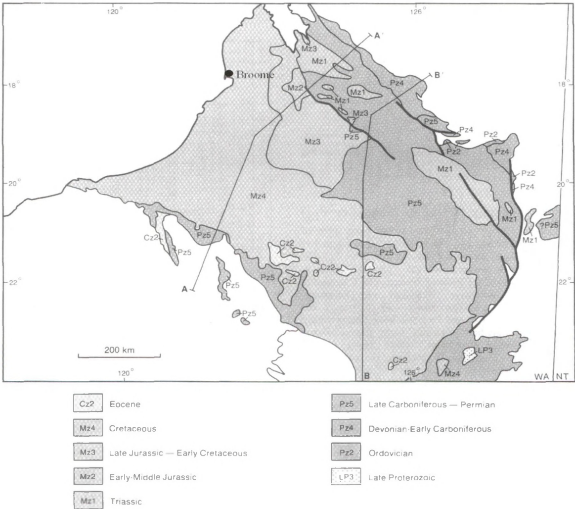
Figure 6.1. Map of Eighty-mile Beach Showing the Onshore Canning Basin (Bureau of Mineral Resources, Geology and Geophysics).
