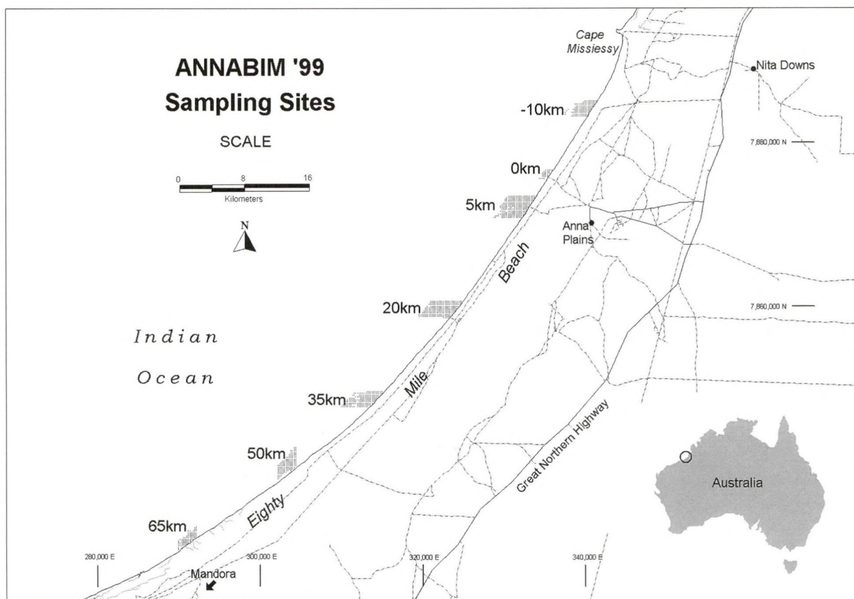
Figure 7.3. Sampling locations along Eighty-mile Beach.
