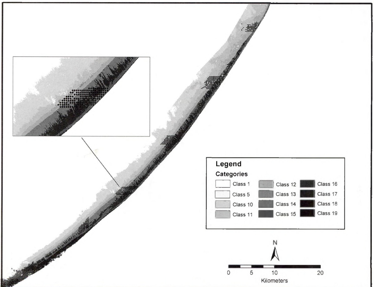
Figure 7.7. Spectral categories of Eighty-mile Beach.
