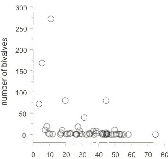
Figure 9.9. The relationship between the total number of individuals of bivalves and the relative amount (%) of sediment in the 0.063 - 0.125 mm size class. Each point is a replicate sample from each of one of the 6 blocks (beaches).
