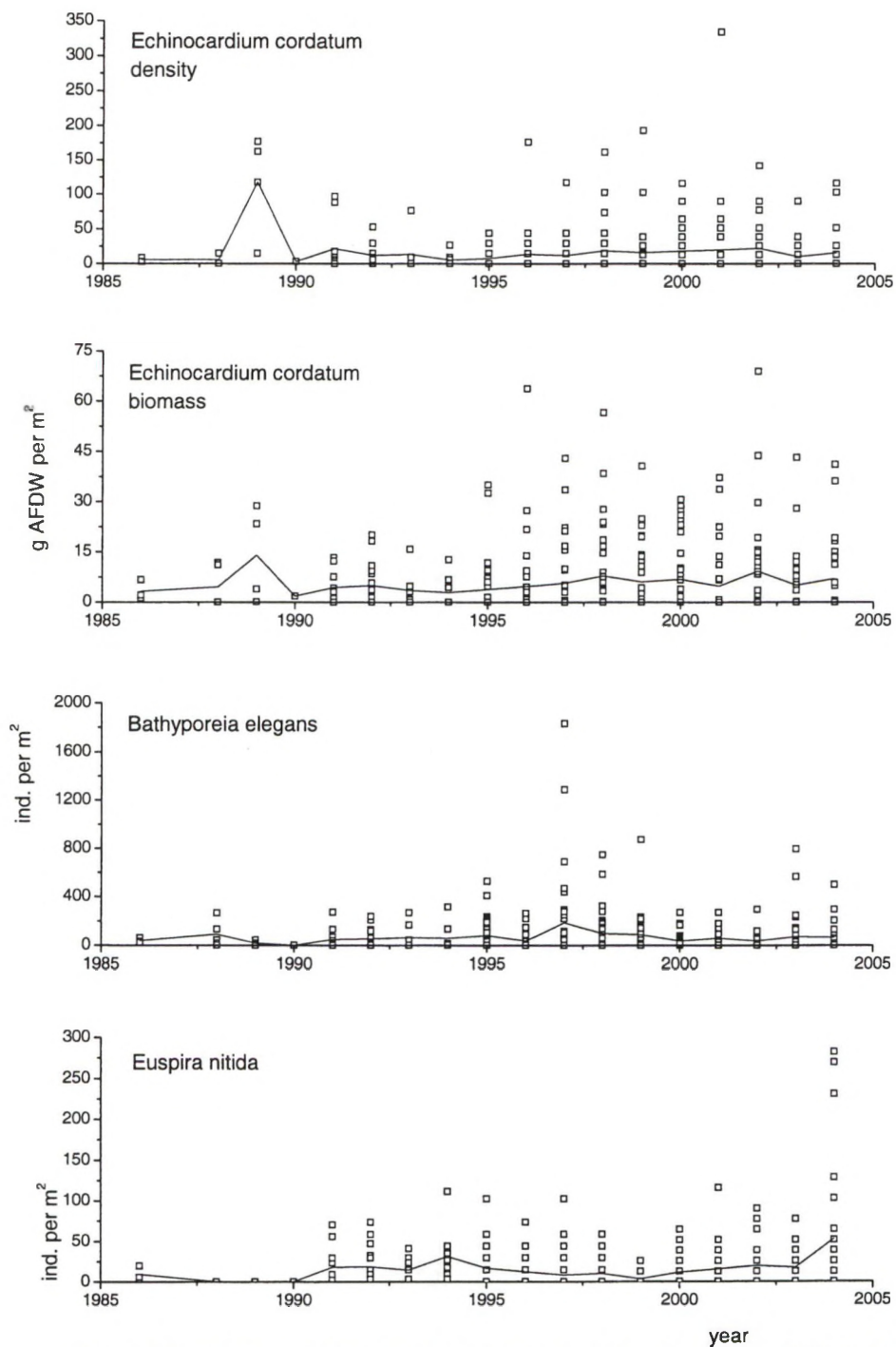
Fig. 17a: Densities (and biomass of E. cordatum ) of 3 species in the offshore area (1986-2004).
