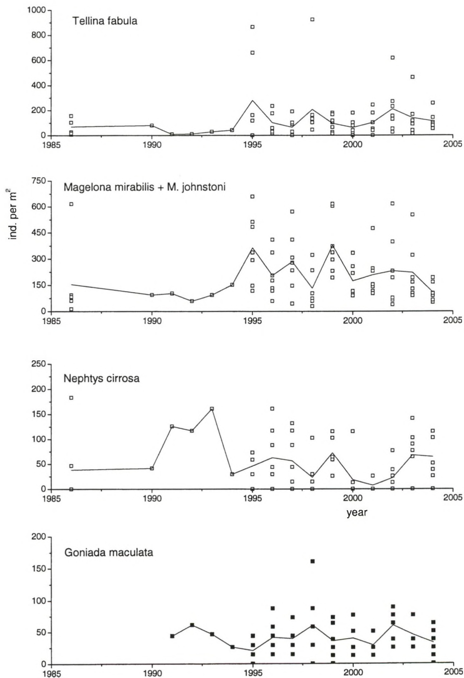
Fig. 15b: Densities of 4 species at the Dogger Bank (1986-2004)
