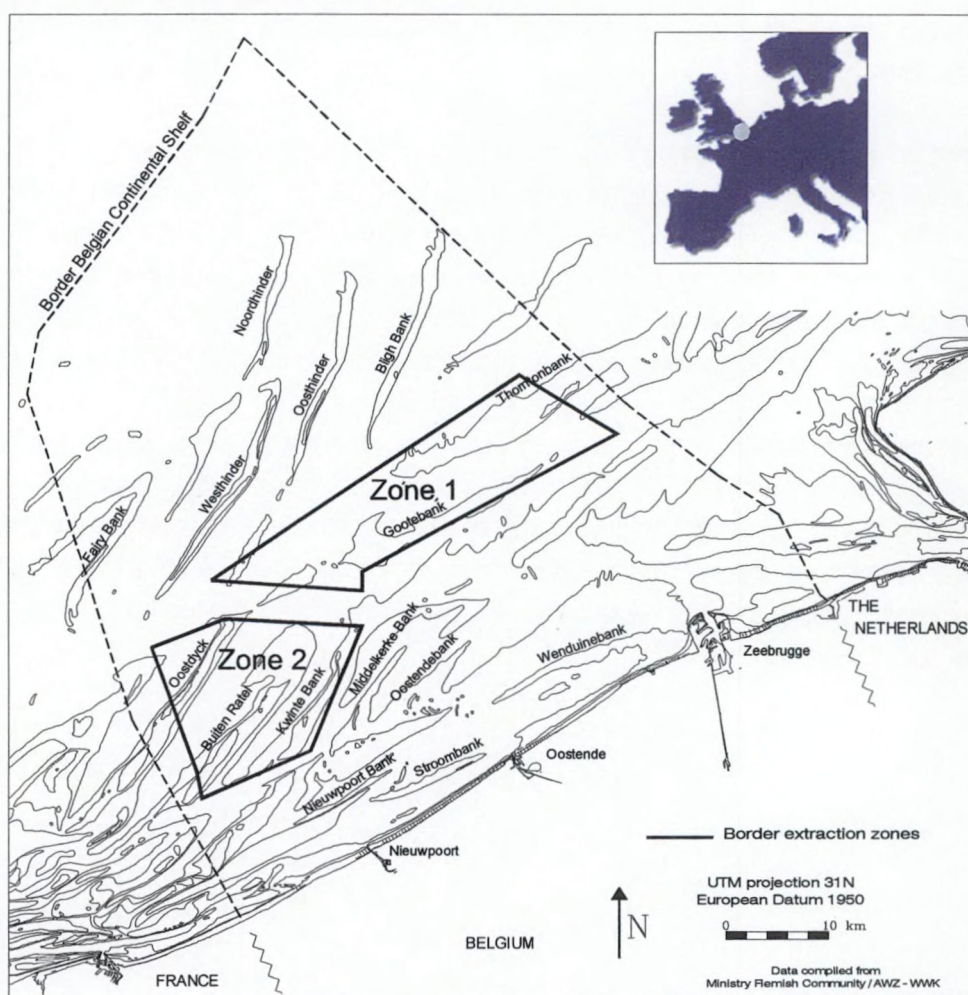
Figure 1. Bathymetry of the BCS with an indication of the present areas of aggregate extraction (data from the Ministry of the Flemish Community, Waterways and Coastal Section).
