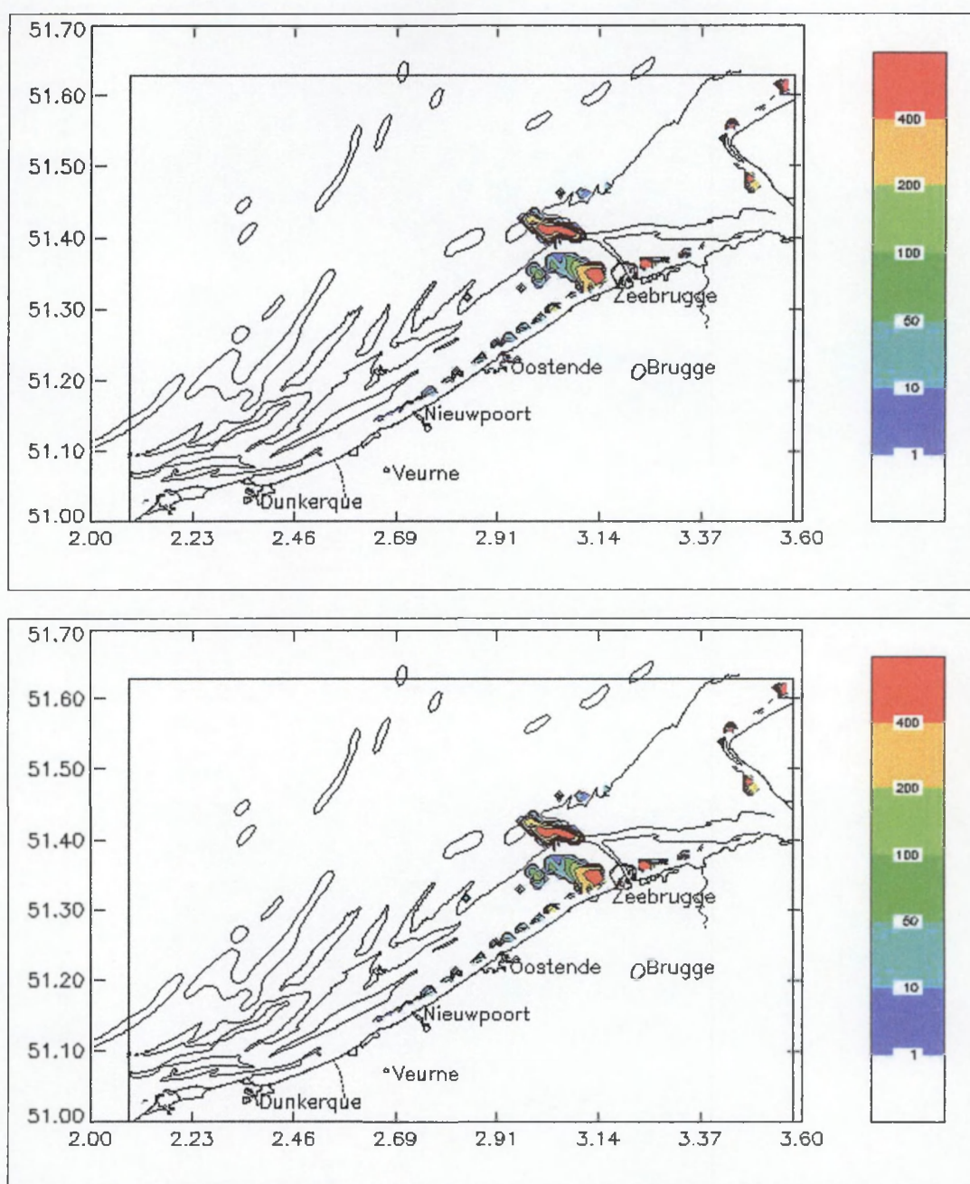
Figure 10. Mud deposition (in \text{kg/m}^2 ) in the active layers according to a model simulation (mu-STM) where the SPM concentration boundary condition is based on measurement data and where initially mud is present in the parent bed. (a) spring tide and (b) neap tide. Assuming a bulk density of the mud of 1300 \text{ kg/m}^3 , 100 \text{ kg/m}^2 corresponds to a mud layer of \pm 8 \text{ cm} .
