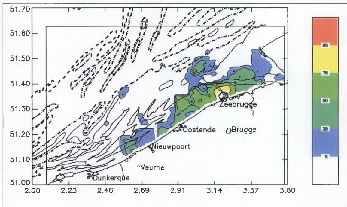
Figure 7. The map shows the mu-STM model boundaries, the 10, 20 and 30 m depth lines (MSL) and the mud (<63 \mu m) content (% weight) of the surficial sediments. The mud content is calculated from a distance-weighted average of field data in a diameter of 3.75 km (i.e. 5 times the grid distance) and is used as input for the numerical model.
