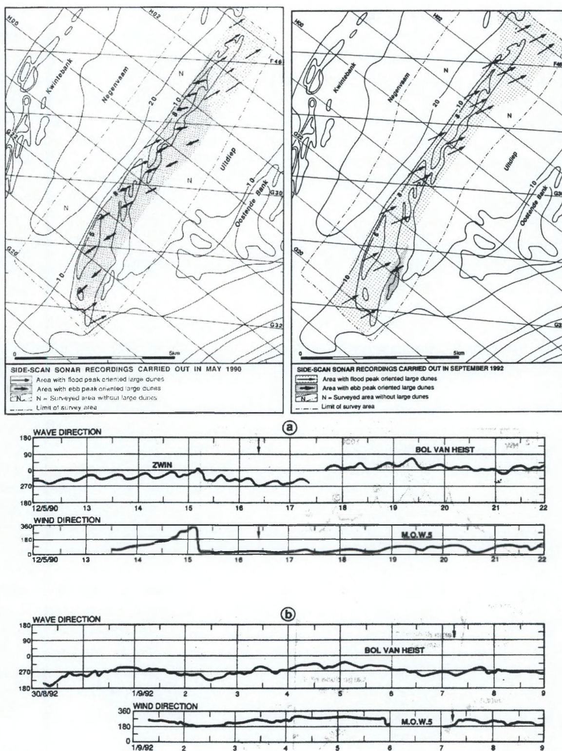
Figure 14. Asymmetry of large dunes and wave and wind direction of the period prior to the side-scan sonar recordings (LANCKNEUS and DE MOOR (1994)). Wave directions recorded with directional wave buoys and wind direction data from the measuring pile MOW5 for the periods 12-22 May 1990 (a) and 30 August – 9 September 1992 (b). The arrows indicate the days of the bathymetric surveys.
