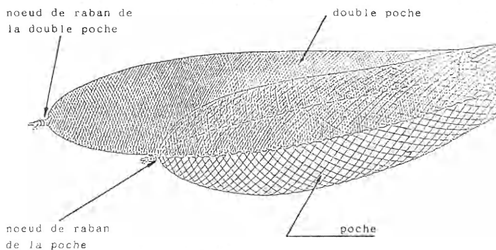
Figure 2 - Double poche partielle
