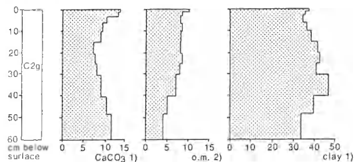
Fig. 2. Changes in \text{CaCO}_3 content with depth in a profile of a pool with a rapid accretion. For explanation of 1), 2) and 3) see Fig. 1. (Van der Sluys, 1970)
