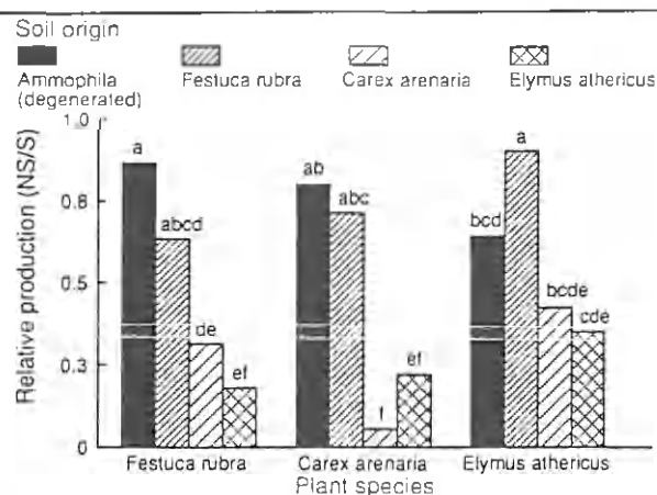
Fig. 14: Production of total biomass of Festuca rubra ssp. arenaria , Carex arenaria and Elymus athericus in unsterilized soil relative to that in sterilized soil. The soils originate from sites with pure stands of degenerated Ammophila arenaria , F. rubra ssp. arenaria , C. arenaria and E. athericus . METHODS. See Table 2. The relative productions were analysed by analysis of variance with factors being soil origin and plant species. As there was two-way interaction, Tukey's multiple comparison was applied to compare means of treatments and significant differences ( P < 0.05 ) are indicated by different letters.
