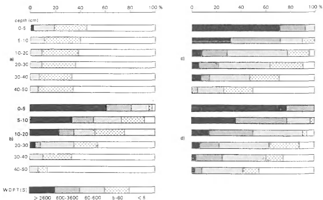
Fig. 11: Relative frequency of the WDPT of samples at six depths in dune sands with a vegetation of a) marram-grass, b) grey hair-grass, c) heather and d) hawthorn. (DEKKER & JUNGRIUS, 1990).
