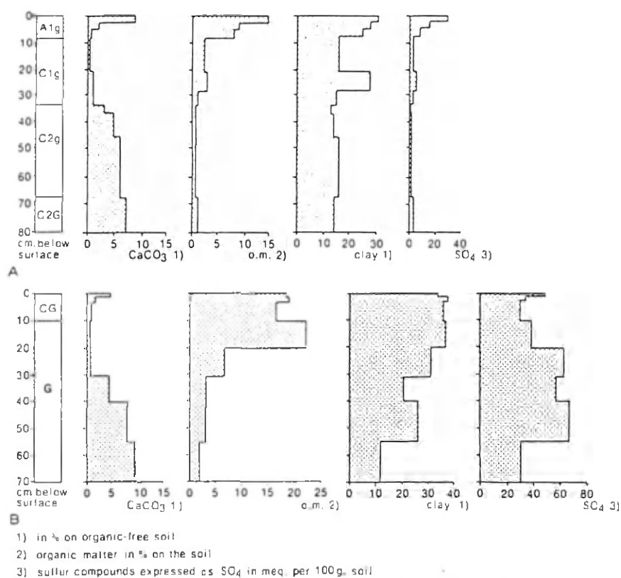
Fig. 1. Changes in \text{CaCO}_3 content with depth in profiles of a salt marsh with a slow accretion. A = levee; B = pool. (Van der Sluys, 1970)
