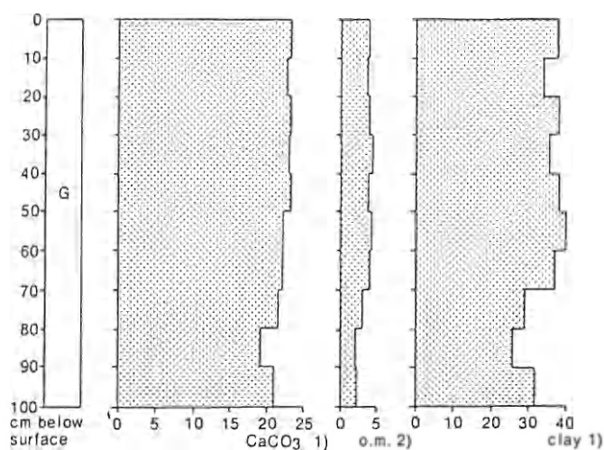
Fig. 3. \text{CaCO}_3 profile in a bare mudflat. For explanation of 1) and 2) see Fig. 1. (Van der Sluys, 1970)
