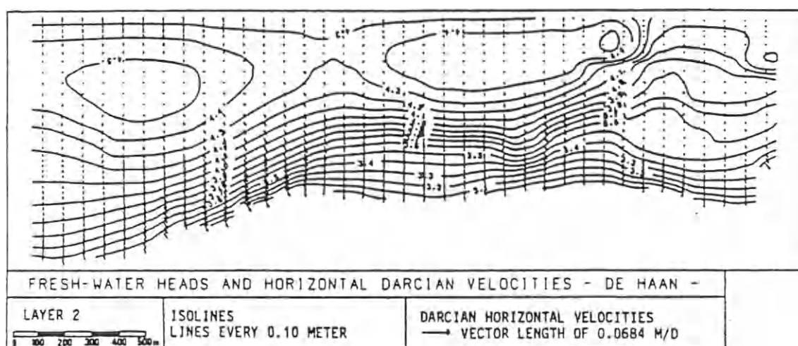
Groundwater flow in semi-confined layer B
