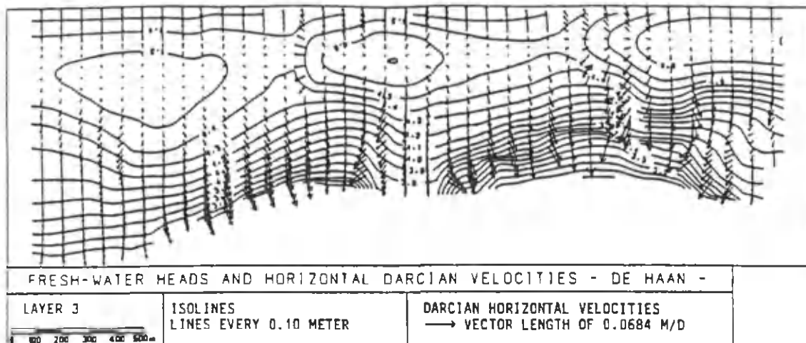
Groundwater flow in phreatic layer A
