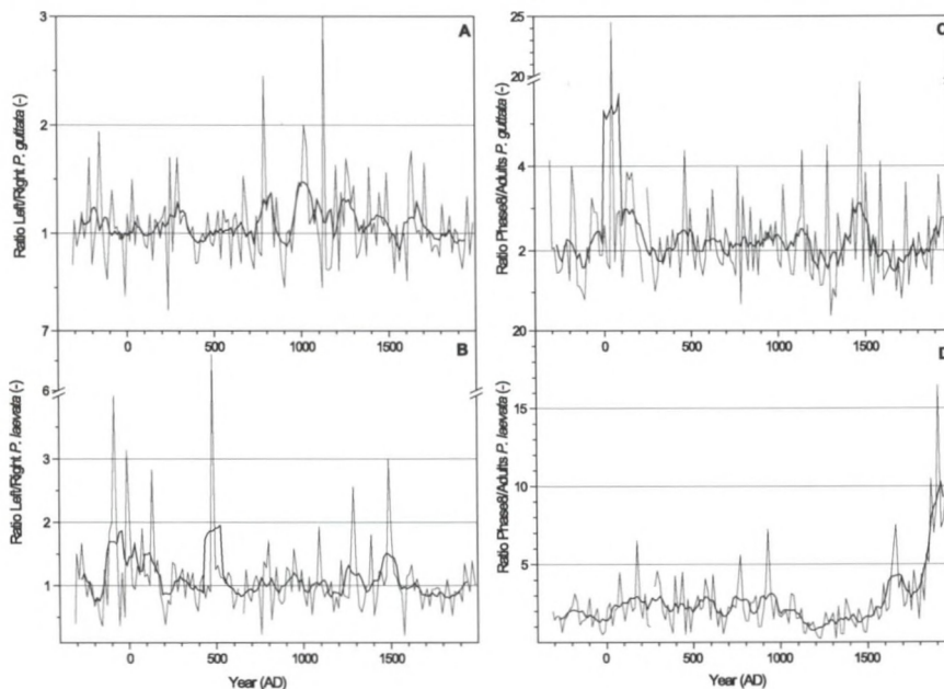
Fig. 3.5.2 Relative shell-deposition rates of ostracods ( \text{n m}^{-2} \text{y}^{-1} ) in the German Bight between -312 and 1996 AD as derived from a pistoncore taken on June 4, 1996. A. Ratio of left and right shell-halves of Palmoconcha guttata (-). B. Ratio of left and right shell-halves of Palmoconcha laevata (-). C. Ratio of phase8 and adult specimen of Palmoconcha guttata (-). D. Ratio of phase8 and adult specimen of Palmoconcha laevata (-).
