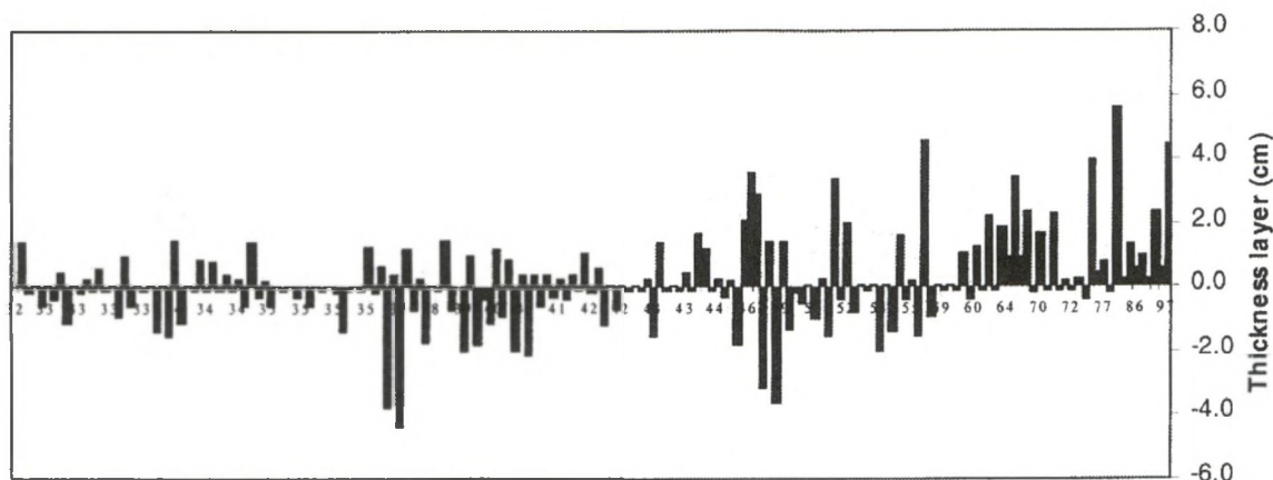
Fig. 4.5.2 Lithology of vibrocore V7D taken in the former Vlieter channel on June 20, 1997. The positive values refer to the thickness of the sandy layers over depth (from left to right is from bottom to top, viz. from May 1932 to June 1997), the negative values to those of the non-sandy layers (mainly containing clay, but also clayey sand or sandy clay).
