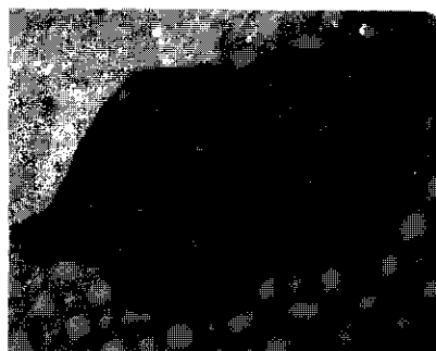
Fig. 6.1d. Scars from former shell damage of B. undatum from the North Sea.
