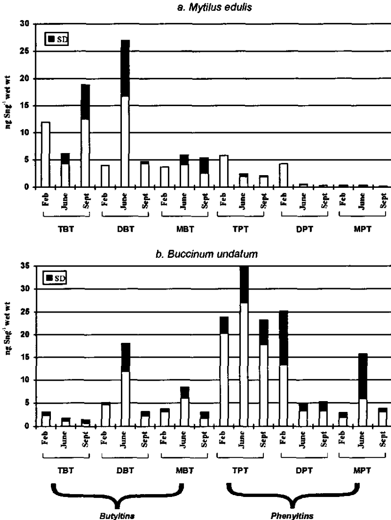
Figure 5.2 a,b. Average ( \pm SD) whole body organotin concentrations ( \text{Sn ng g}^{-1} wet weight) in M. edulis (a) or for all specimens of B. undatum (b) per month. (For values < \text{DL} , half of the reported DL was used.)
