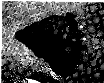
Fig. 6.1a. Severe outer lip damage in B. undatum from the North Sea.
