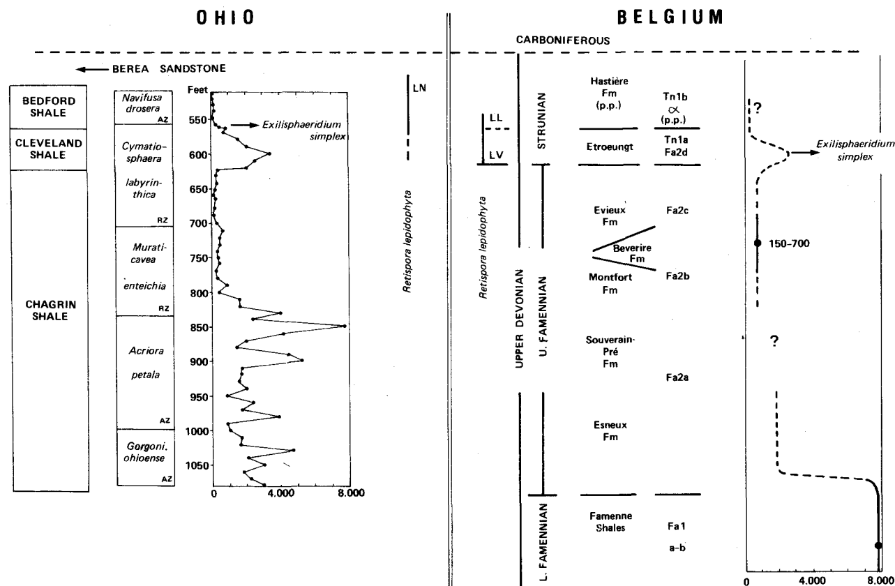
Figure 4. - Comparison of acritarch abundance profiles for the Upper Famennian-Strunian of Ohio, U.S.A. (after Wicander, 1975) and Famennian-Strunian of Belgium (profile based on Streel in Becker, Bless, Streel & Thorez, 1974, on Rouhart in Vanguestaine et al. , 1983, and on unpublished data).
