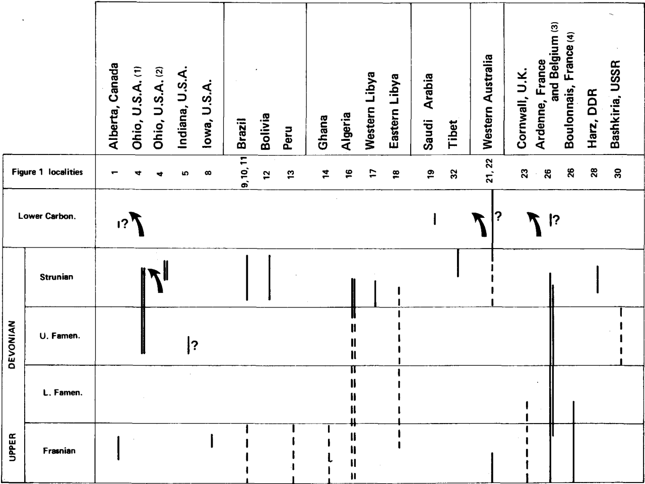
Figure 3. - Approximate stratigraphic position of sequences investigated on their acritarch contents in the Upper Devonian and Lower Carboniferous. Single line : spot samples, reduced or incompletely studied interval (no zonation proposed); double line : sequence studied in detail (zonation proposed); dashed line or question mark : poorly dated; full line : dated; arrow : possible reworking.
