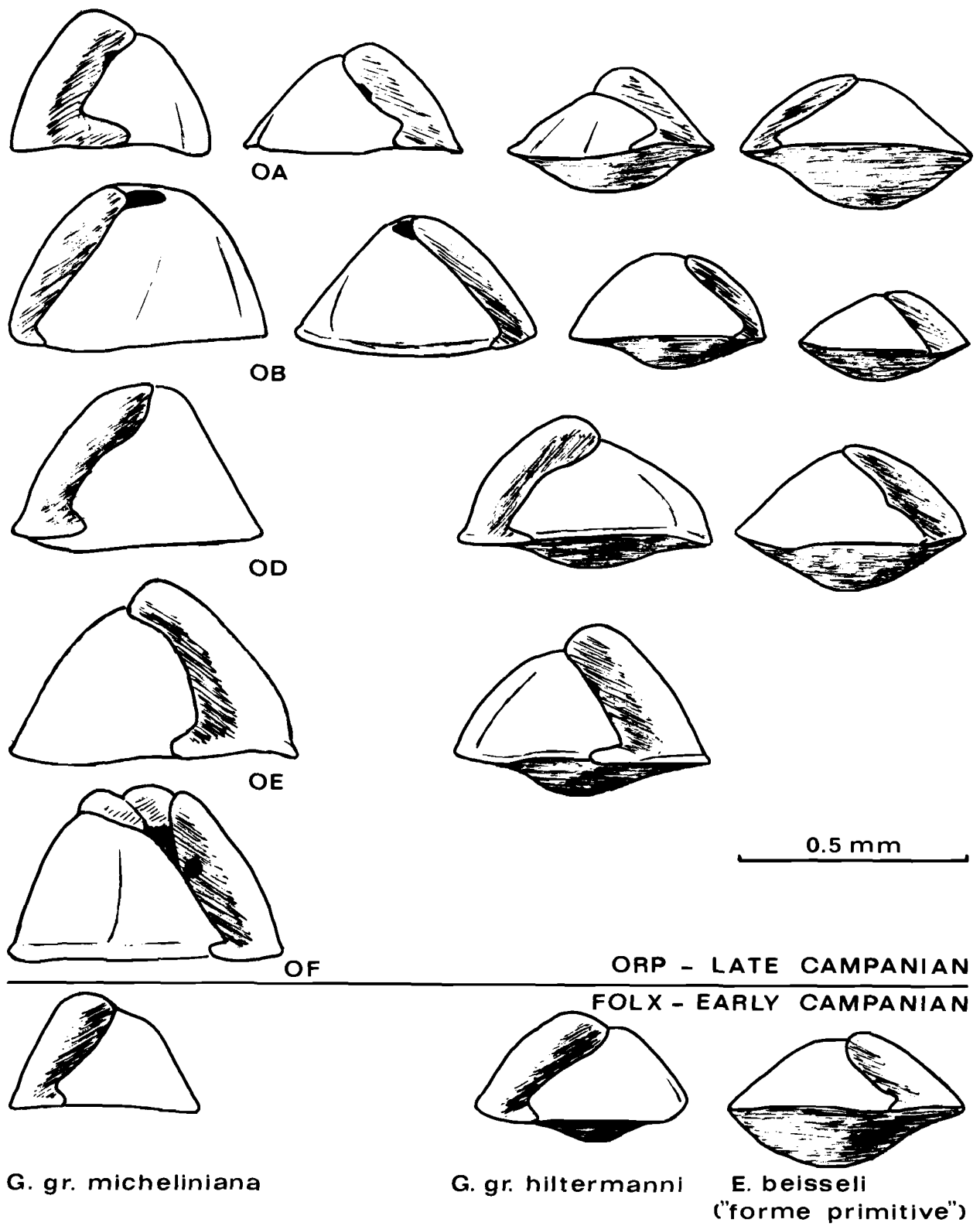
Fig.7.- Co-occurrence of the benthic forams Globorotalites gr. micheliniana (ORBIGNY), G. gr. hiltermanni KAEVER and « Eponides beisseli , forme primitive» (HOFKER, 1956. 1963, 1966) in the (middle-late) early Campanian of Folx-les-Caves and the late Campanian of Orp-le-Petit. Only the slightly schematized lateral views are shown. In the MAL area (Hofker, 1966; Robaszynski et al. , 1985), the Hautes Fagnes area (Bless et al. , 1990) and the Mons basin (Robaszynski & Christensen,
