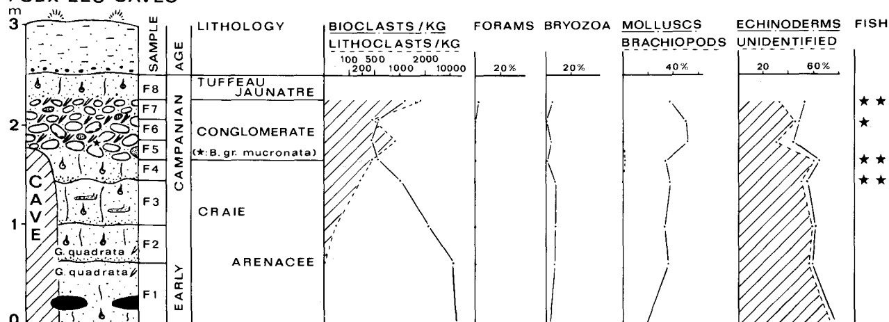
Fig.2.- Lithological section of the outcrop Folx-les-Caves (entry to cave of former subterranean chalk/flint quarry; flint nodules shown in the figure in subunit F1 do not occur in the outcrop itself but c. 2 m into the cave) with frequency profiles
