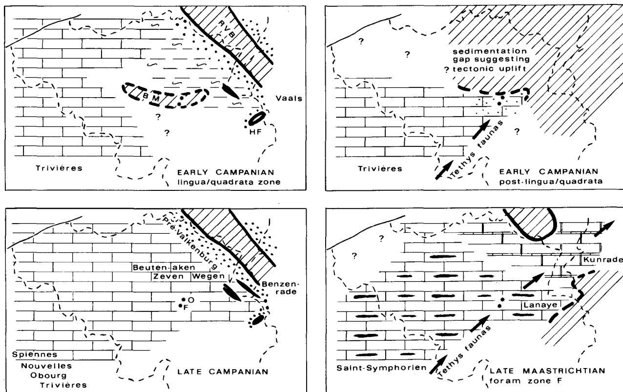
Fig.9.- Palaeogeographic evolution of Belgium and the southern Netherlands during the Campanian and Maastrichtian. Non-depositional areas are indicated by diagonal
