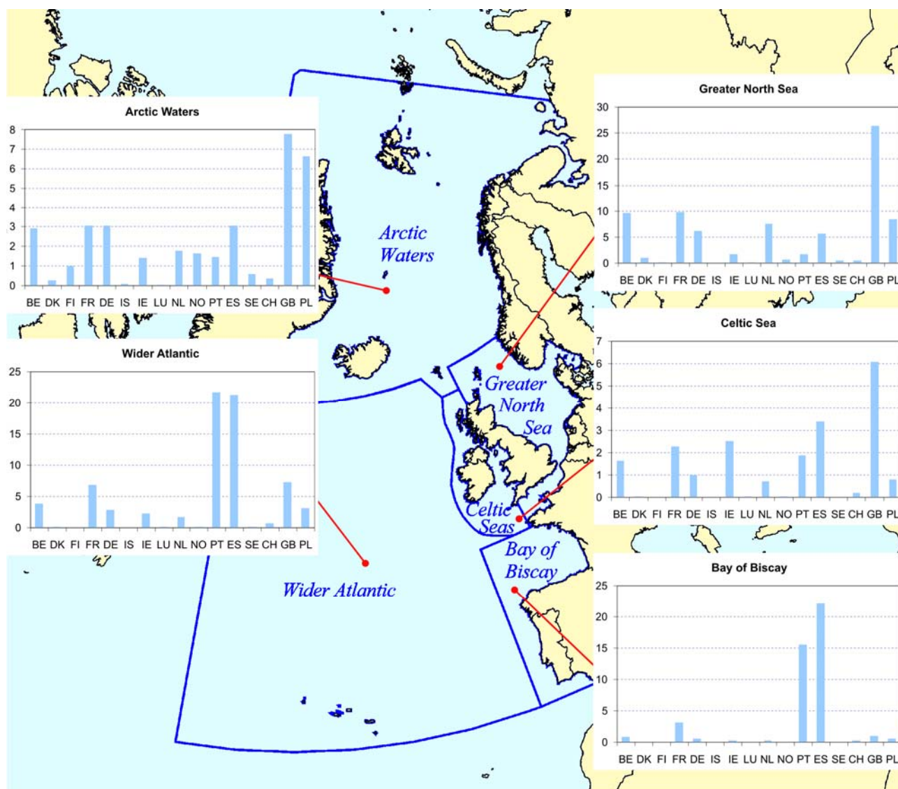
Figure 6.14: Contribution of individual countries to the modelled annual deposition of lead to the OSPAR Regions for 2006. Units are in t/yr.
