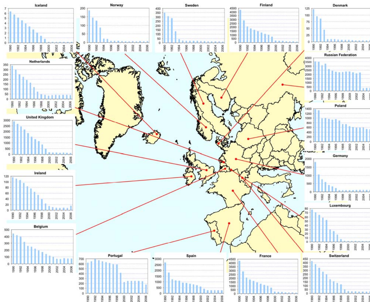
Figure A2.1: Atmospheric emission of lead in tonnes per year.
