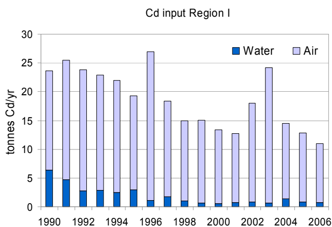
Figure A10.3: Total cadmium input to Region I by direct discharges and riverine inputs (RID) and EMEP modelled atmospheric deposition (Note: RID data only for Norway).
