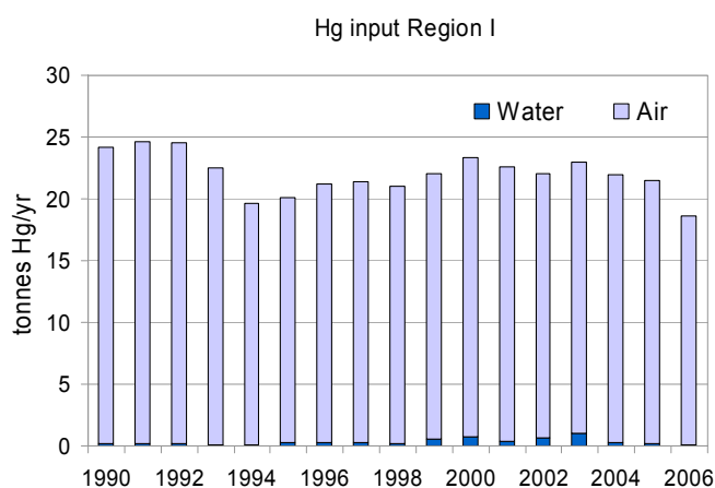
Figure A10.4: Total mercury input to Region I by direct discharges and riverine inputs (RID) and EMEP modelled atmospheric deposition.
