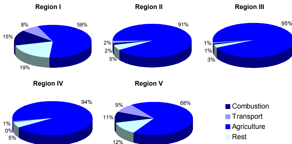
Figure 6.11: Contribution of sectors to the annual deposition of reduced nitrogen to the OSPAR Regions in 2006 (Sectors as for Figure 6.3).
