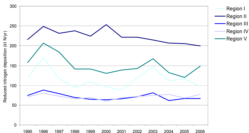
Figure 6.9: Time series of EMEP modelled annual deposition of reduced nitrogen to the OSPAR Regions. Units in kt N/yr.
