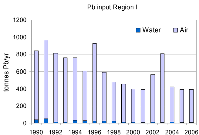
Figure A10.2: Total lead input to Region I by direct discharges and riverine inputs (RID) and EMEP modelled atmospheric deposition (Note: RID data only for Norway).
