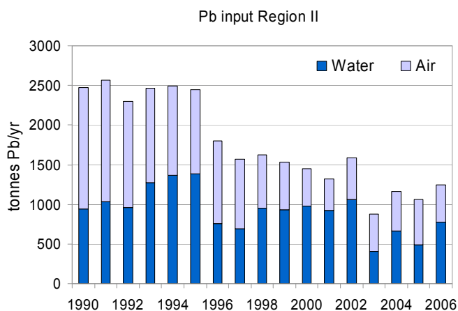
Figure A10.6: Total lead input to Region II by direct discharges and riverine inputs (RID) and EMEP modelled atmospheric deposition.
