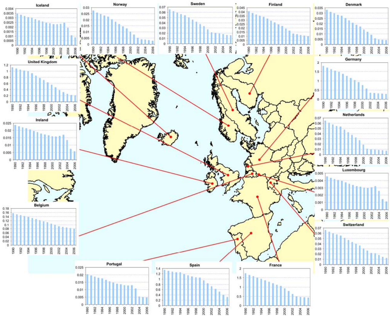
Figure A2.5: Atmospheric emission of PCB-153 in tonnes per year.
