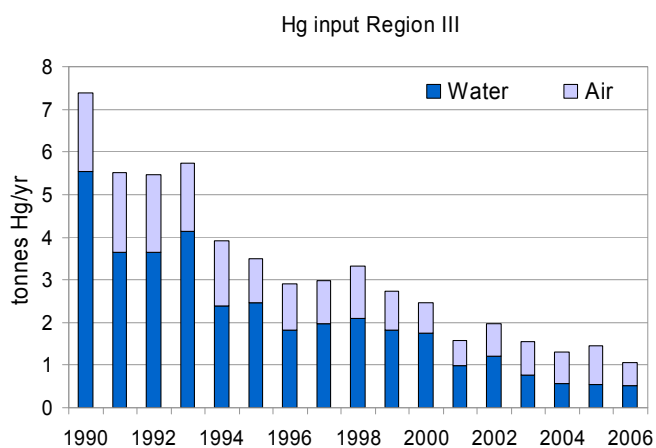
Figure A10.12: Total mercury inputs to Region III by direct discharges and riverine inputs (RID) and EMEP modelled atmospheric deposition.
