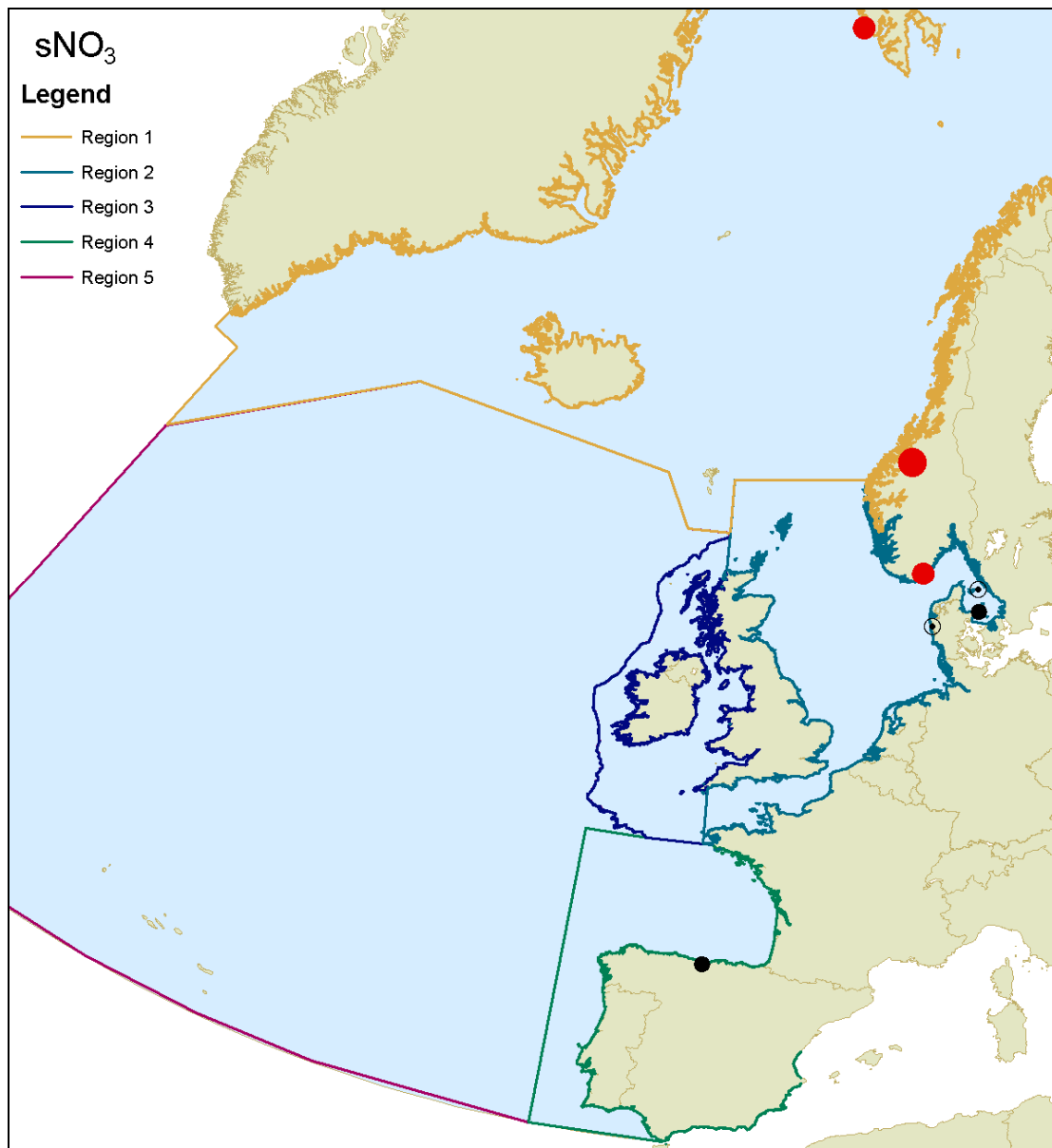
Figure 5.3: Geographical distribution of results from the trend analysis for sNO 3 in air. Explanation as for Figure 5.1
