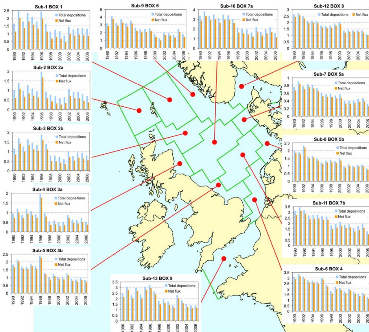
Figure 6.22: Time series (1990 – 2006) of modelled total and net deposition fluxes of cadmium to the 13 sub-areas of the Greater North Sea; units are in t/yr.
