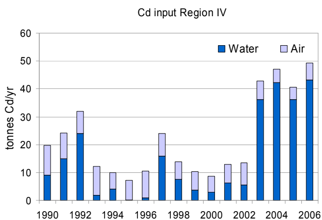
Figure A10.15: Total cadmium inputs to Region IV by direct discharges and riverine inputs (RID) and EMEP modelled atmospheric deposition (Note: RID data for Spain and Portugal only).
