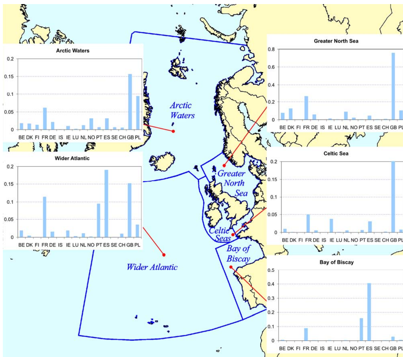
Figure 6.24: Contribution of individual countries to the annual depositions of mercury to the OSPAR Regions for 2006; units are in t/yr.
