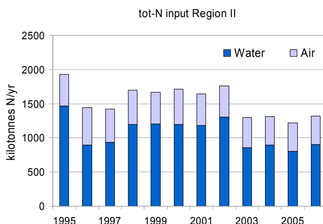
Figure A10.5: Total nitrogen load into Region II by direct discharges and riverine inputs (RID) and the total EMEP modelled atmospheric deposition. Units are in kt N/yr.
