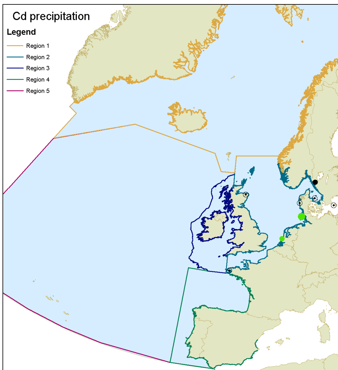
Figure 4.4: Geographical distribution of results from trend analysis for cadmium in precipitation. See Figure 4.1 for details. In this graph only small and medium size dots are depicted.
