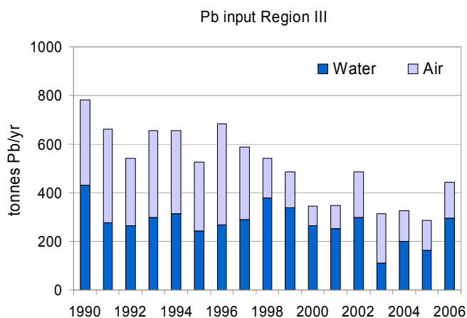
Figure A10.10: Total lead inputs to Region III by direct discharges and riverine inputs (RID) and EMEP modelled atmospheric deposition.
