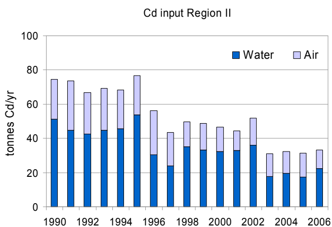
Figure A10.7: Total cadmium input to Region II by direct discharges and riverine inputs (RID) and EMEP modelled atmospheric deposition.
