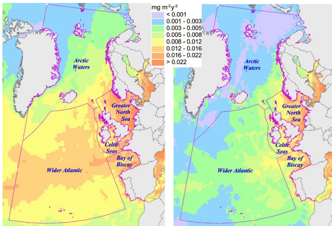
Figure 6.18: Total (left panel) and net (right panel) deposition fluxes for cadmium to the OSPAR Regions in 2006; units are in \text{mg/m}^2 per year.
