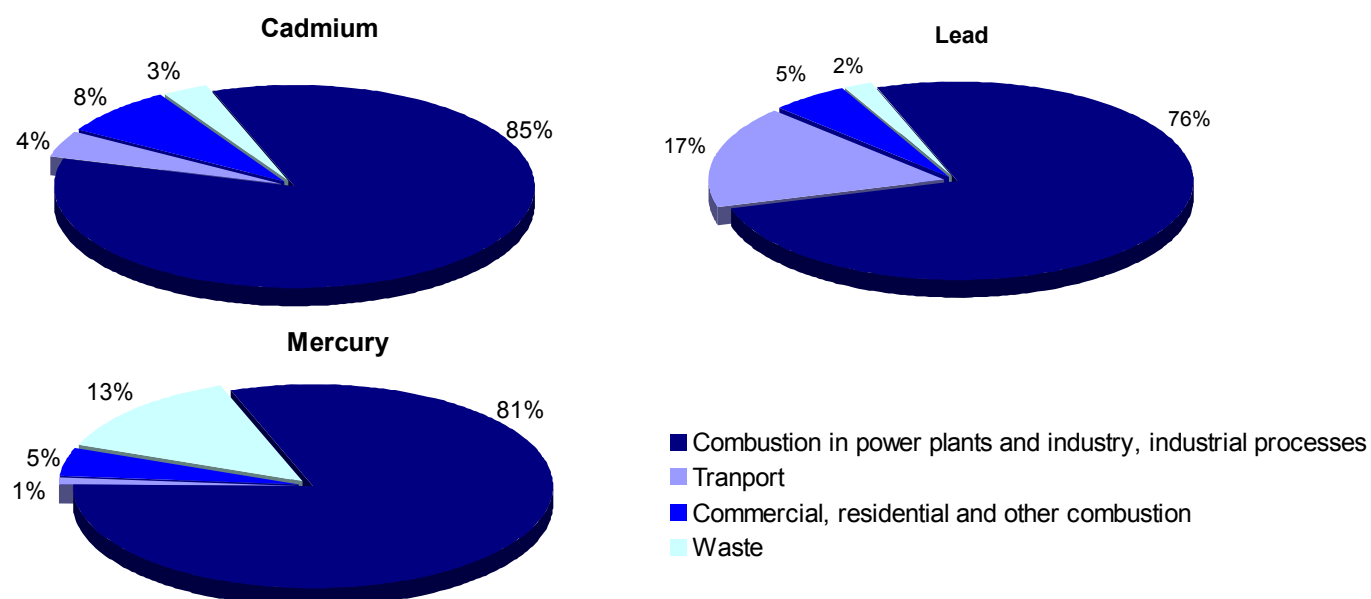
Figure 0.3: Relative contribution of different emission source categories to atmospheric deposition of cadmium, mercury and lead to the OSPAR area in 2005.
