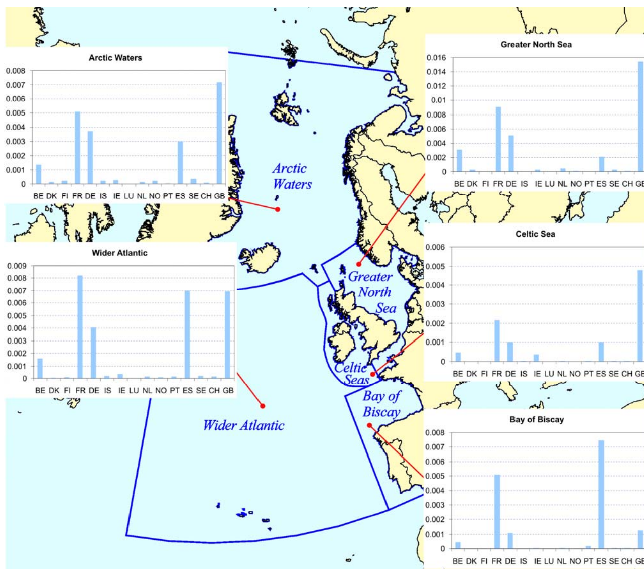
Figure 6.32: Contribution of individual countries to the modelled annual deposition of PCB-153 to the OSPAR Regions for 2006; units are in t/yr.
