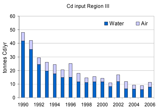
Figure A10.11: Total cadmium inputs to Region III by direct discharges and riverine inputs (RID) and EMEP modelled atmospheric deposition.
