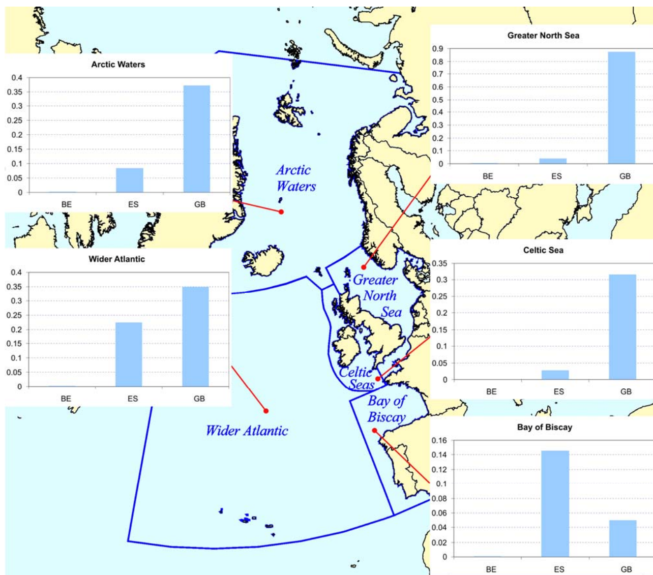
Figure 6.29: Contribution of individual countries to the annual deposition of lindane to the OSPAR Regions for 2006, based on available data; units are in t/yr.
