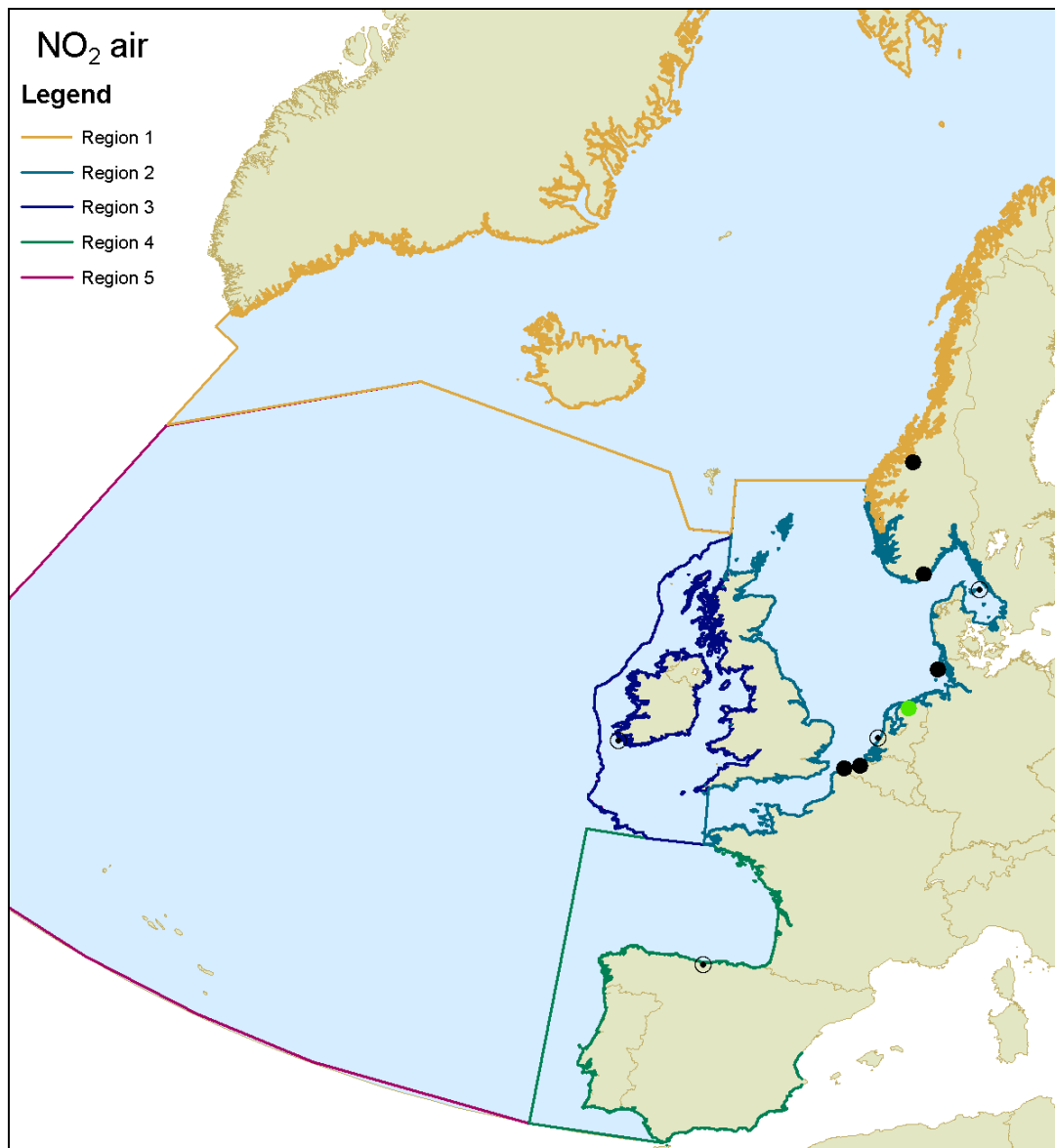
Figure 5.1: Geographical distribution of results from the trend analysis for nitrogen dioxide in air. Green dots indicate declining trends, red dots upward trends and black dots indicate no trends above the 90% significance level. A black circle around the dots indicates that the period 1998 – 2006 is not fully covered. There are 3 sizes for the dots: small size: the slope is less than 10%, medium size: the slope is in between 10% and 20% and large size: the slope is above 20%. In this graph only small size dots are depicted.
