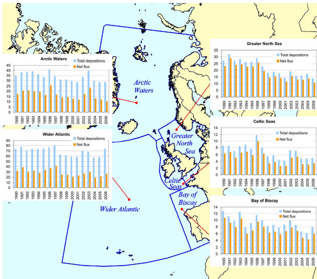
Figure 6.21: Time series (1990 – 2006) of modelled total and net deposition fluxes of cadmium to the OSPAR Regions; units are in t/yr.
