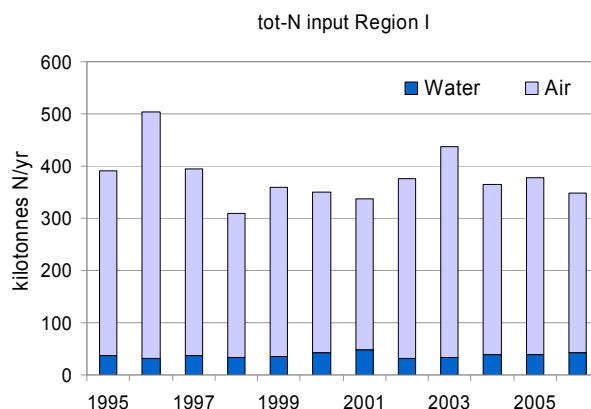
Figure A10.1: Total nitrogen inputs to Region I by direct discharges and riverine inputs (RID) and the total EMEP modelled atmospheric deposition (Note: RID data only for Norway).
