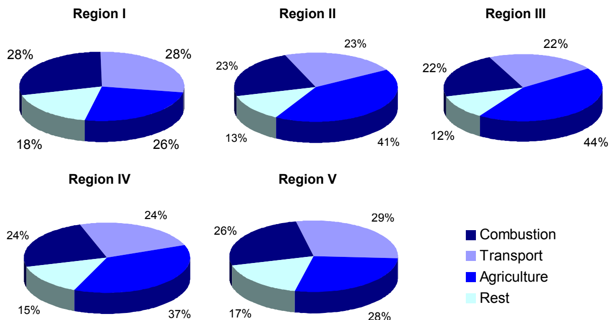
Figure 0.8: Main emission sources (as defined by the EMEP Selected Nomenclature for reporting of Air Pollutants (SNAP)) contributing to total nitrogen deposition to the OSPAR Regions in 2006. “Combustion” comprises combustion from stationary sources relating to the energy and transformation industries (SNAP 1), non-industrial combustion plants (SNAP 2) and manufacturing industries (SNAP 3). “Transport” comprises road transport (SNAP 7) and other mobile sources and machinery (SNAP 8) (including emissions from shipping). “Agriculture” refers to SNAP emission category 10. “Rest” refers to remaining SNAP emission categories.
