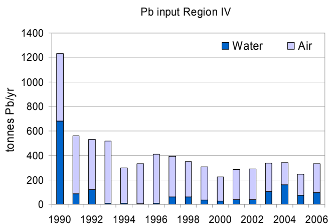
Figure A10.14: Total lead inputs to Region IV by direct discharges and riverine inputs (RID) and EMEP modelled atmospheric deposition (Note: RID data for Spain and Portugal only).
