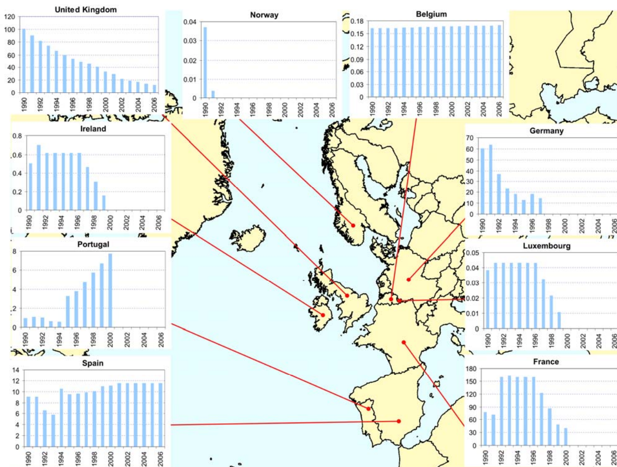
Figure A2.4: Atmospheric emissions of lindane in tonnes per year.
