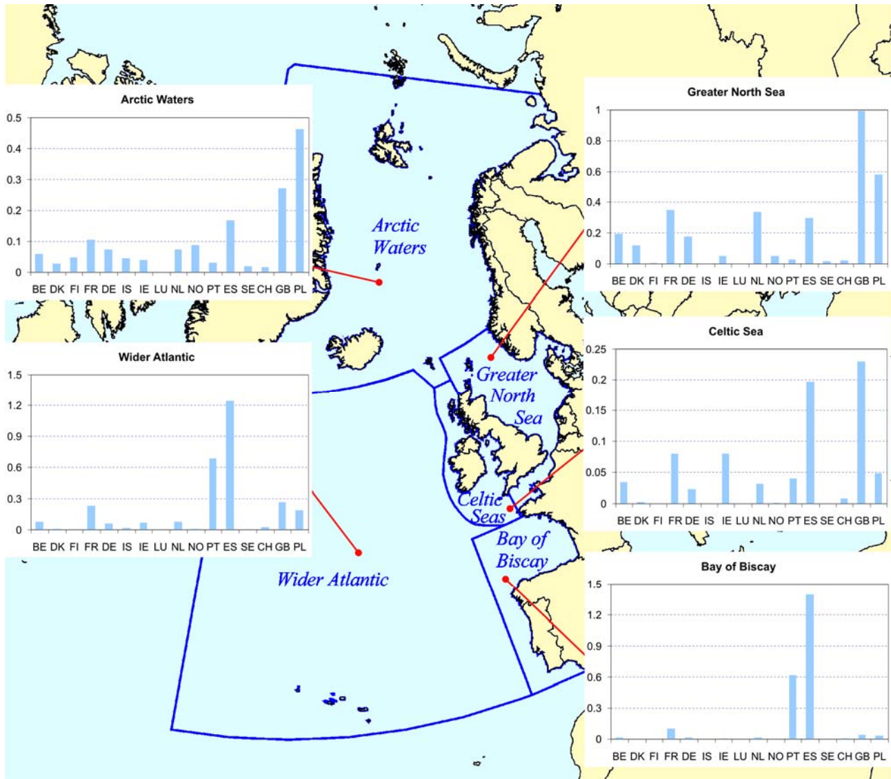
Figure 6.19: Contribution of individual countries to the modelled annual depositions of cadmium to the OSPAR Regions for 2006; units are in t/yr.
