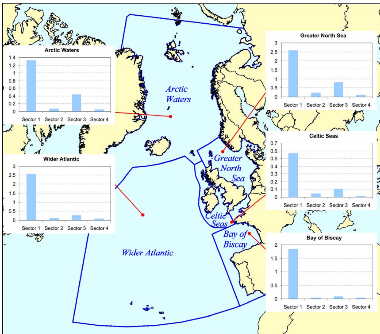
Figure 6.20: Contribution of four key source sectors to the cadmium deposition to the OSPAR Regions in 2005; units are in t/yr.
