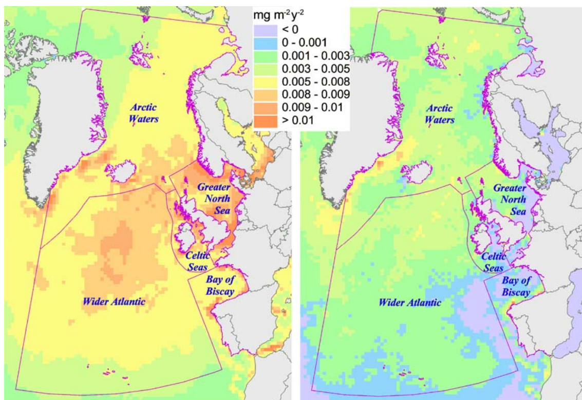
Figure 6.23: Total (left panel) and net (right panel) modelled deposition fluxes for mercury ( \text{mg}/\text{m}^2/\text{yr} ) to the OSPAR Regions in 2006; units are in \text{mg}/\text{m}^2 per year.
