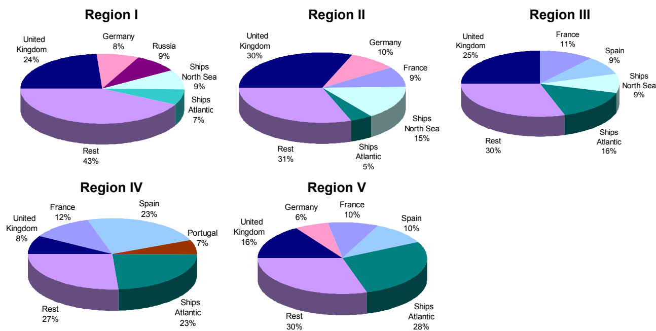
Figure 6.7: Contribution of major individual countries to the annual deposition of oxidized nitrogen to the OSPAR Regions in 2006. The contribution of international shipping on the North Sea and the Atlantic Ocean is presented as “Ships North Sea” and “Ships Atlantic” respectively.
