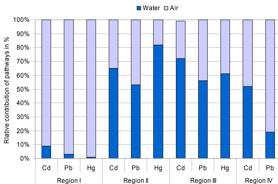
Figure 7.1: Total inputs of cadmium (Cd), lead (Pb) and mercury (Hg) to OSPAR Regions I – IV via direct discharges to water and riverine inputs (RID monitoring) and total atmospheric deposition (EMEP model calculations) averaged over the period 1990 - 2006. Waterborne inputs for Region IV are for 1997 – 2006 and inputs of mercury are insufficient to allow an assessment. Waterborne inputs for Region I are based on Norwegian data only.
