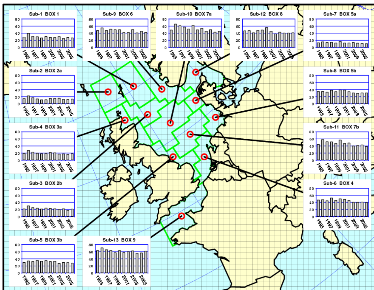
Figure 6.5: Map with time series of EMEP modelled total annual nitrogen (oxidized and reduced) deposition to the 13 sub-areas of Region II. Units in kt N/yr.
