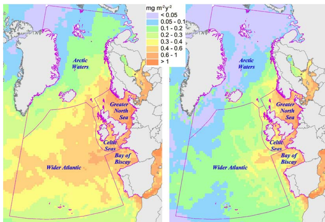
Figure 6.13: Map of modelled total deposition (left panel) and net deposition (right panel) of lead ( \text{mg}/\text{m}^2/\text{yr} ) to the OSPAR Regions in 2006; units are in \text{mg}/\text{m}^2 per year.
