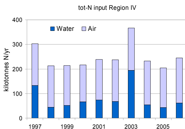
Figure A10.13: Total nitrogen inputs into Region IV by direct discharges and riverine inputs (RID) and the total EMEP modelled atmospheric deposition (Note: RID data for Spain and Portugal only).
