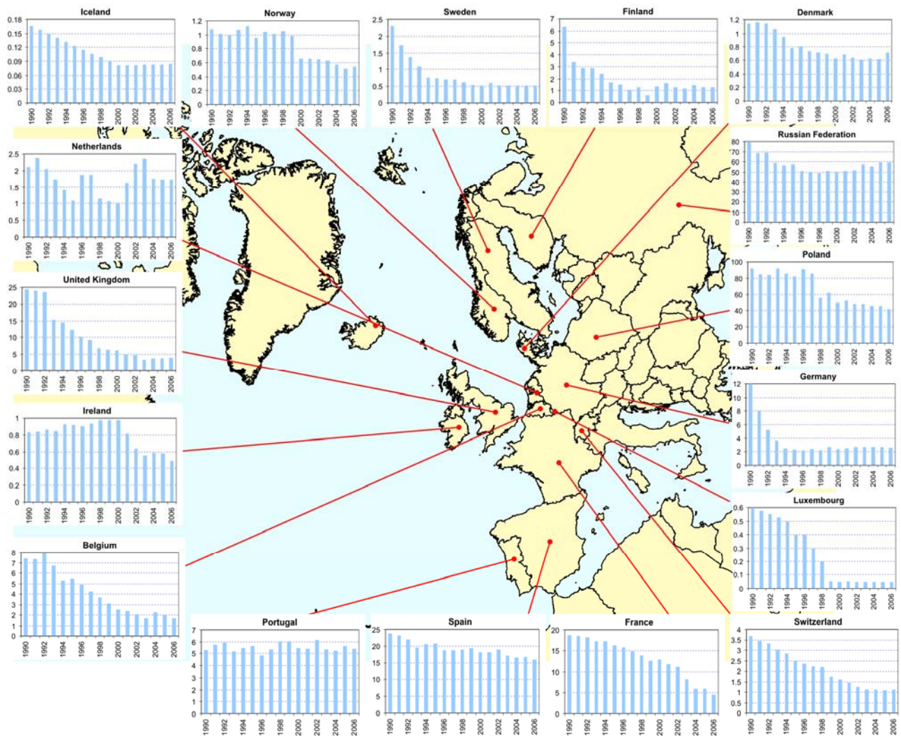
Figure A2.2: Atmospheric emission of cadmium in tonnes per year.
