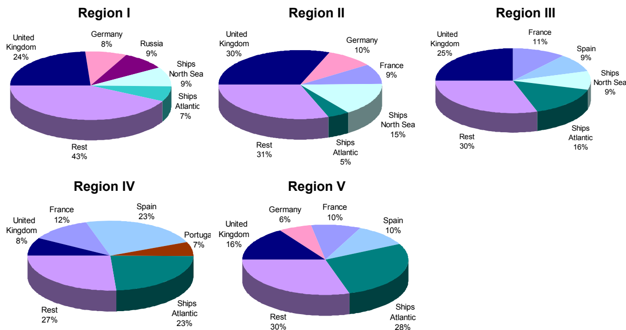
Figure 0.6: Main contributors to oxidized nitrogen deposition to the OSPAR Regions in 2006. Contribution of international shipping on the North Sea and the Atlantic is presented as “Ships North Sea” and “Ships Atlantic”, respectively.
