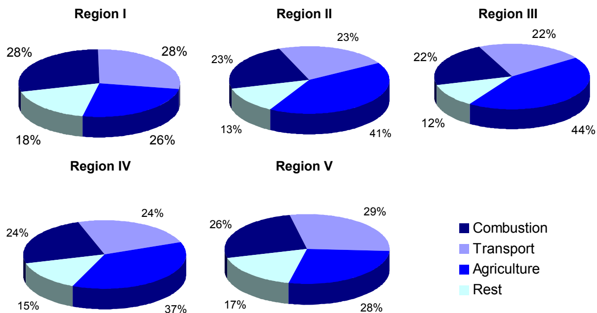
Figure 6.3: Contribution of sectors (as defined by the EMEP Selected Nomenclature for reporting of Air Pollutants (SNAP)) to the total annual nitrogen (oxidized and reduced) deposition to the OSPAR Regions in 2006. Combustion includes SNAP 1 (combustion in energy and transformation industry), SNAP 2 (non-industrial combustion plants) and SNAP 3 (combustion in manufacturing industry). Transport includes SNAR 7 (road transport) and SNAP 8 (other mobile sources and machinery, including international shipping). SNAP 10 is the basis for agricultural data.
