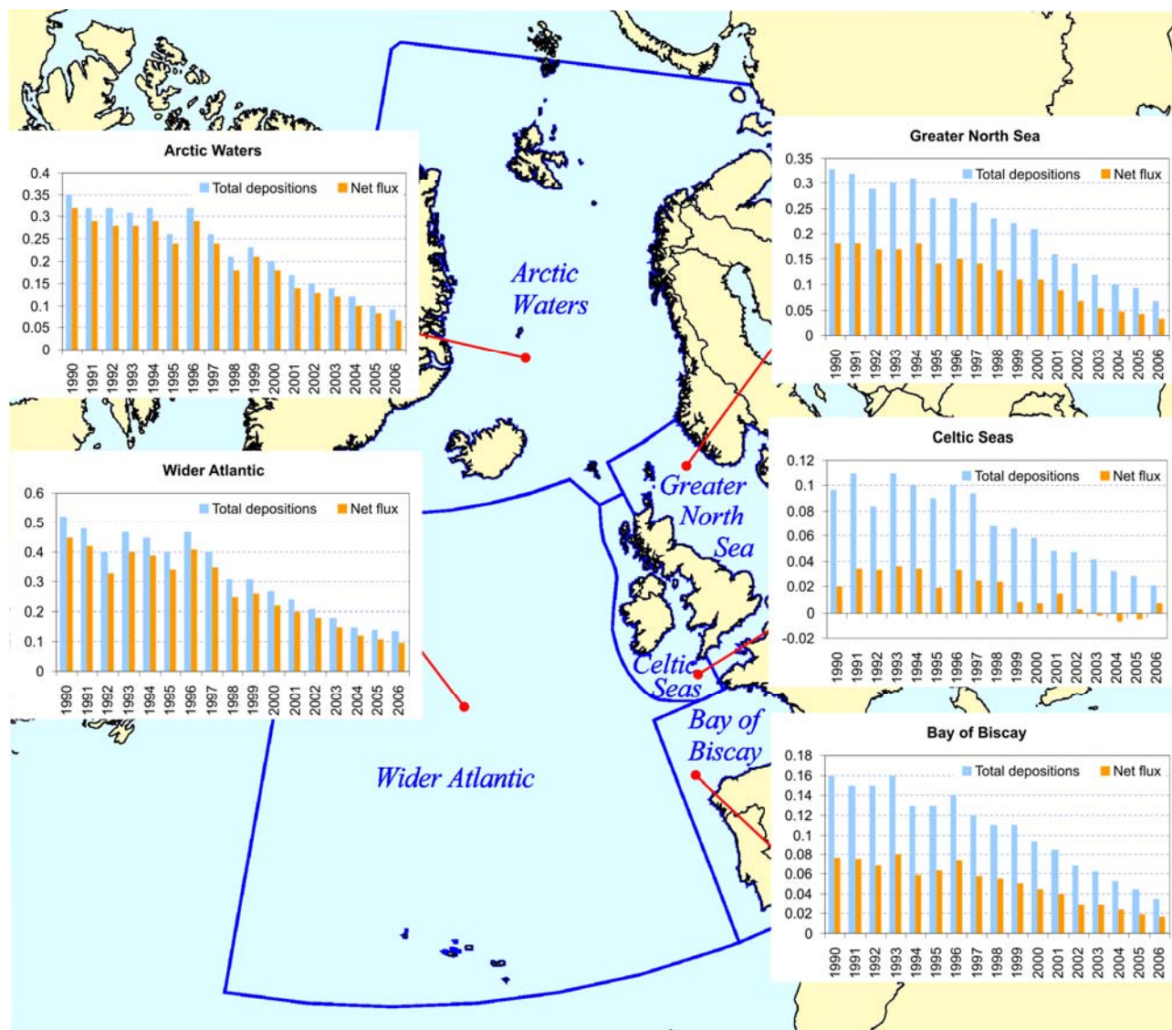
Figure 6.33: Time series (1990 – 2006) of modelled total and net deposition fluxes of PCB-153 to the OSPAR Regions; units are in t/yr.
