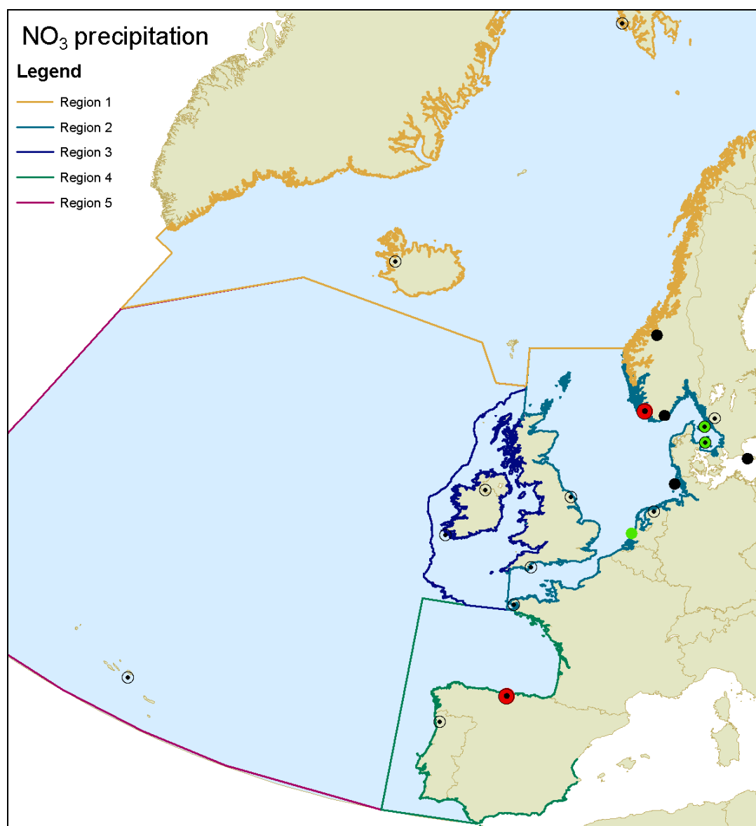
Figure 4.2: Geographical distribution of results from the trend analysis for nitrate in precipitation. For explanation see Figure 4.1. In this graph only small and medium size dots are depicted.
