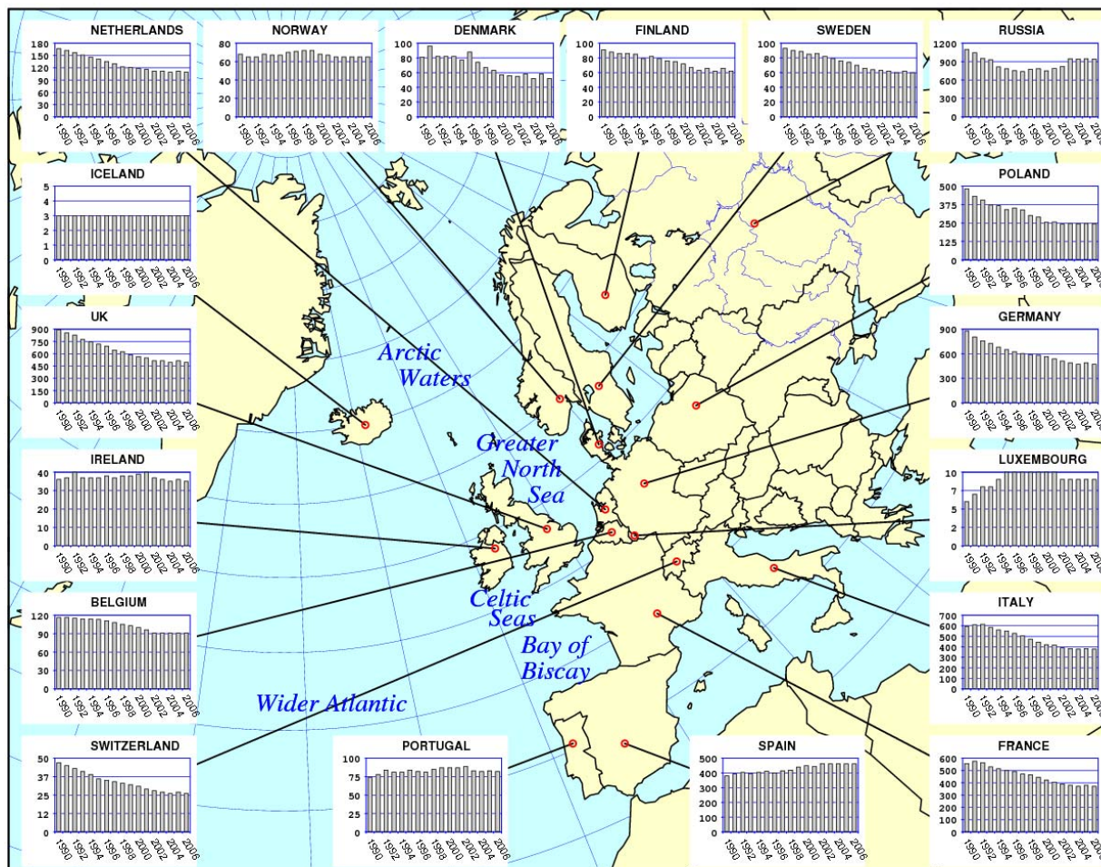
Figure A1.1: Annual nitrogen oxides (NO x ) emissions from the OSPAR Contracting Parties, Russia, Poland and Italy. Units are in kt N/yr.
