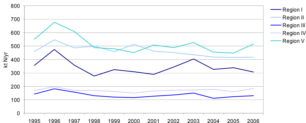
Figure 0.4: Time series of total nitrogen deposition to the OSPAR Regions for the period 1995 – 2006 (unit: kt N/yr).
