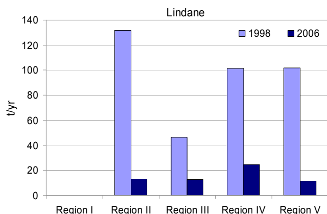
Figure 3.4: Comparison of the total atmospheric emissions of lindane to the different OSPAR Regions for the years 1998 and 2006.
