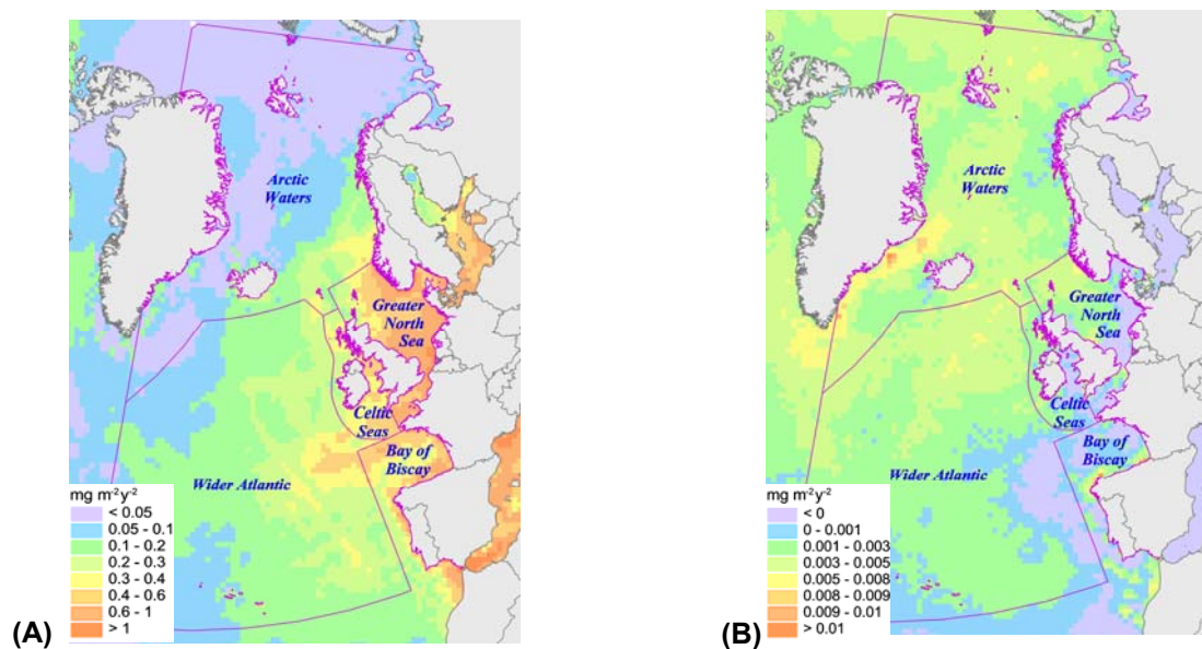
Figure 0.2: Spatial distribution of the annual net deposition in 2006 of lead (A) and mercury (B) to the OSPAR area and its Regions. Unit is in \text{mg/m}^2/\text{yr} .
