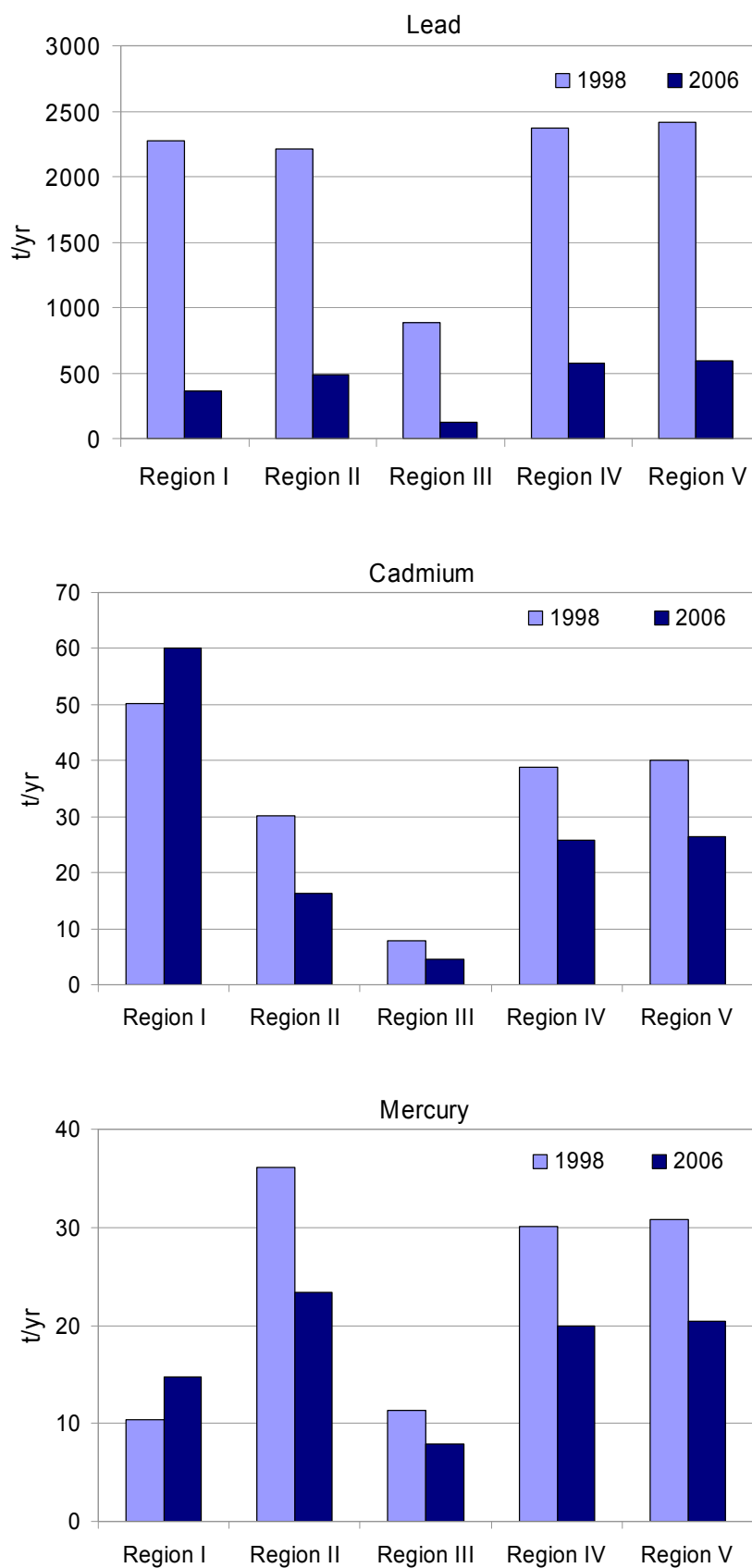
Figure 3.3: Comparison of the total atmospheric emissions of lead, cadmium and mercury to the five OSPAR Regions for the years 1998 and 2006.
