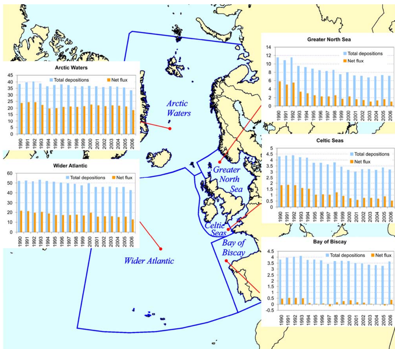
Figure 6.26: Time series of modelled total and net deposition fluxes of mercury to the OSPAR Regions (1990 – 2006); units are in t/yr.
