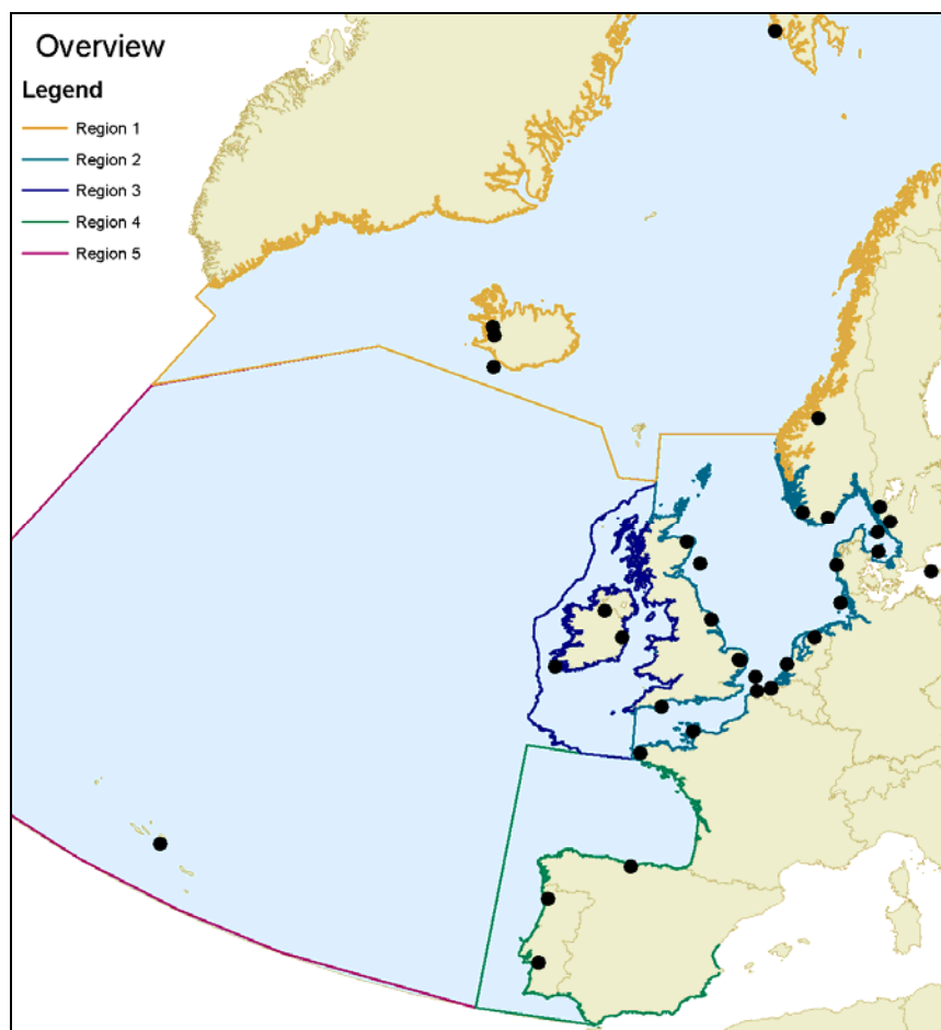
Figure 2.2: Geographical position of the CAMP monitoring stations used in this report.
