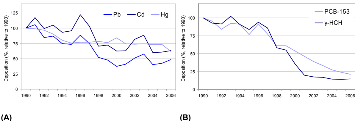
Figure 0.1: Percentage change in modelled total deposition of the metals lead, cadmium and mercury (A) and of the organic contaminants PCB-153 and lindane ( \gamma -HCH) (B) to the OSPAR area in 1990 - 2006.
