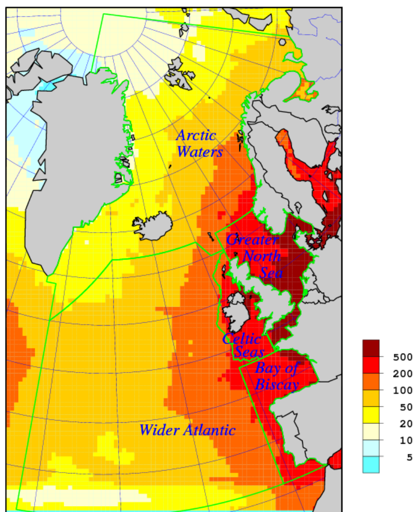
Figure 6.1: Map of EMEP modelled total annual nitrogen (oxidized and reduced) deposition to the five OSPAR Regions in 2006. Units are in mg N/m 2 per year.
