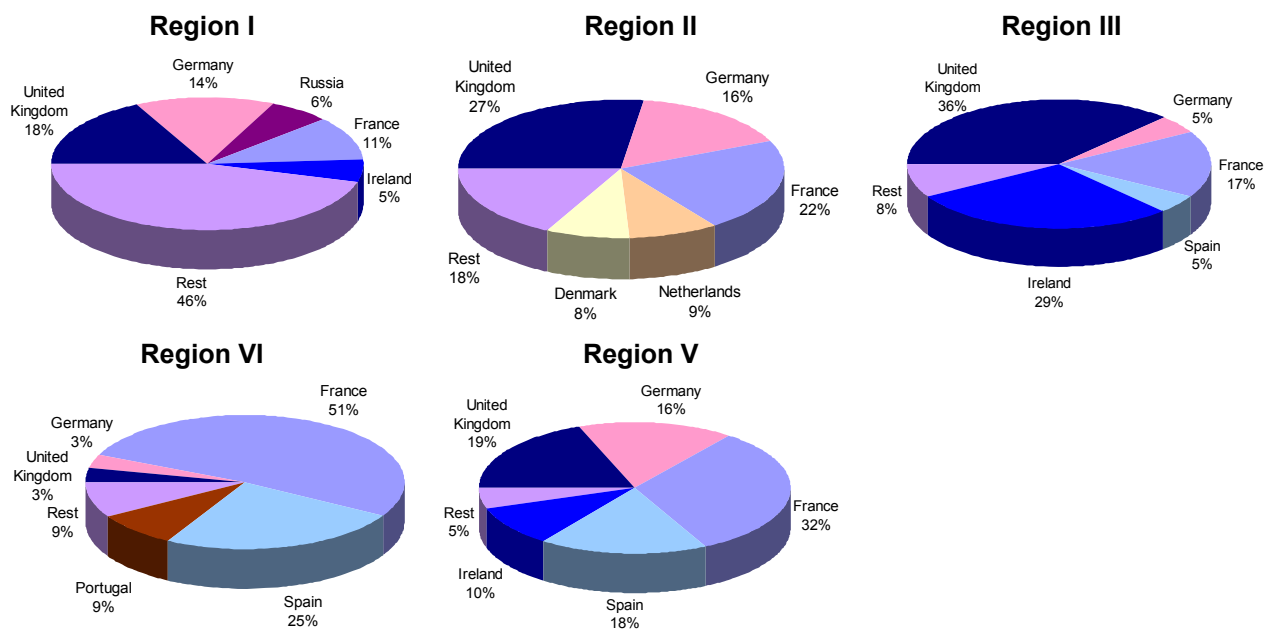
Figure 6.10: Contribution of major individual countries to the annual deposition of reduced nitrogen to the OSPAR Regions in 2006.
