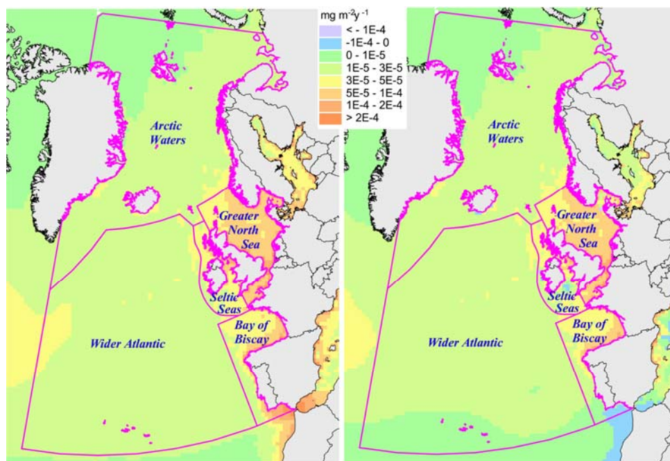
Figure 6.31: Total (left panel) and net (right panel) modelled deposition fluxes of PCB-153 to the OSPAR Regions in 2006; units are in \text{mg/m}^2 per year.
