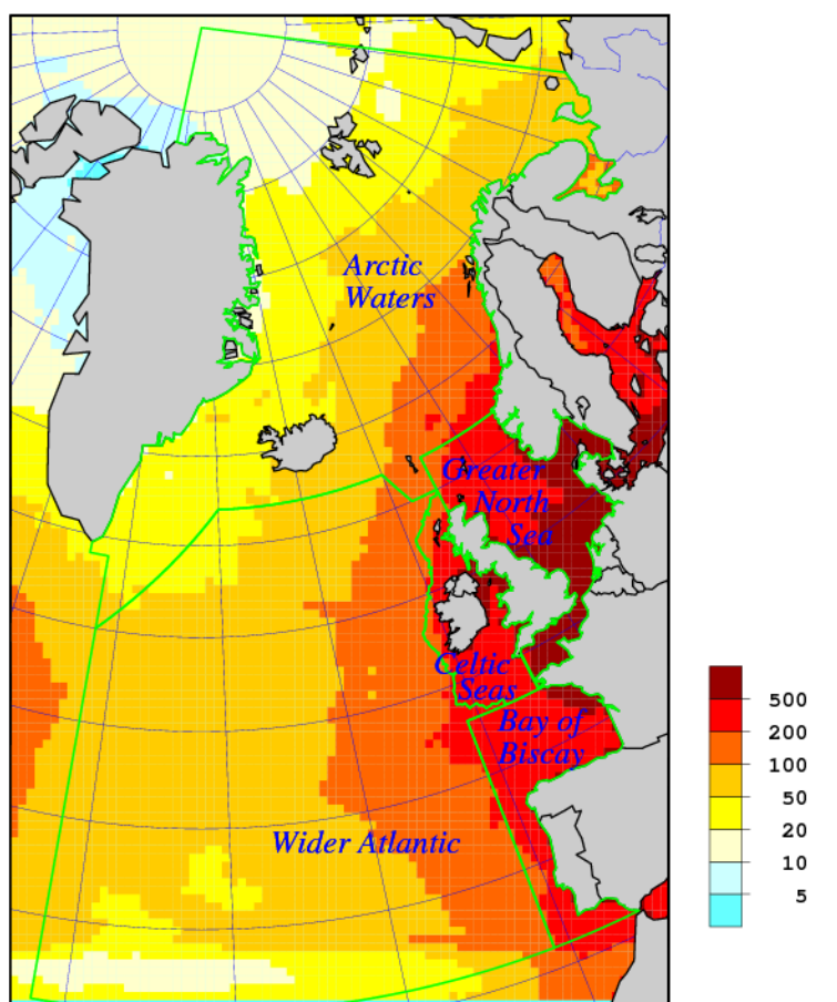
Figure 0.5: Modelled spatial distribution of total nitrogen deposition to the OSPAR area and its Regions in 2006 (unit: t N/yr/grid).
