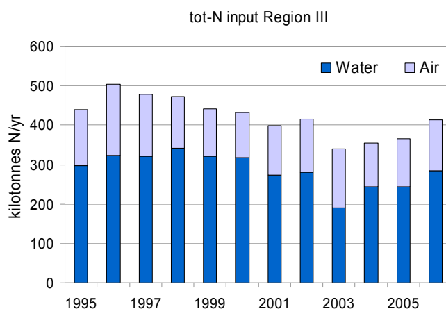
Figure A10.9: Total nitrogen inputs to Region III by direct discharges and riverine inputs (RID) and the total EMEP modelled atmospheric deposition.
