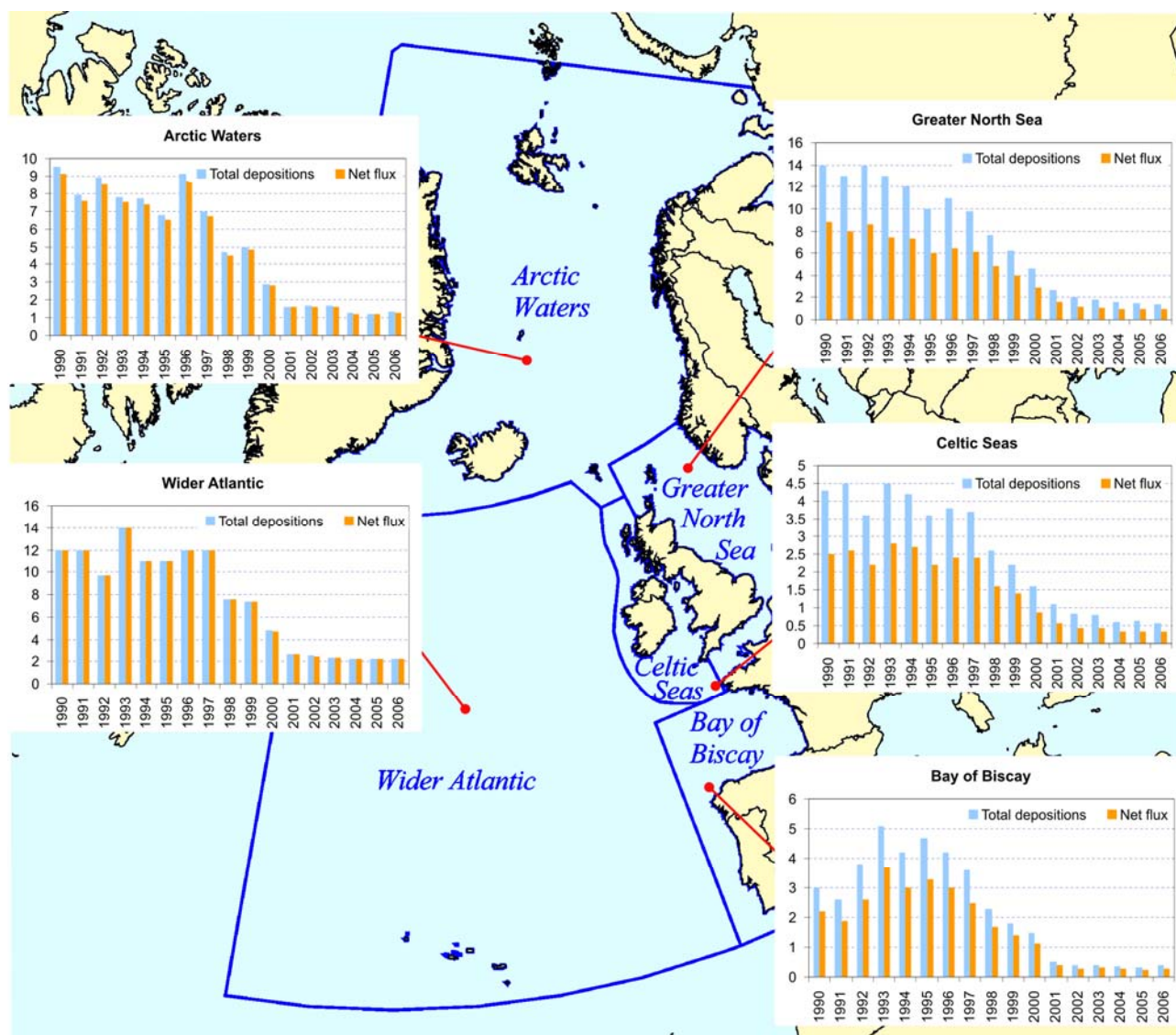
Figure 6.30: Time series (1990 – 2006) of modelled total and net deposition fluxes of lindane to the OSPAR Regions; units are in t/yr.
