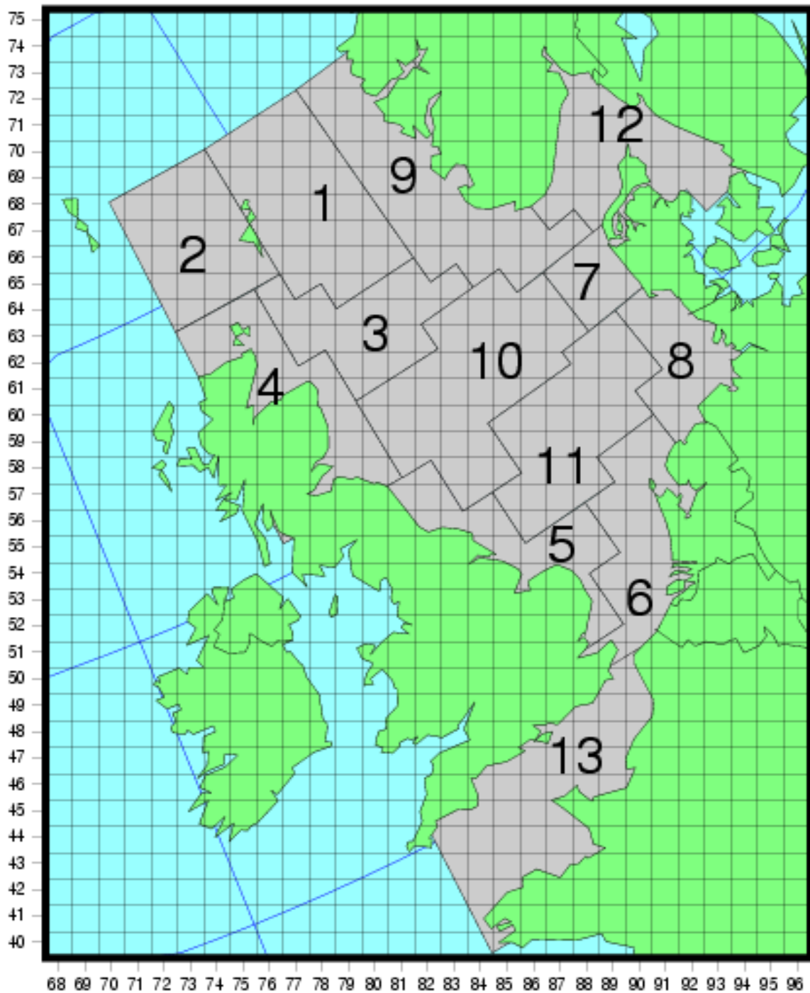
Figure 3. Location of the 13 sub-regions of OSPAR Region II (Greater North Sea) in the EMEP model grid system.
