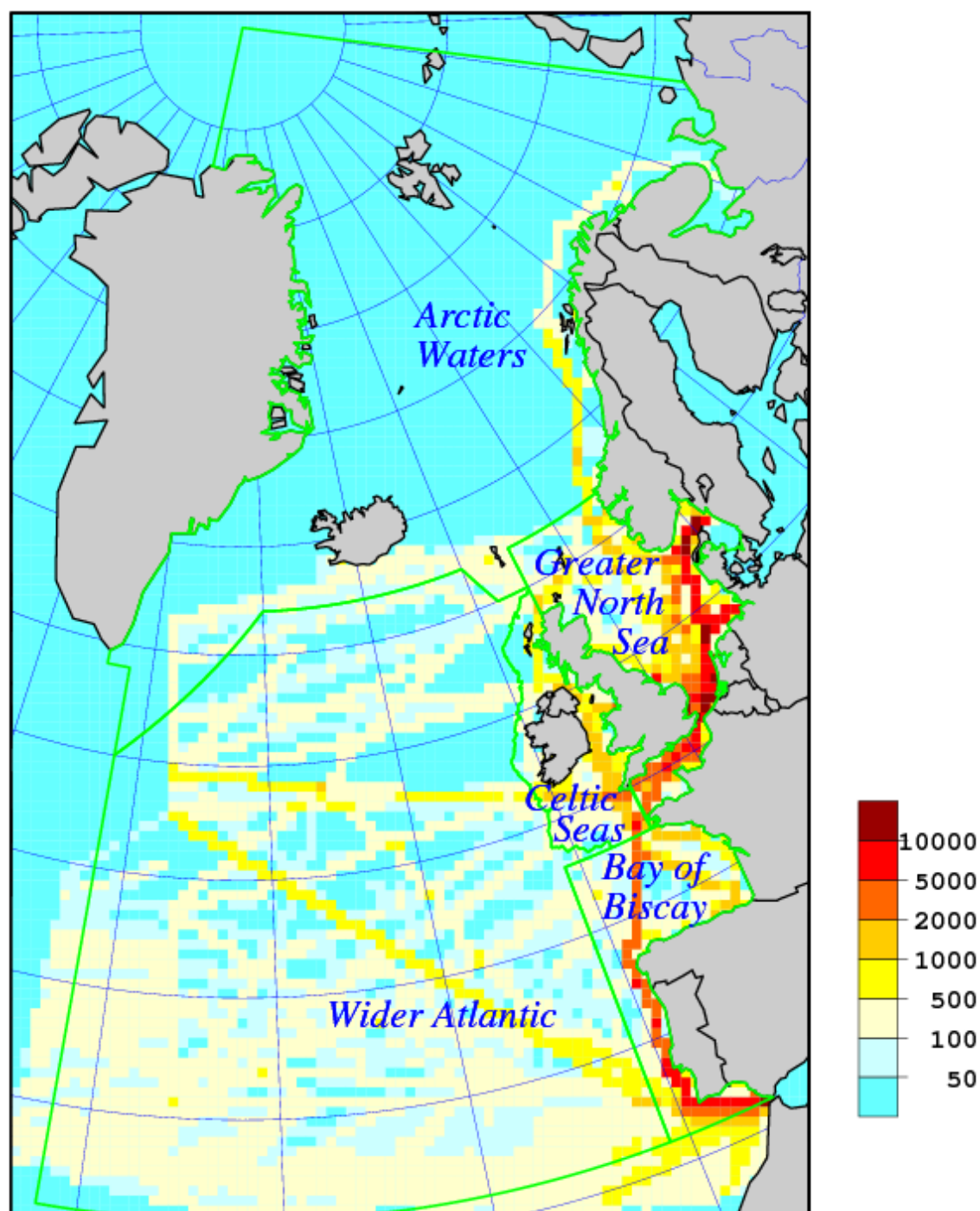
Figure 4. A map of 2004 nitrogen oxides emissions from the international ship traffic over the North Sea and Atlantic Ocean used in the model calculations for 2004. Units: t\ N\ a^{-1} ( 50 \times 50\ km^2 model grid square) 1 .
