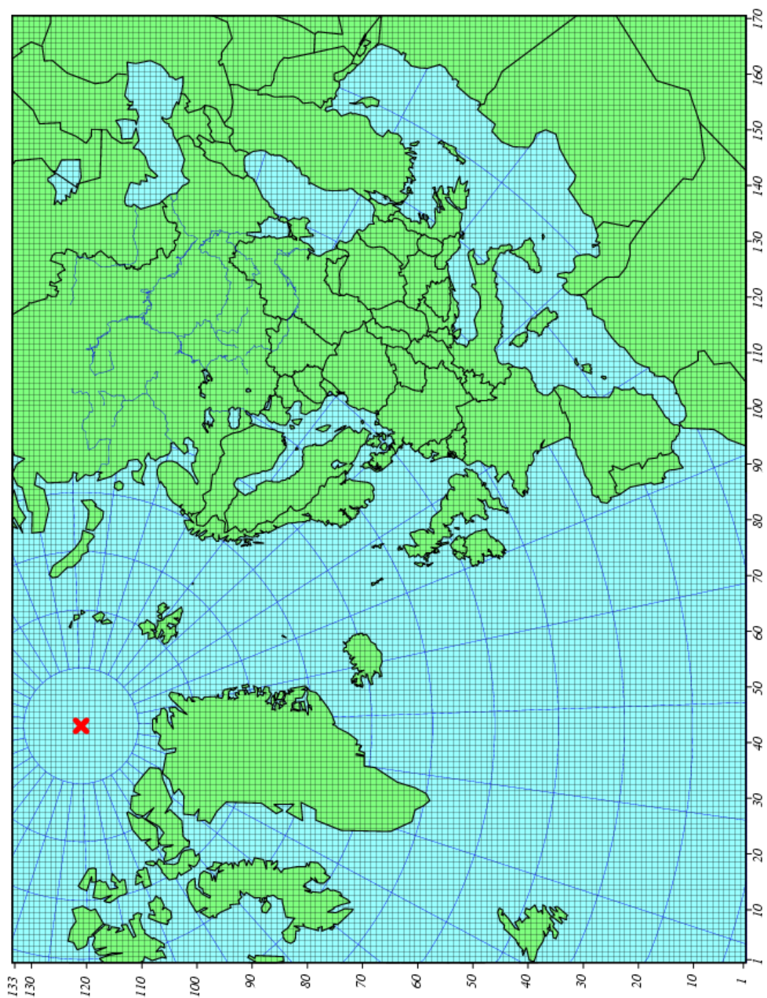
Figure 1. The EMEP model grid system of the size 170 \times 133 in the Polar Stereographic projection. The grid resolution is 50 km at 60^\circ N.
