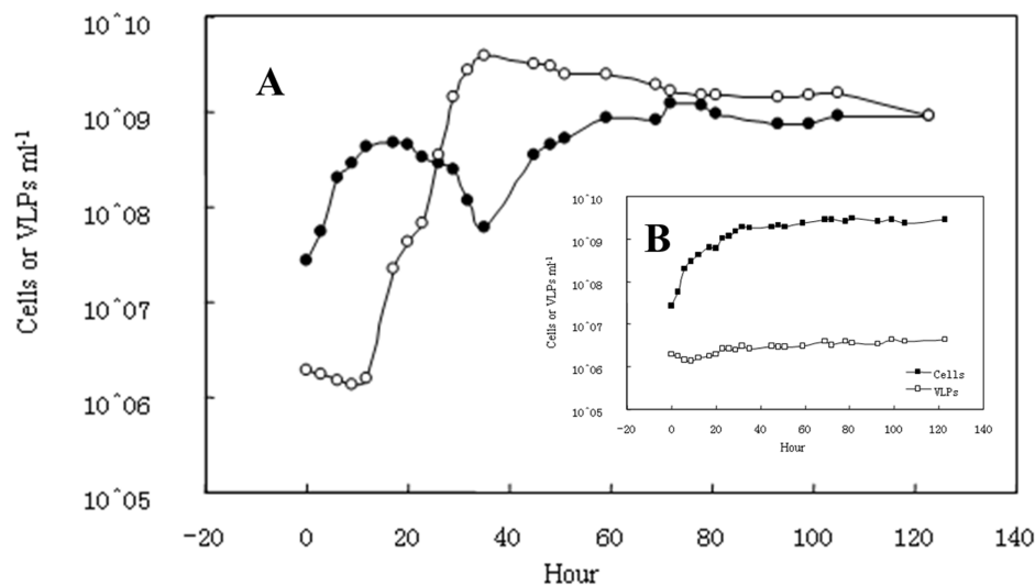
Figure 1 | Viral particle yield following mitomycin C induction of C. bathyomarinum JL354. Flow cytometry counts of JL354 cells and viral-like particles were performed with (A) a mitomycin C-treated culture and (B) a control culture without mitomycin C.
