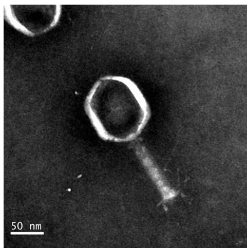
Figure 2 | Virus generated by mitomycin C induction of C. bathyomarinum JL354. Scale bars, 50 nm.
