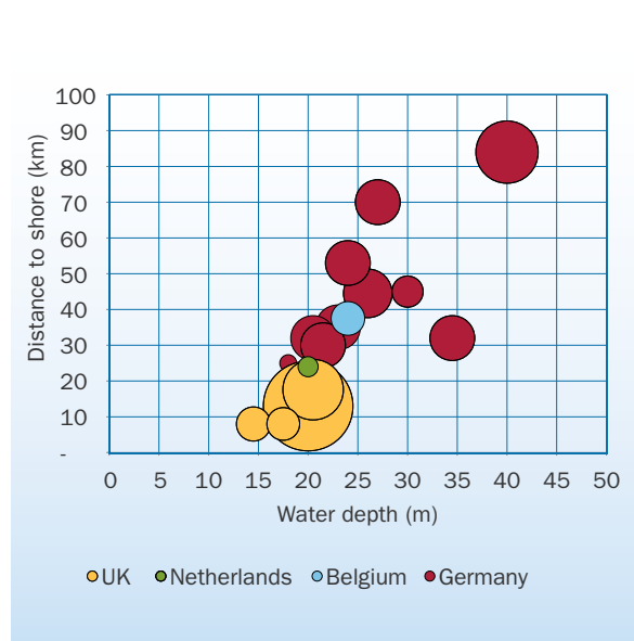
FIG 10: WATER DEPTH, DISTANCE TO SHORE AND SIZE OF OFFSHORE WIND FARMS UNDER CONSTRUCTION DURING 2014
