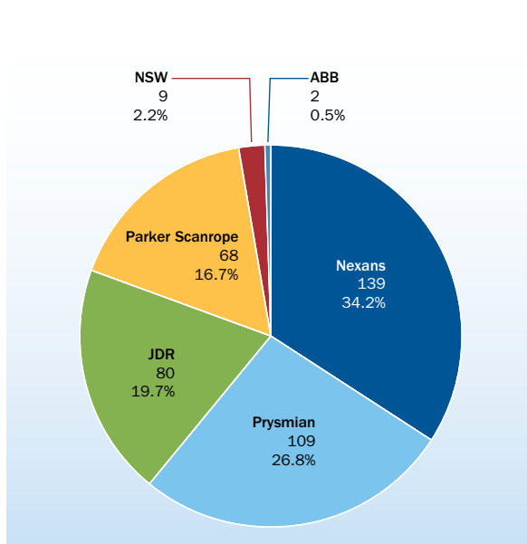
FIG 8: SHARE OF INTER-ARRAY CABLE SUPPLIERS TO OFFSHORE WIND FARMS IN 2014 (NO. OF CABLES) 4
