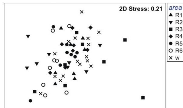
Figure 3. MDS plot of species abundance ( \text{m}^{-2} ) data (Bray–Curtis index, fourth root-transformed) of boxcore samples in OWEZ wind farm (W) and the six reference areas in 2011.
