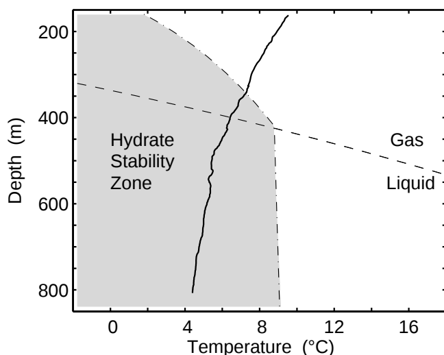
Figure 1: The phased diagram for CO 2 in sea water showing the hydrate phase boubary. A temperature profile for the ocean off northern California is overlaid.
